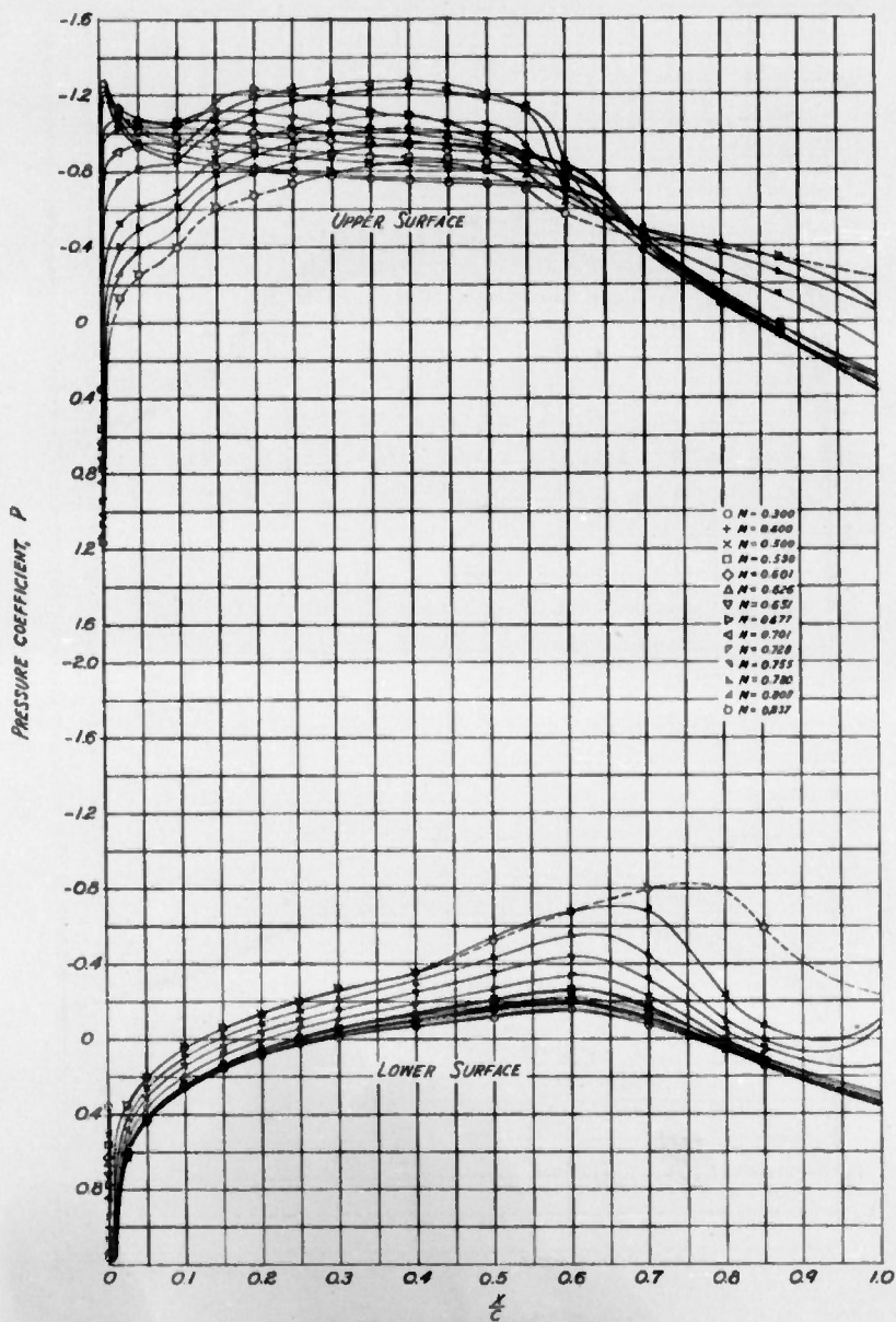
(1) SECTION ANGLE OF ATTACK, \alpha_0 = 4^\circ FIGURE 3.- CONTINUED. NACA 66.2-215 ( q = 0.6 ) AIRFOIL SECTION
