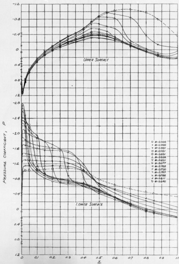
(a) SECTION ANGLE OF ATTACK, \alpha_s = -6^\circ FIGURE 2.- PRESSURE DISTRIBUTION OVER THE NACA 65-215 ( a=0.5 ) AIRFOIL SECTION WITH CONSTANT ANGLE OF ATTACK AND VARYING MACH NUMBER.
