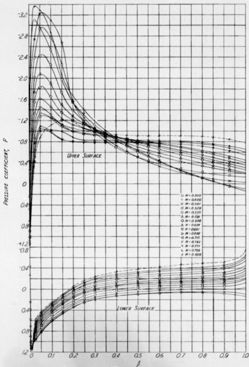
FIGURE 5.- CONTINUED NACA 23015 AIRFOIL SECTION
