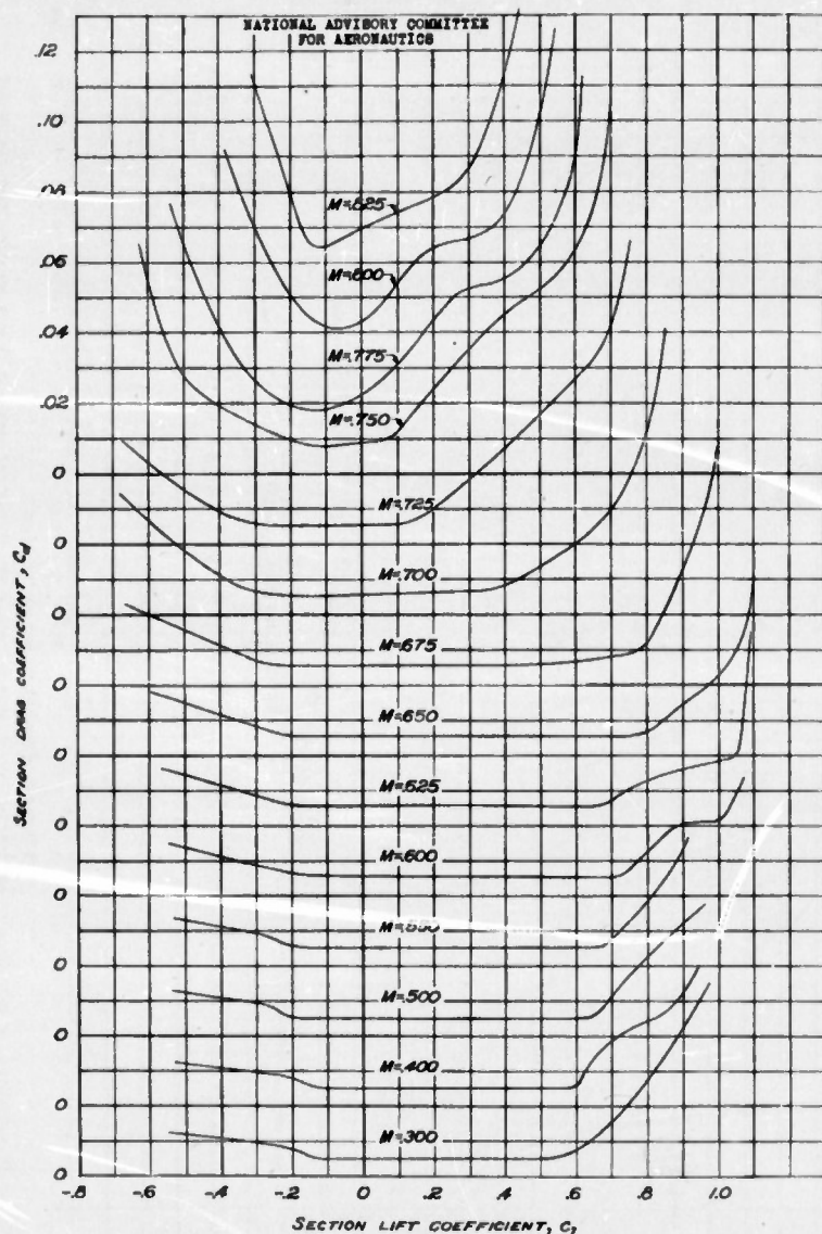
FIGURE 30.—VARIATION OF SECTION DRAG COEFFICIENT WITH LIFT COEFFICIENT FOR THE NACA 65-215 ( q=0.5 ) AIRFOIL.
