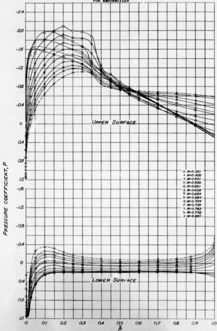
FIGURE 6.-CONTINUED. NACA 4415 AIRFOIL SECTION
