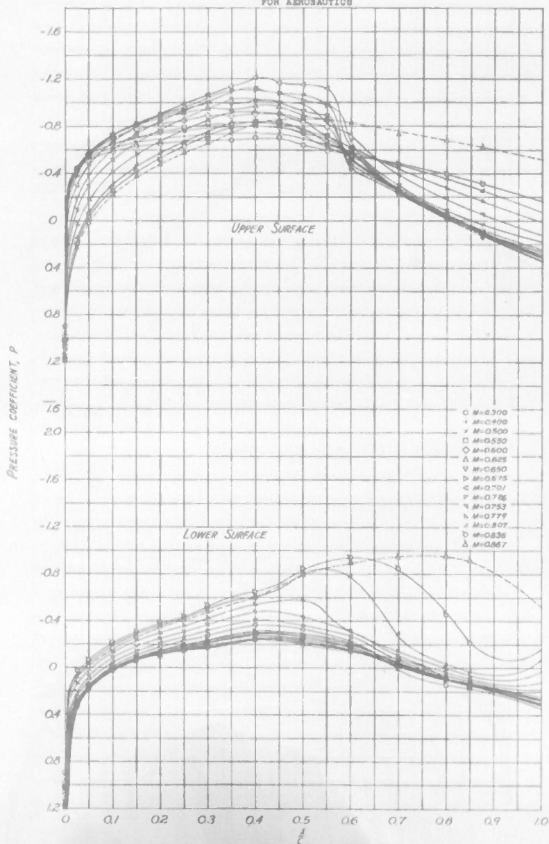
(a) SECTION ANGLE OF ATTACK, \alpha = 2^\circ FIGURE 2- CONTINUED NACA 65-215 ( a=0.5 ) AIRFOIL SECTION
