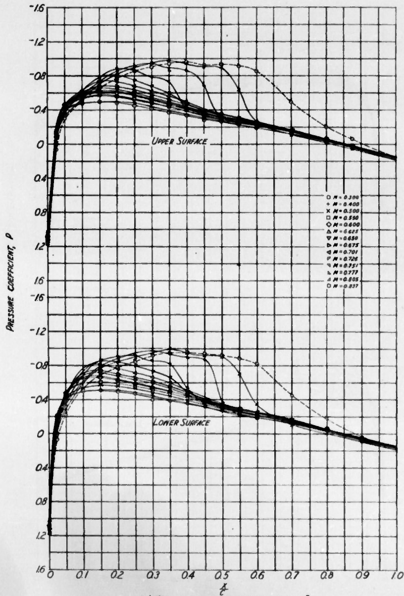
(2) SECTION ANGLE OF ATTACK, \alpha_0 = 0^\circ FIGURE 4.- PRESSURE DISTRIBUTION OVER THE NACA 0015 AIRFOIL SECTION WITH CONSTANT ANGLE OF ATTACK AND VARYING MACH NUMBER CONFIDENTIAL
