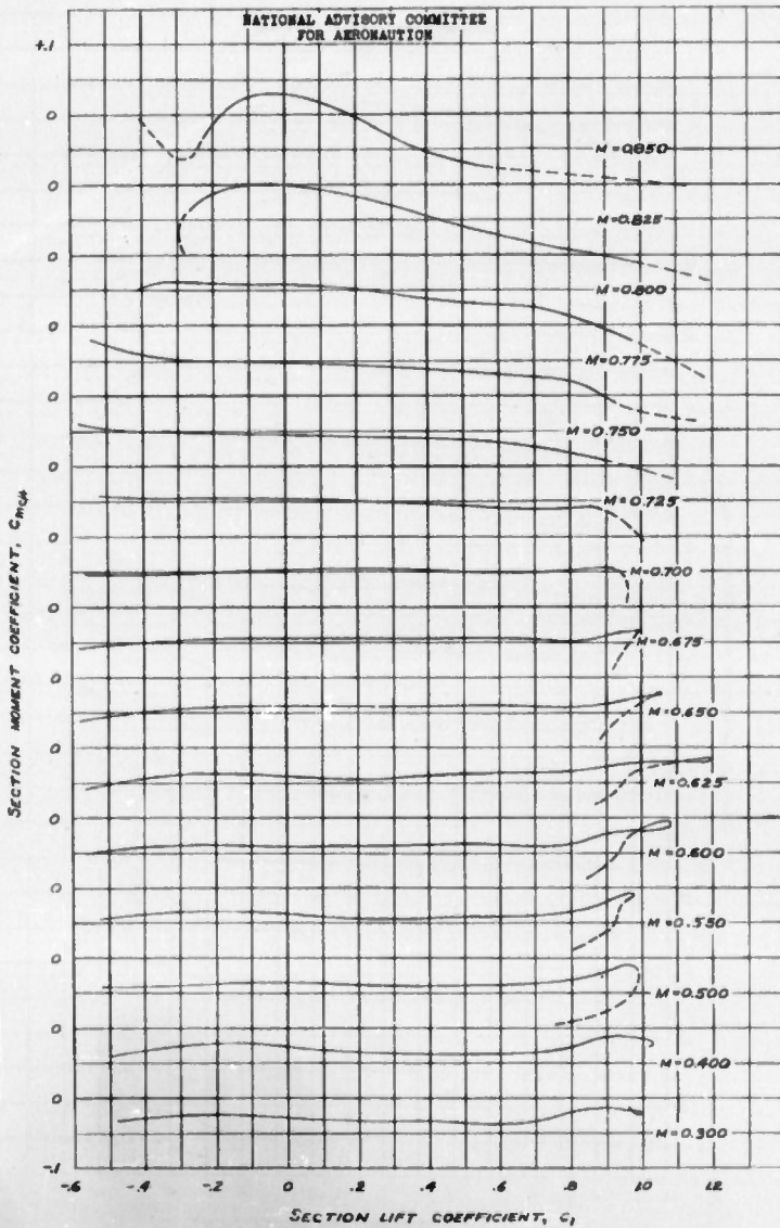
FIGURE 35.— VARIATION OF SECTION QUARTER-CHORD MOMENT COEFFICIENT WITH LIFT COEFFICIENT FOR THE NACA 63-215 ( \alpha=0.5 ) AIRFOIL.
