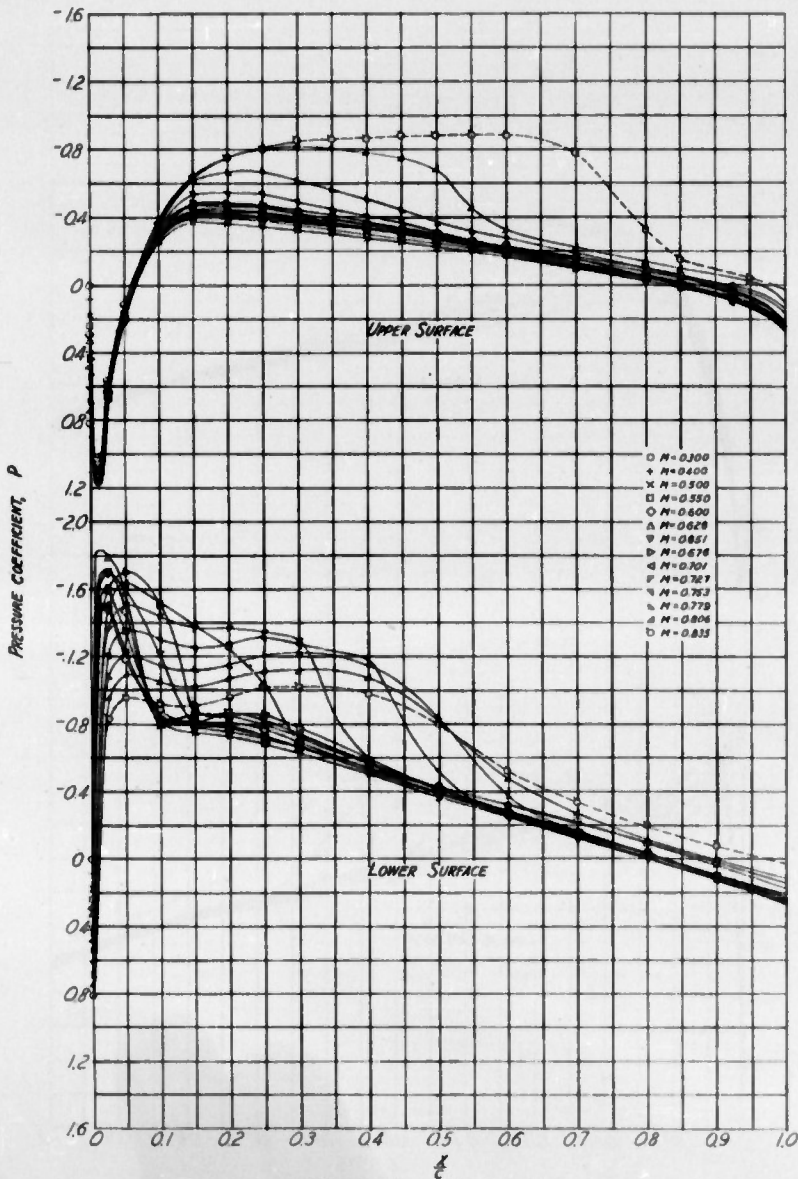
(A) SECTION ANGLE OF ATTACK, \alpha_s = -4^\circ FIGURE 5.- CONTINUED NACA 23015 AIRFOIL SECTION
