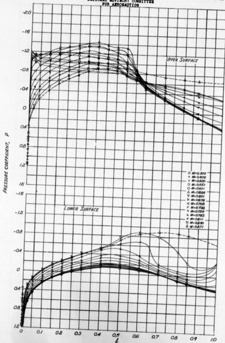
(K) SECTION ANGLE OF ATTACK, \alpha = 4^\circ FIGURE 2-CONTINUED. NACA 63-215 ( a=0.5 ) AIRFOIL SECTION
