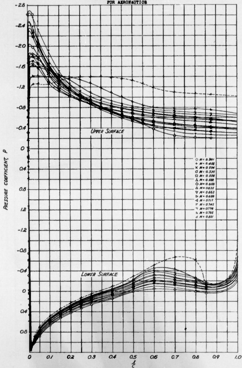
(j) SECTION ANGLE OF ATTACK, \alpha_0 = 12^\circ FIGURE 3- CONTINUED. NACA 66,2-215 \frac{1}{2} -0.6 AIRFOIL SECTION
