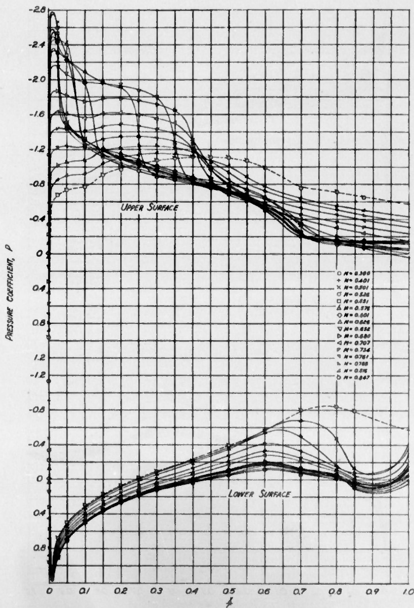
(N) SECTION ANGLE OF ATTACK, \alpha_s = 8^\circ FIGURE 3.- CONTINUED. NACA 66,2-213 ( a=0.6 ) AIRFOIL SECTION
