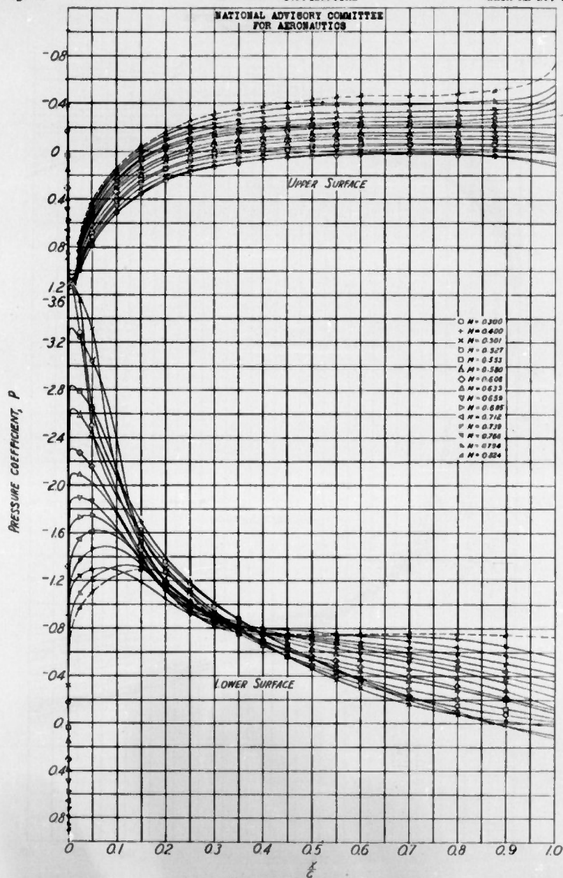
(A) SECTION ANGLE OF ATTACK, \alpha_s = -10^\circ FIGURE 4.- CONTINUED NACA 0015 AIRFOIL SECTION
