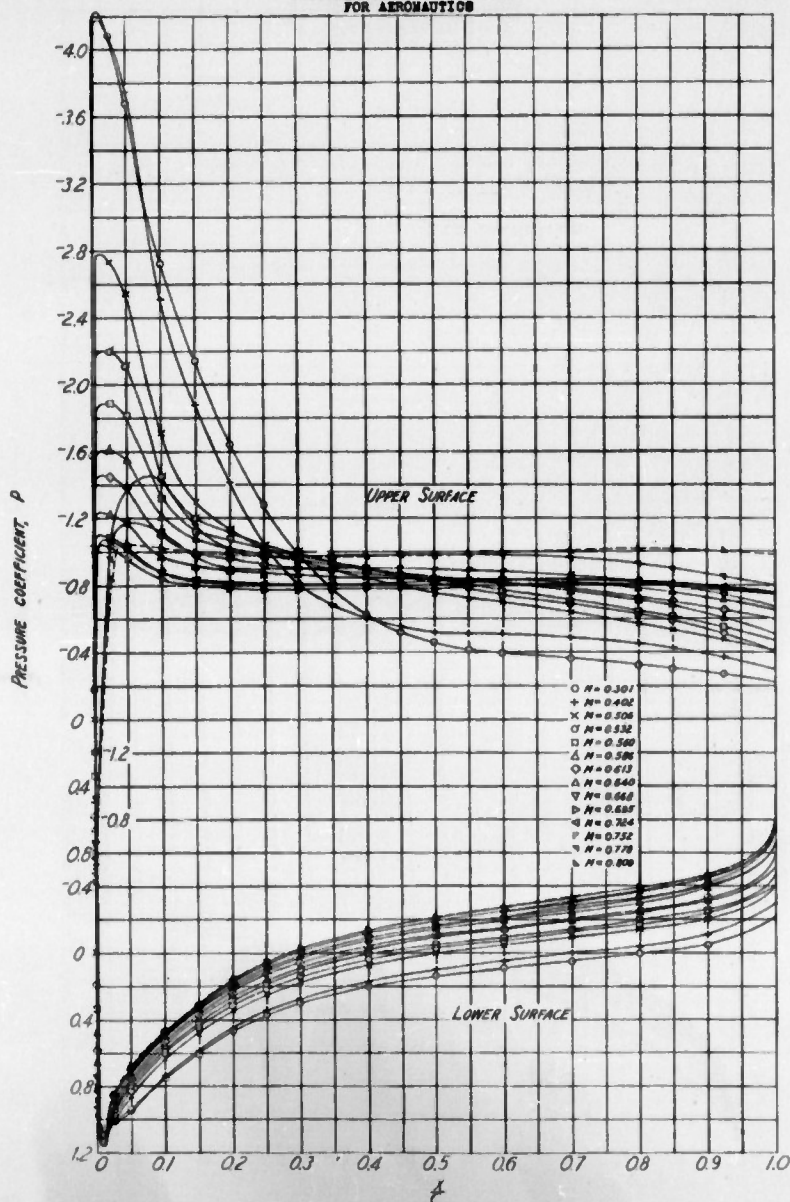
FIGURE 5.- CONTINUED. NACA 23015 AIRFOIL SECTION
