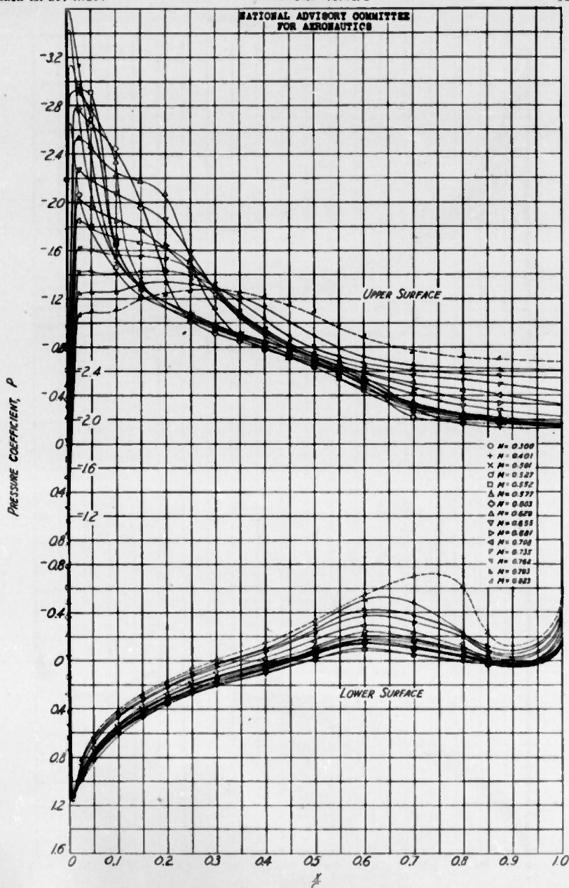
(1) SECTION ANGLE OF ATTACK, \alpha_s = 10^\circ FIGURE 3- CONTINUED. NACA 66,2215(a-06) AIRFOIL SECTION
