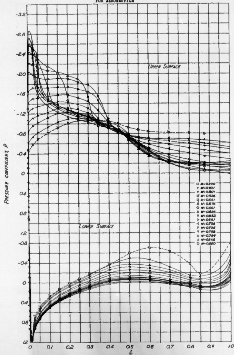
(h) SECTION ANGLE OF ATTACK, \alpha = 0^\circ FIGURE 2-CONTINUED. NACA 65-215 ( a=0.5 ) AIRFOIL SECTION
