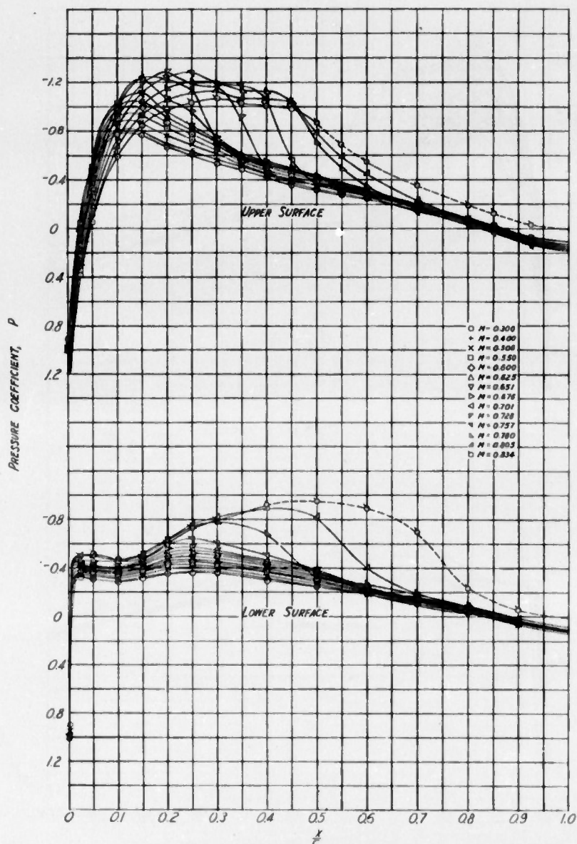
(d) SECTION ANGLE OF ATTACK, \alpha = 0^\circ FIGURE 5.- CONTINUED NACA 23015 AIRFOIL SECTION
