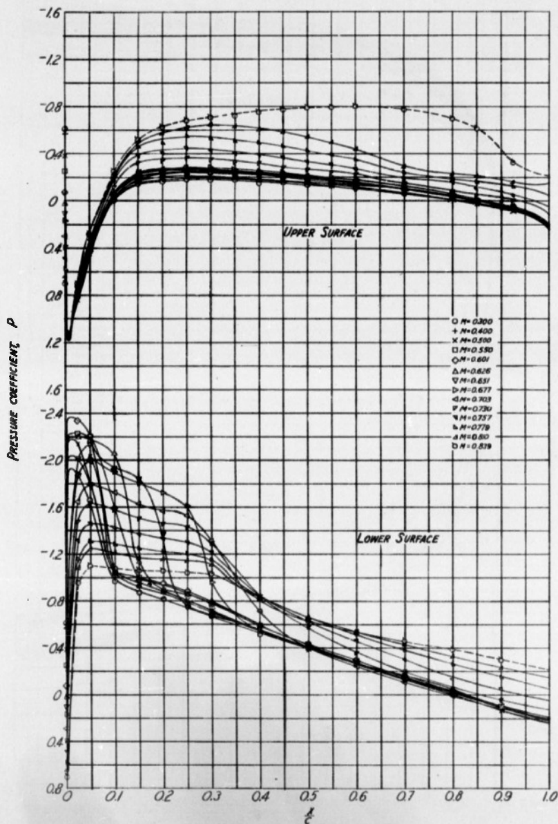
(a) SECTION ANGLE OF ATTACK, \alpha_s = 6^\circ FIGURE 5.- PRESSURE DISTRIBUTION OVER THE NACA 23015 AIRFOIL SECTION WITH CONSTANT ANGLE OF ATTACK AND VARYING MACH NUMBER CONFIDENTIAL
