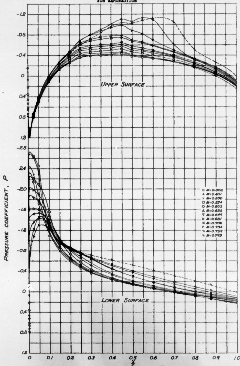
FIGURE 6-PRESSURE DISTRIBUTION OVER THE NACA 4415 AIRFOIL SECTION WITH CONSTANT ANGLE OF ATTACK AND VARYING MACH NUMBER
