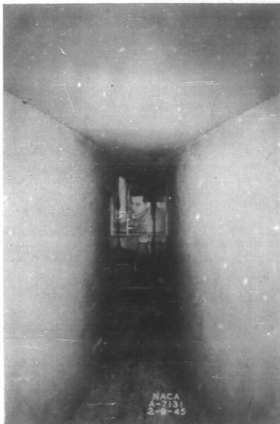
Figure 1.- Airfoil model mounted in the test section of the Ames 1 - by 3 1/2 foot high-speed wind tunnel.
