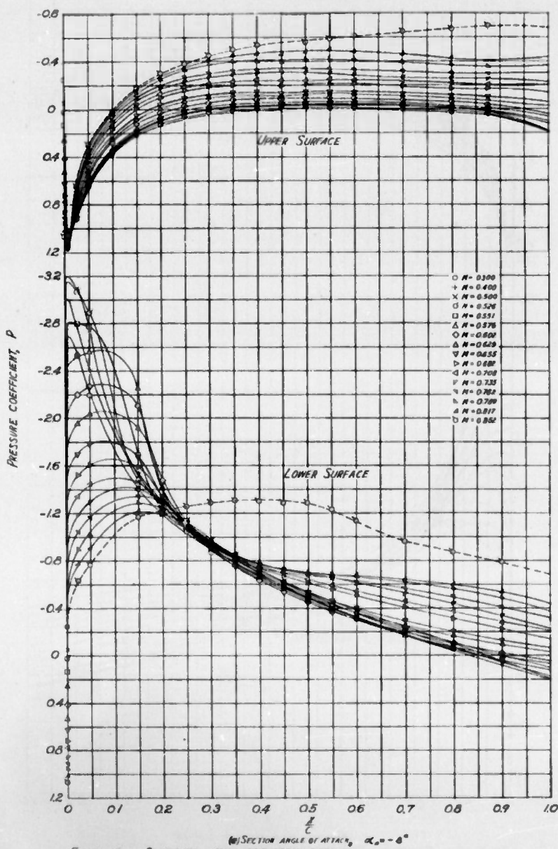
FIGURE 4c. CONTINUED NACA 0015 AIRFOIL SECTION
