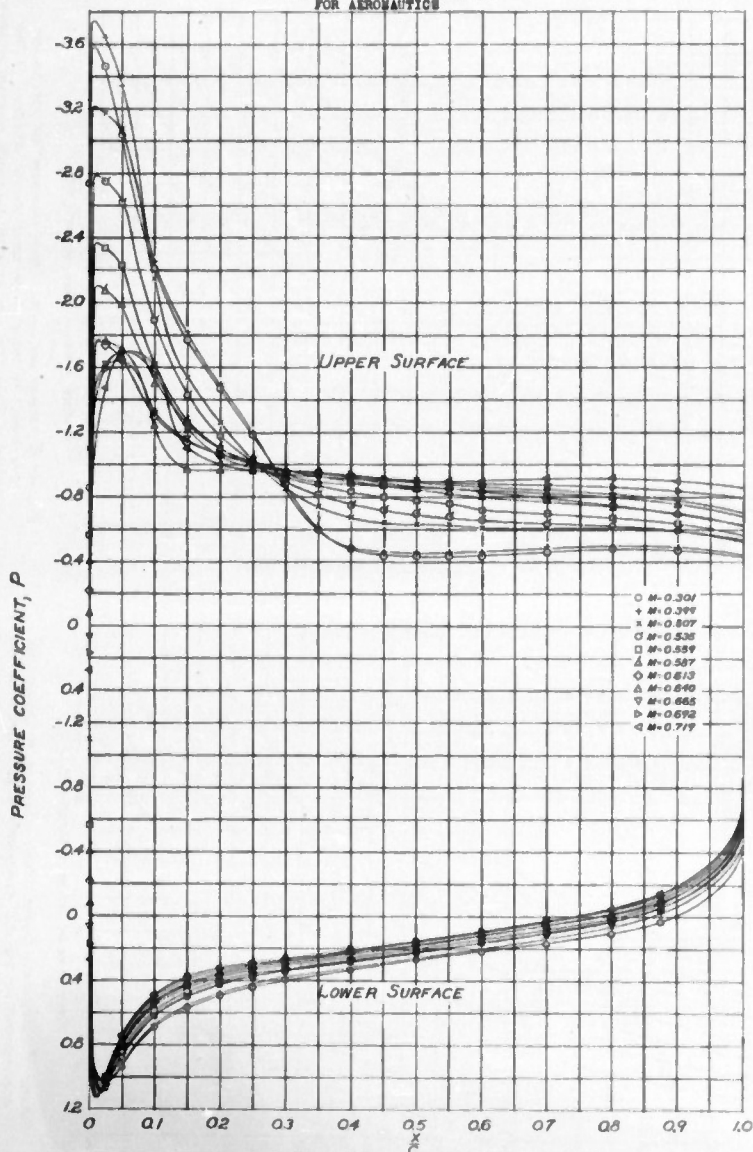
FIGURE 6: CONCLUDED. NACA 4415 AIRFOIL SECTION
