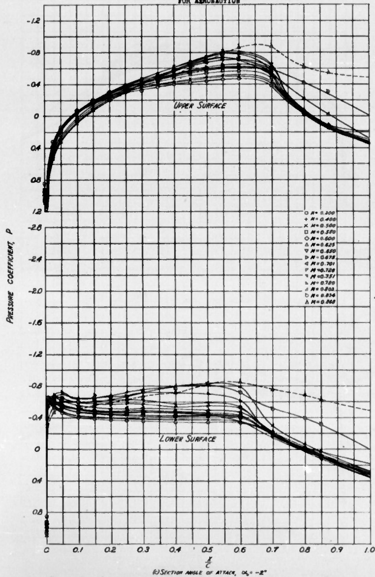
FIGURE 3.- CONTINUED. NACA 662-215 ( \mu = 0.6 ) AIRFOIL SECTION
