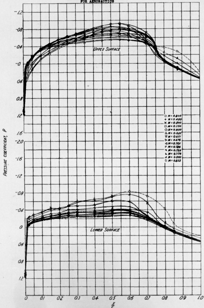
FIGURE 3.- CONTINUED. NACA 662-215 ( \theta = 0.6 ) AIRFOIL SECTION
