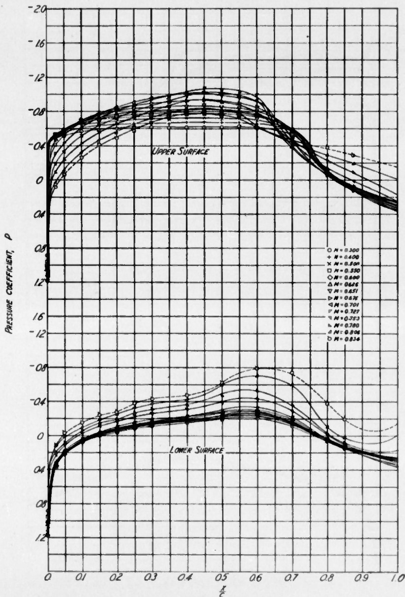
(H) SECTION ANGLE OF ATTACK, \alpha_0 = 2^\circ FIGURE 3.- CONTINUED. NACA 662-215(0.06) AIRFOIL SECTION
