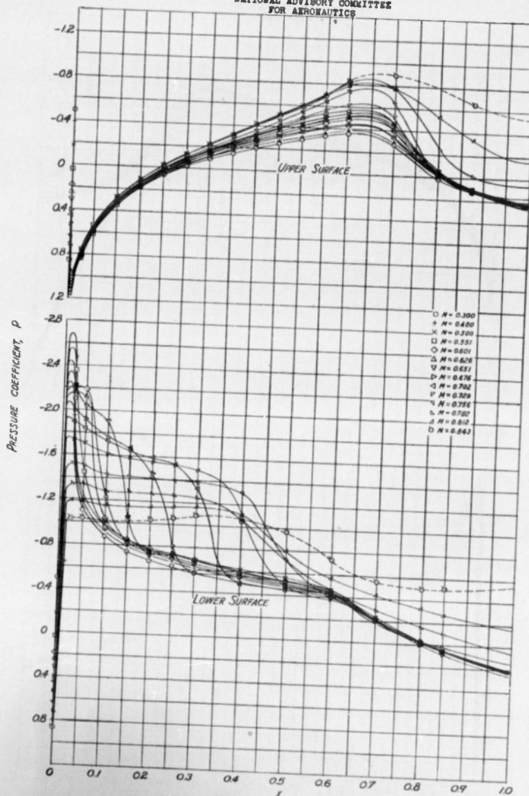
(a) SECTION ANGLE OF ATTACK, \alpha = 6^\circ FIGURE 3.- PRESSURE DISTRIBUTION OVER THE NACA 662-215 ( z = 0.6 ) AIRFOIL SECTION WITH CONSTANT ANGLE OF ATTACK AND VARYING MACH NUMBER
