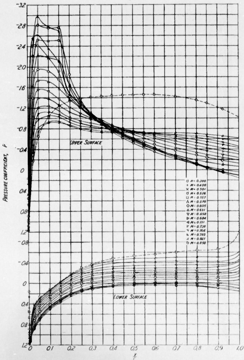
(a) SECTION ANGLE OF ATTACK, \alpha_0 = 0^\circ FIGURE 5- CONTINUED NACA 23015 AIRFOIL SECTION
