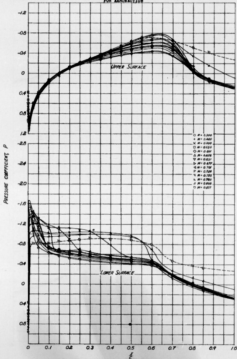
FIGURE 3- CONTINUED. (b) SECTION ANGLE OF ATTACK, \alpha = 4^\circ NACA 66,2-215 ( a = 0.8 ) AIRFOIL SECTION
