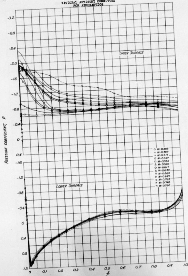
(2) SECTION ANGLE OF ATTACK, \alpha = 16^\circ FIGURE 2.—CONCLUDED NACA 65-215 ( \alpha = 0.5 ) AIRFOIL SECTION
