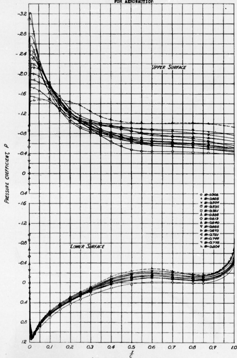
(A) SECTION ANGLE OF ATTACK, \alpha_s = 19^\circ FIGURE 2.- CONTINUED NACA 63-215 ( \theta=0.5 ) AIRFOIL SECTION
