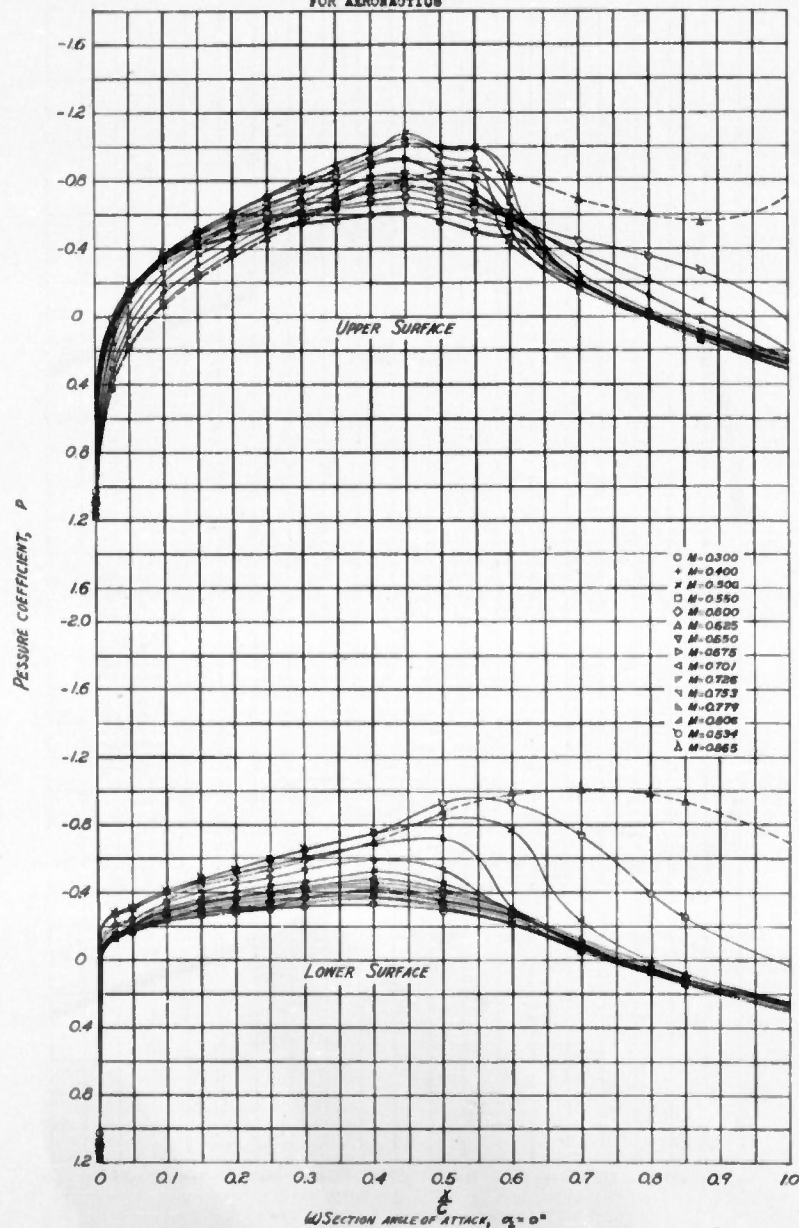
FIGURE 2-CONTINUED. NACA 63-215 ( \alpha = 0.5 ) AIRFOIL SECTION
