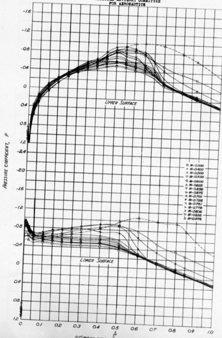
FIGURE 2-CONTINUED NACA 65-215 ( m=0.5 ) AIRFOIL SECTION
