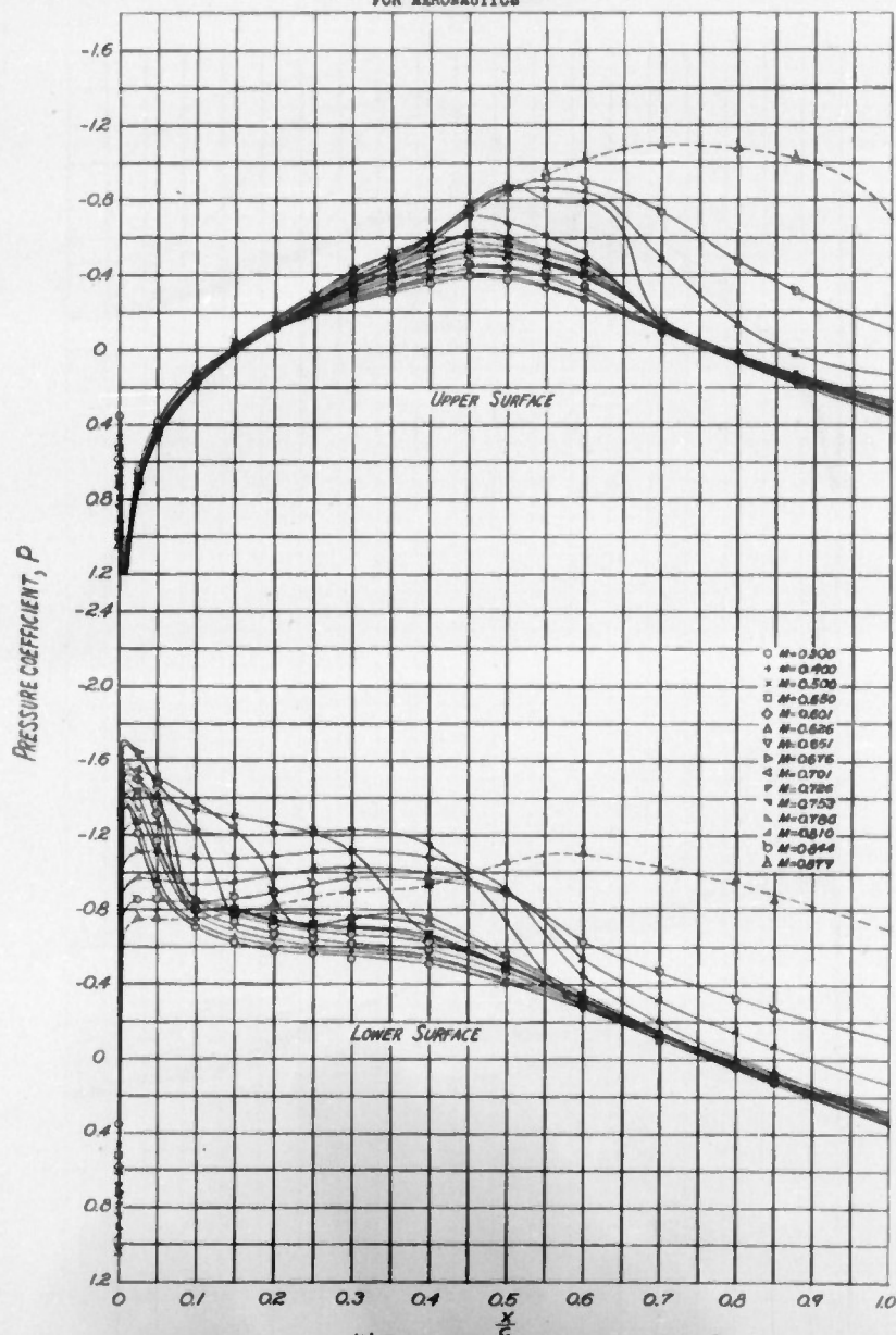
(b) SECTION ANGLE OF ATTACK, \alpha_0 = -4^\circ FIGURE 2- CONTINUED. NACA 65-215 ( a = 0.5 ) AIRFOIL SECTION
