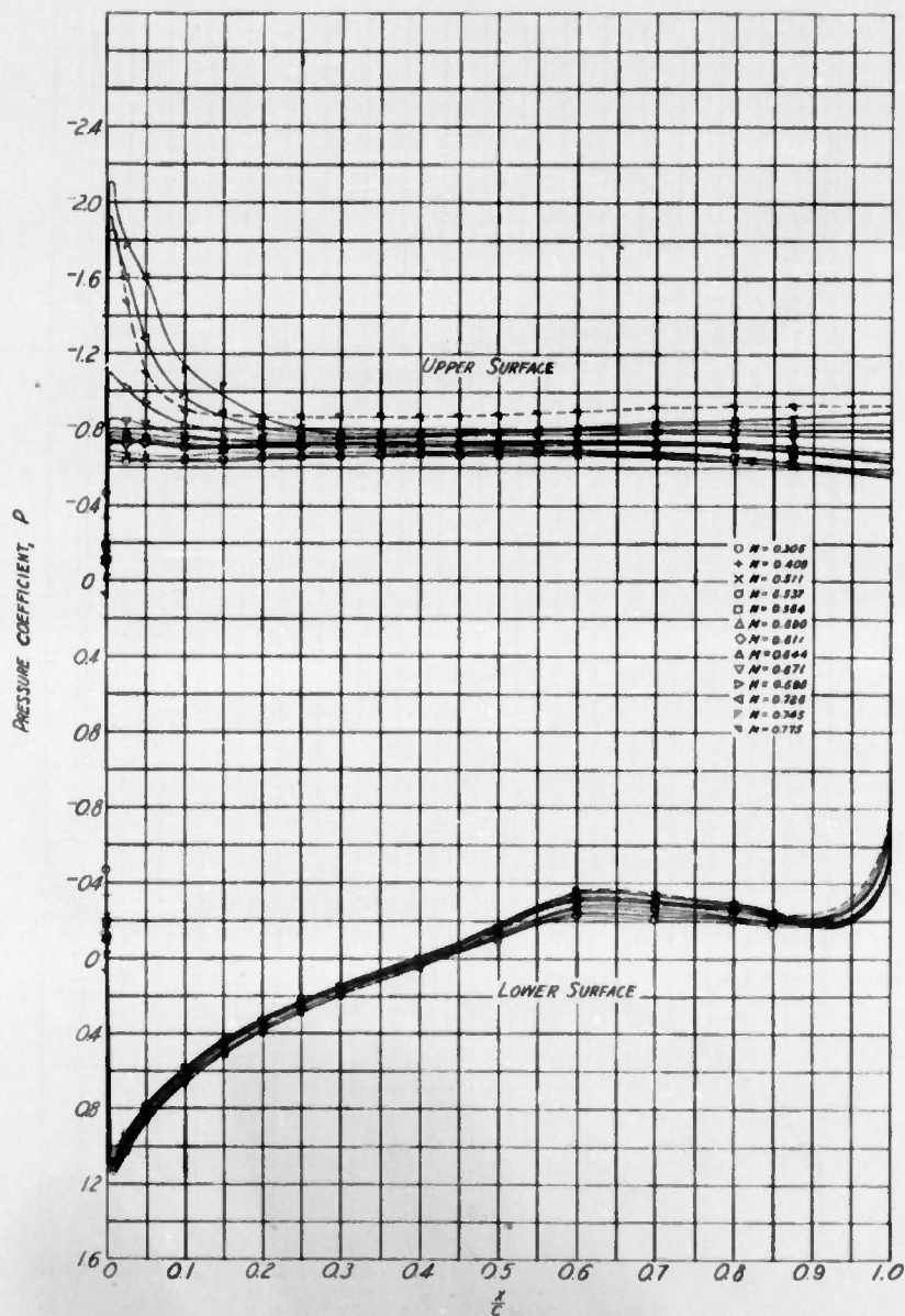
(2) SECTION ANGLE OF ATTACK, \alpha_0 = 16^\circ FIGURE 3.- CONCLUDED. NACA 66,215 ( a=0.6 ) AIRFOIL SECTION
