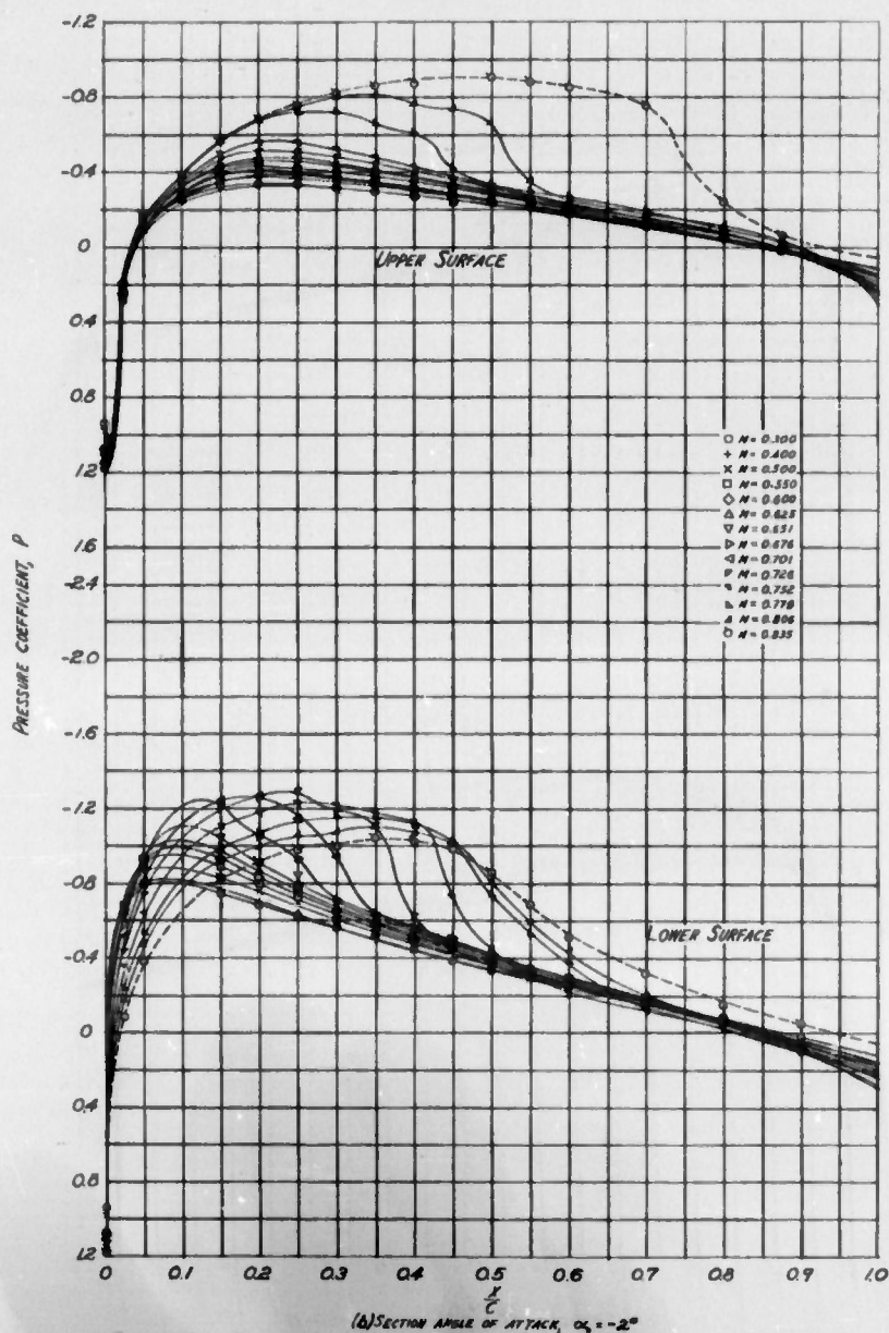
(b) SECTION ANGLE OF ATTACK, \alpha_s = -2^\circ FIGURE 4- CONTINUED. NACA 0015 AIRFOIL SECTION
