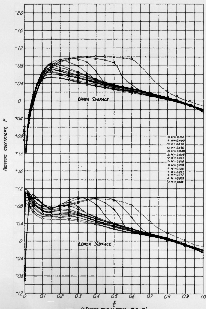
(c) SECTION ANGLE OF ATTACK, \alpha = -2^\circ FIGURE 5.- CONTINUED. NACA 23015 AIRFOIL SECTION
