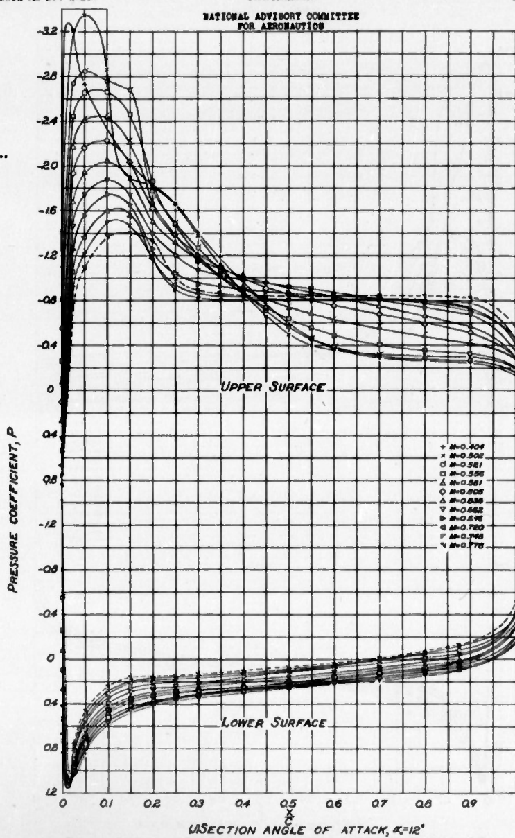
FIGURE 6.-CONTINUED. NACA 4415 AIRFOIL SECTION
