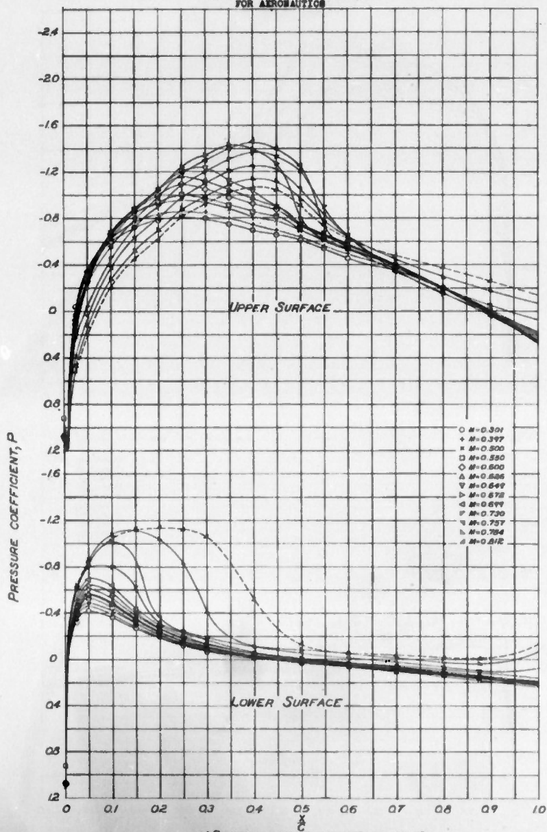
SECTION ANGLE OF ATTACK, \alpha = 0^\circ FIGURE 6-CONTINUED. NACA 4415 AIRFOIL SECTION
