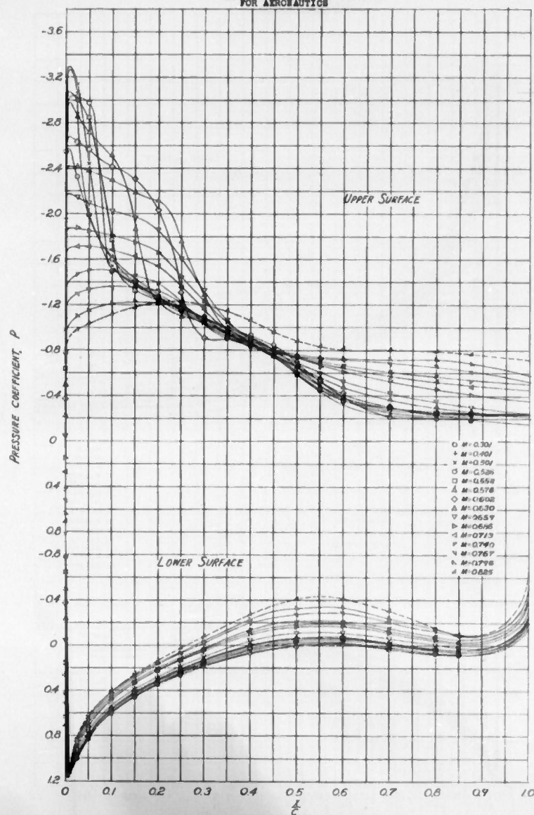
FIGURE 2-CONTINUED NACA 63-215 ( \alpha = 10^\circ ) AIRFOIL SECTION
