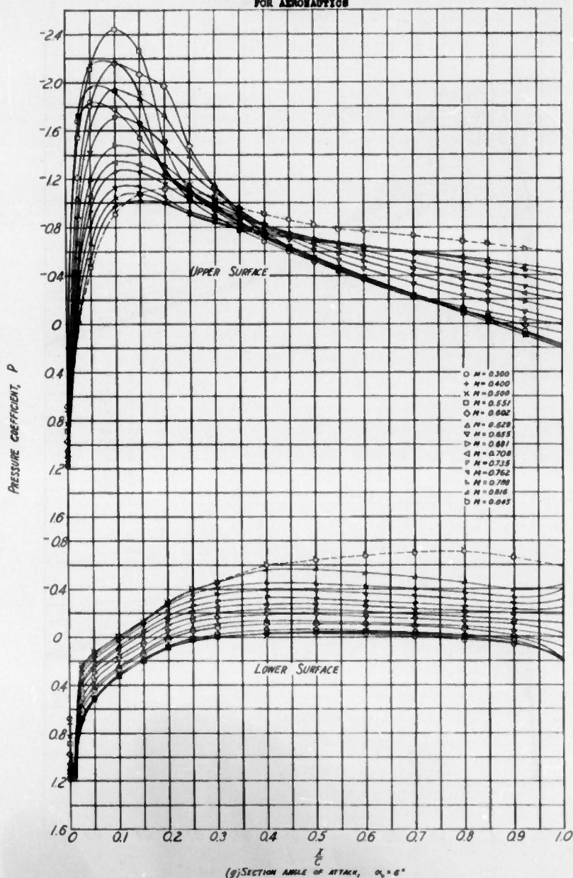
FIGURE 5- CONTINUED NACA 23015 AIRFOIL SECTION
