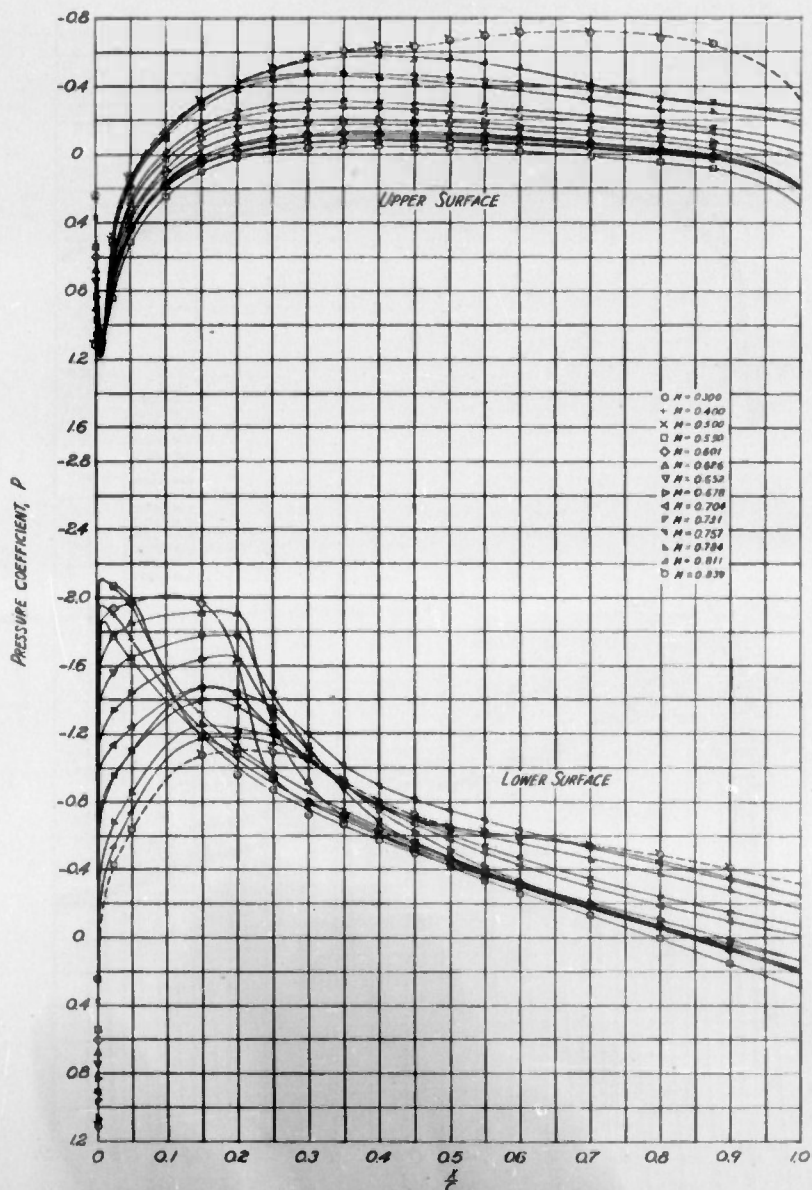
(d) SECTION ANGLE OF ATTACK, \alpha_s = -6^\circ FIGURE 4- CONTINUED. NACA 0015 AIRFOIL SECTION
