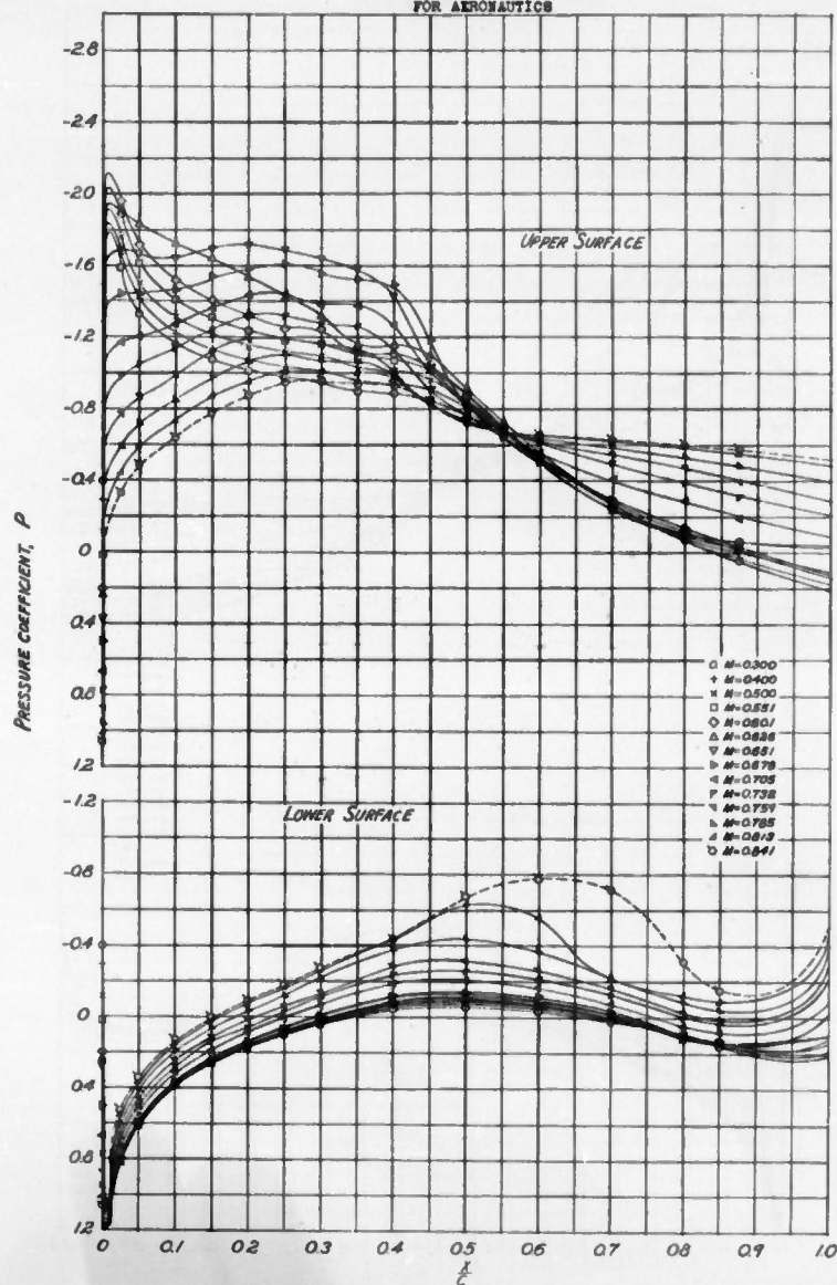
(g) SECTION ANGLE OF ATTACK, \alpha_s = 8^\circ FIGURE 2-CONTINUED NACA 63-215 ( \theta=0.5 ) AIRFOIL SECTION
