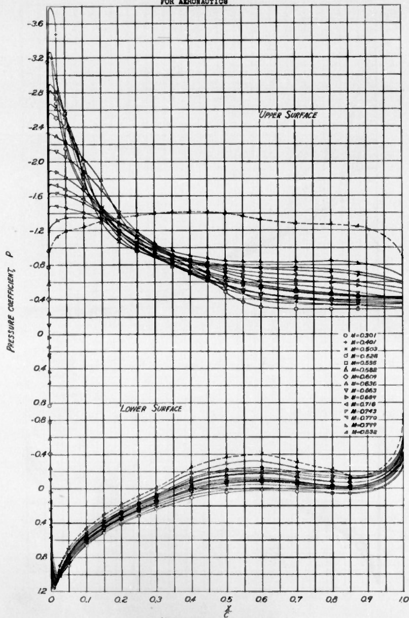
(j) SECTION ANGLE OF ATTACK, \alpha = 12^\circ FIGURE 2- CONTINUED NACA 65-215 ( \theta = 0.5 ) AIRFOIL SECTION
