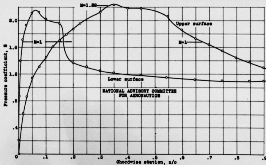
Figure 3.- Distribution of pressures over an NACA 4412 airfoil section at 0° angle of attack, Mach number 0.775, and Reynolds number 1.5 millions.
