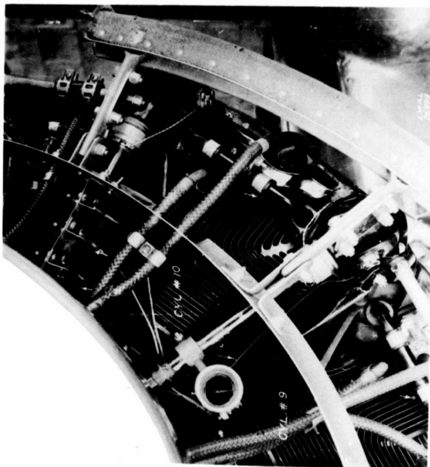
Figure 16.- Pressure tubes in baffles of cylinder 10.
