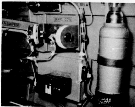
Figure 12.- Thermos bottle used as hot junction.
