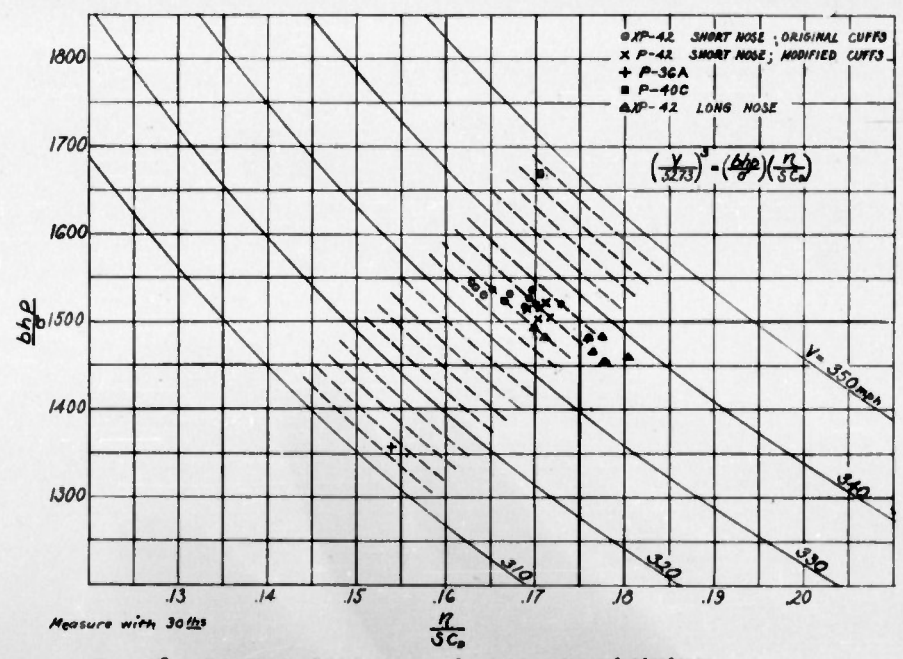
Figure 28.- Comparison of high-speed performance on several airplanes.
