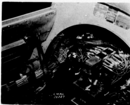
Figure 14.- Manometer and pressure- switch installation.
