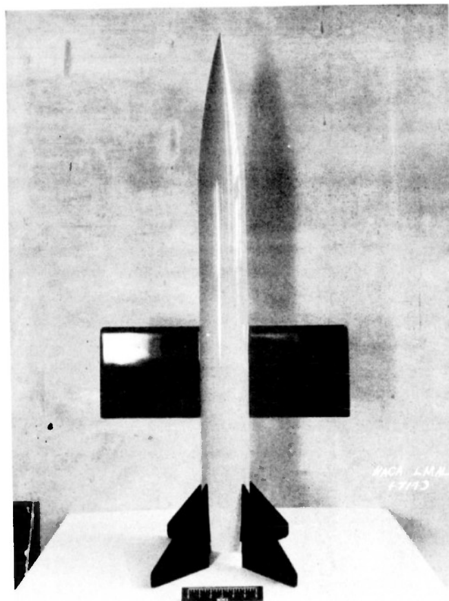
Figure 1.- General arrangement of typical winged test body.
