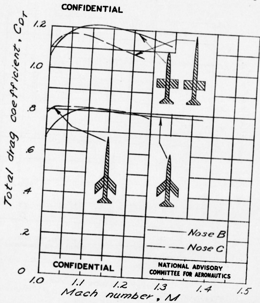
Figure 6.- Total drag coefficient for winged configurations of two nose types with wings of 0^\circ and 45^\circ sweepback, aspect ratio of 2.7.
