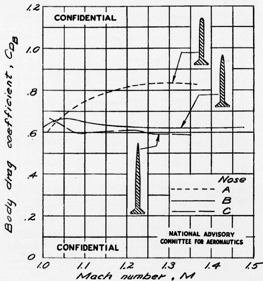
Figure 7.- Body drag coefficient for three nose shapes.
