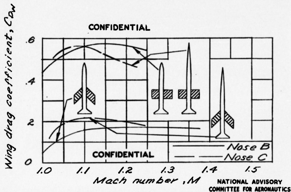
Figure 8.- Wing drag coefficient for wings of 0° and 45° sweepback in presence of bodies of two nose types, aspect ratio of 2.7.
