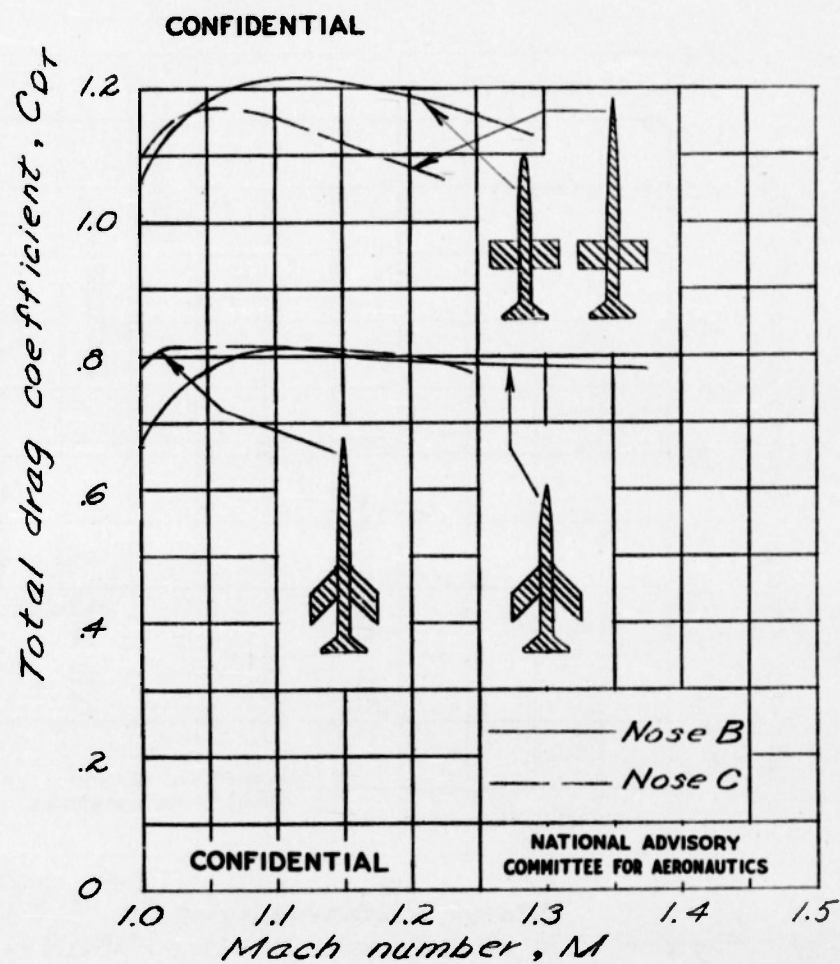
Figure 6.- Total drag coefficient for winged configurations of two nose types with wings of 0° and 45° sweepback, aspect ratio of 2.7.
