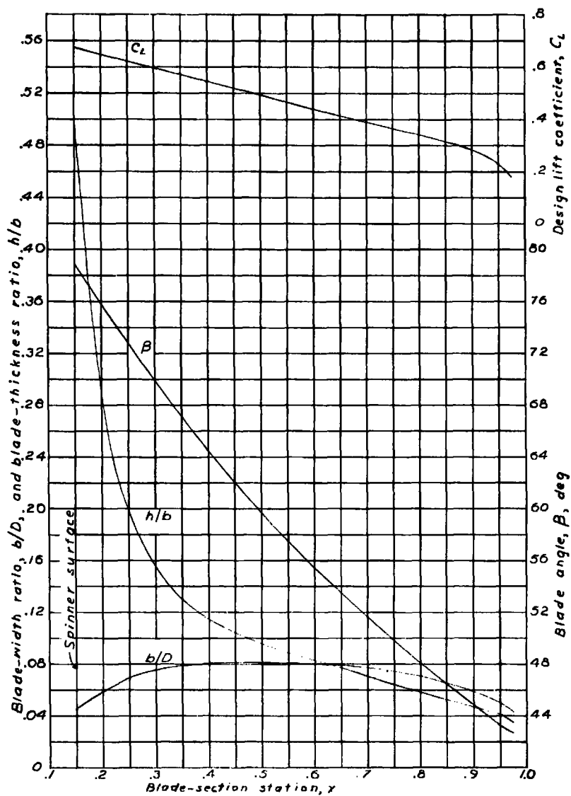
Figure 2. - NACA 4-(39107)-0345-B propeller blade-form curves.
