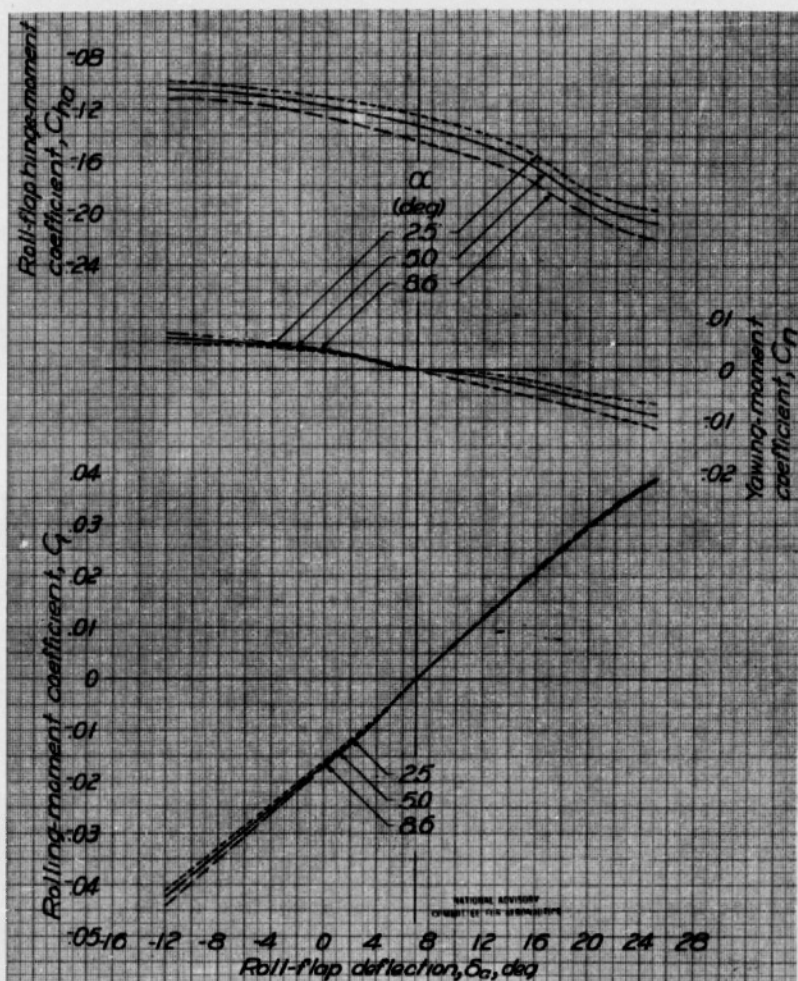
Figure 14.- Roll-flap characteristics with full-span flaps fully extended. Standard model configuration, \delta_f = 7^\circ , R = 5200,000 , M = 0.12 .
