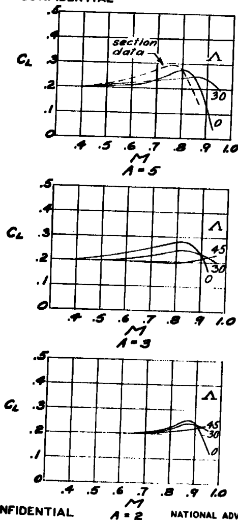
Figure 3. - Effect of compressibility on the lift coefficient of a wing with various aspect ratios and angles of sweepback.
