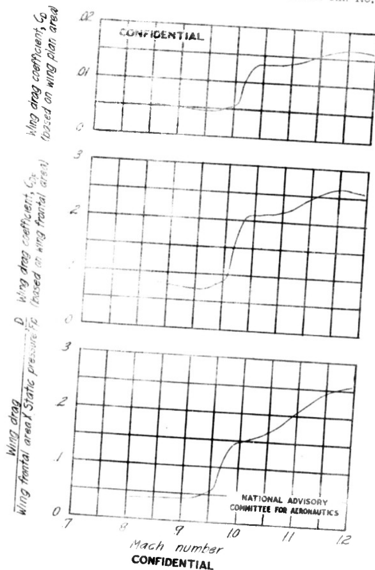
Figure 5.- Variation with Mach number of drag coefficients and D/F_p for the 45° half-back wing of the tested configuration.
