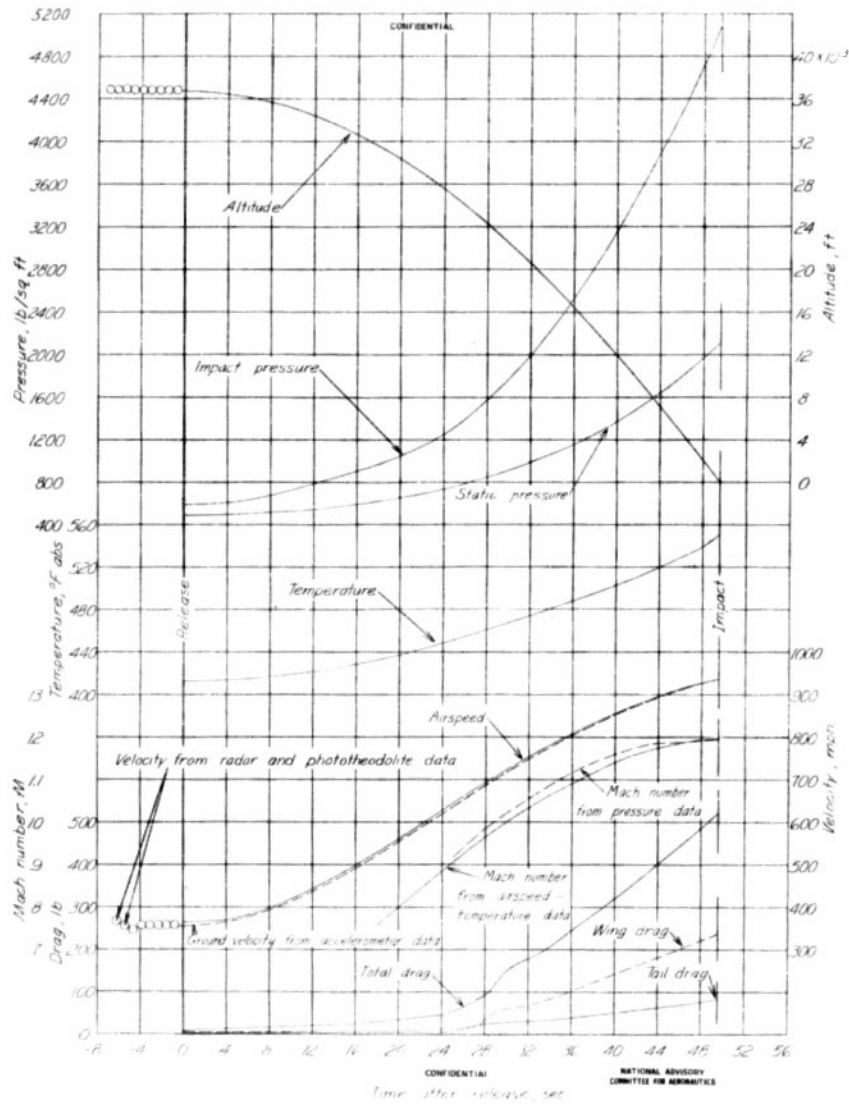
Figure 3.- Time history of free fall of wing-body configuration.
