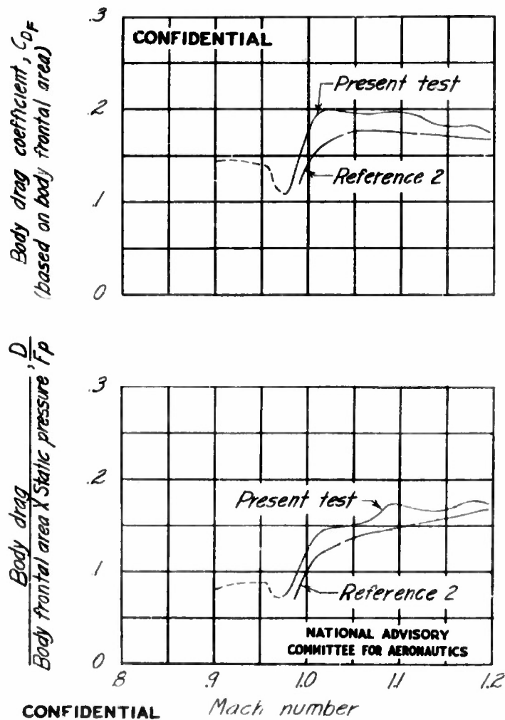
Figure 7.- Variation with Mach number of drag coefficient and D/\bar{F}_p for the body of the tested configuration. Data for identical body without wings taken from reference 2.
