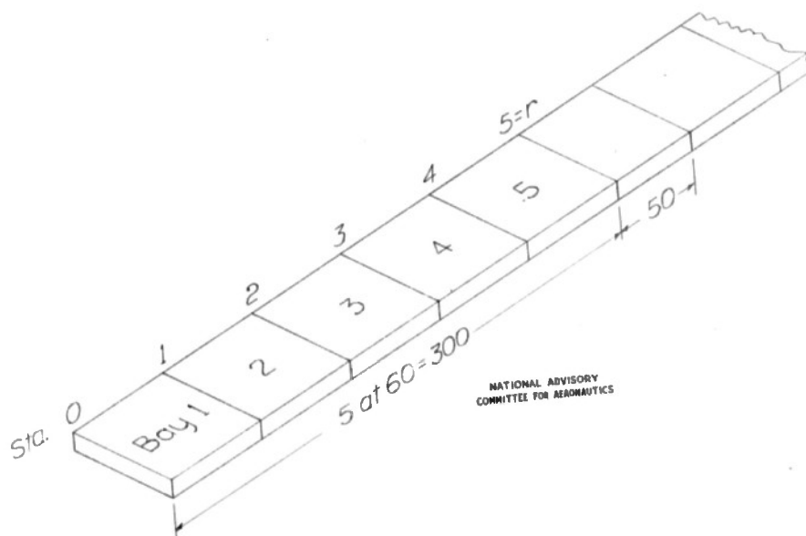
Figure 15.-Box beam for numerical examples.
