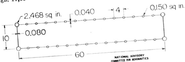
Figure 14.-Cross section of box beam for numerical examples.
