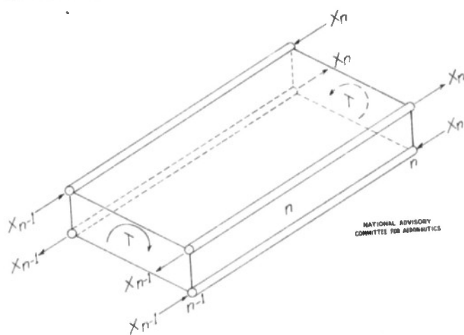
(b) Convention for positive forces acting on a bay.
