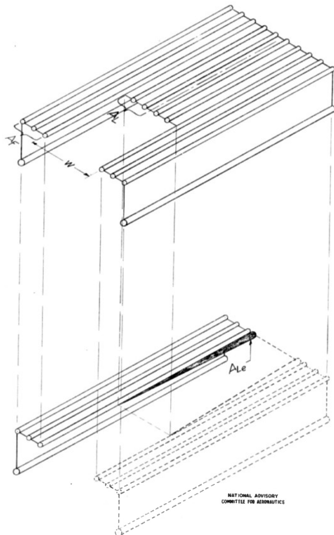
Figure 13.-Cut-out in cover of box beam.
