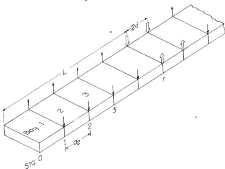
(a) Convention for numbering stations and bays.
