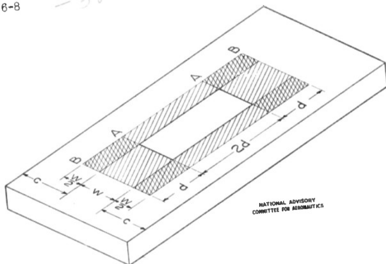
Figure 6.- Bay with small cut-out.
