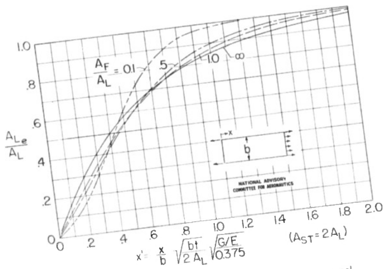
Figure 12.- Stringer effectiveness in axially loaded panel.
