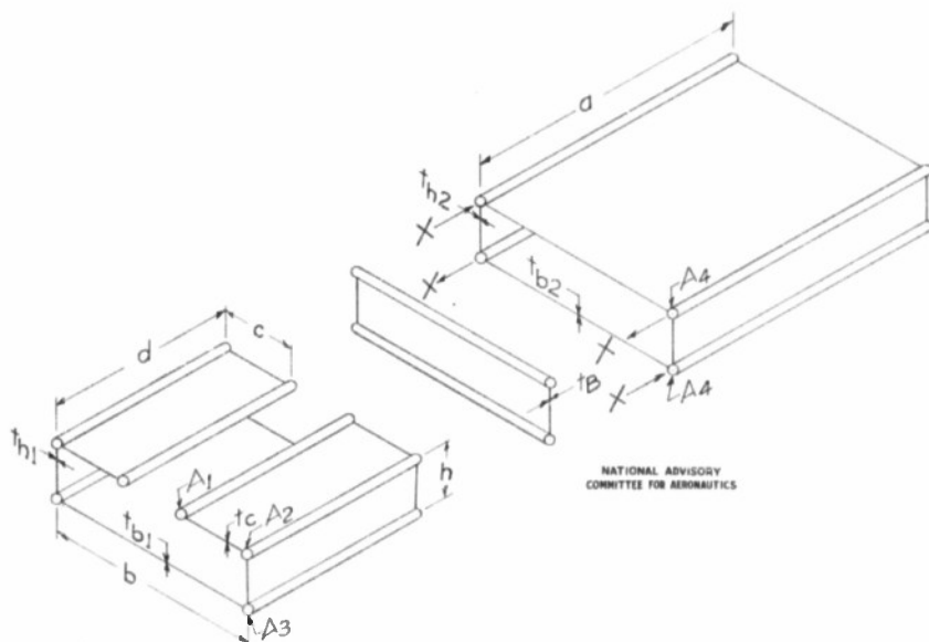
(b) Exploded view of half-structure.
