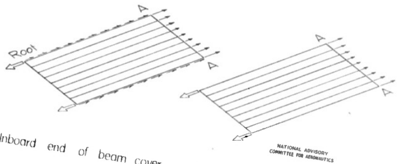
Figure 10.- Introduction of concentrated end loads.
