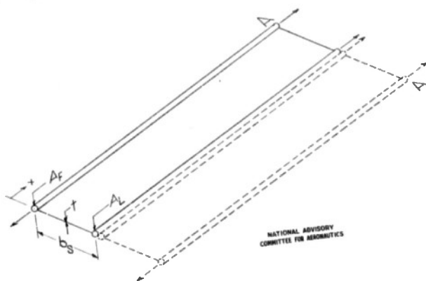
Figure 11.- Substitute single-stringer panel.
