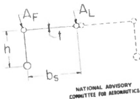
Figure 7.- Cross section of box idealized for shear-lag calculation.
