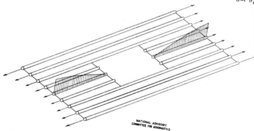
Figure 9.- Stresses in stringers interrupted by cut-out.
