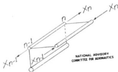
Figure 8.- Positive X-groups caused by shear lag acting on a bay.
