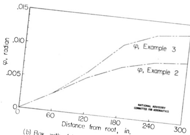
Figure 16.- Twist curves for numerical examples.
