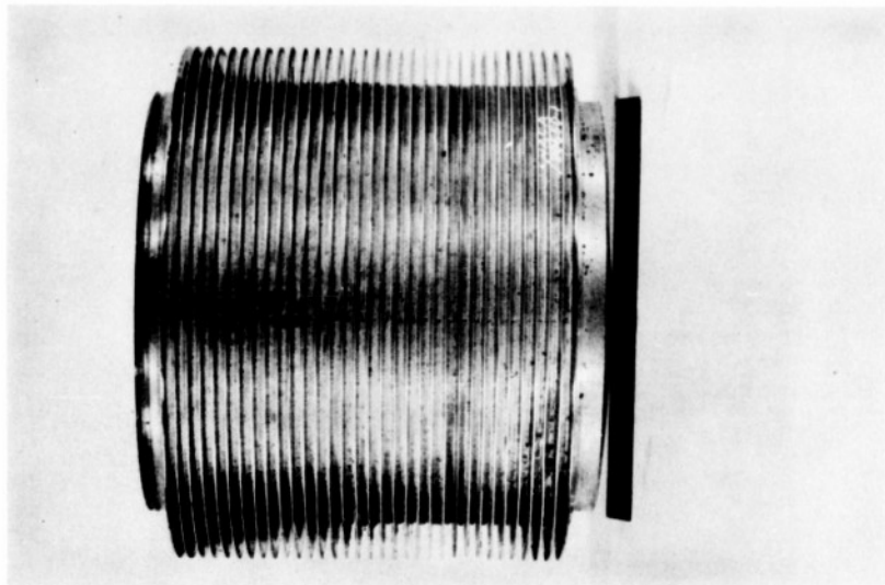
(b) Barrel with 0.09-inch fin space.
