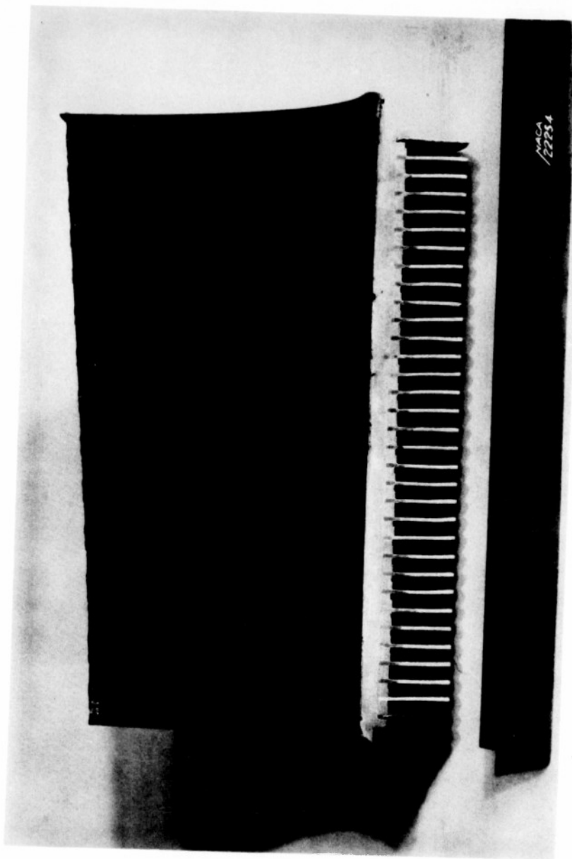
Figure 7. - Polished and etched section of cylinder showing fin outline.
