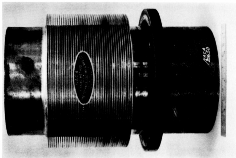
(a) Barrel with 0.052-inch fin space.
