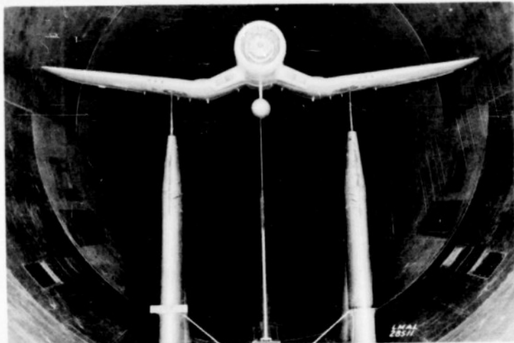
Figure 3.- Airplane model with the small circular external auxiliary fuel tank under the fuselage.
