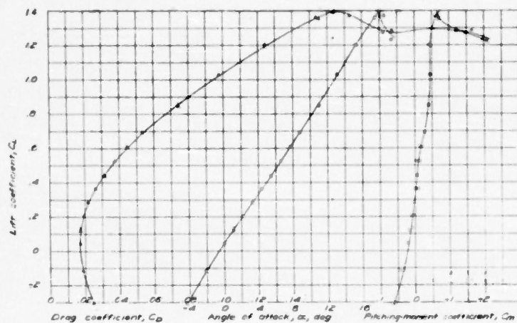
Figure 12- Variation of C_D , \alpha , and C_m with C_L for the airplane model without external auxiliary fuel tanks.
