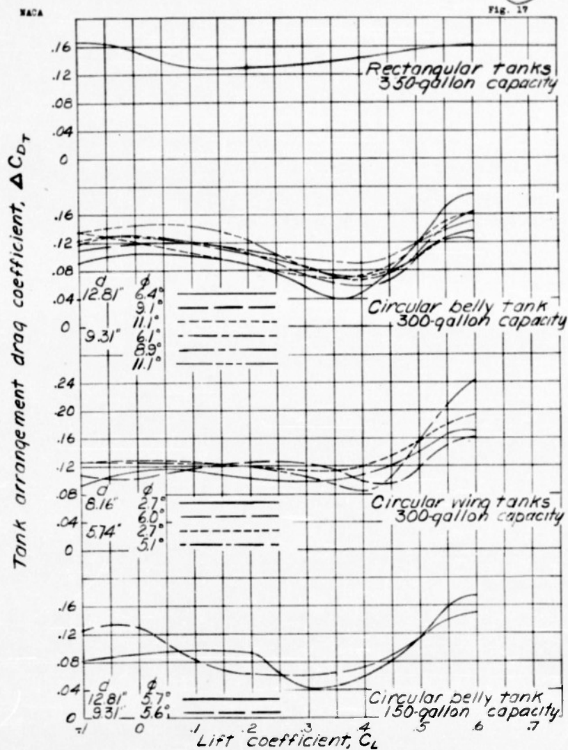
Figure 17:- Variation of \Delta C_{D_T} with C_L .
