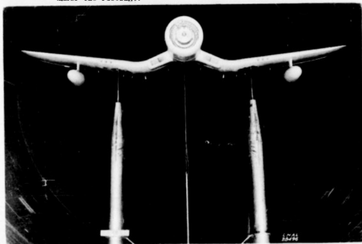
Figure 4.- Airplane model with the circular external auxiliary fuel tanks under the wing.
