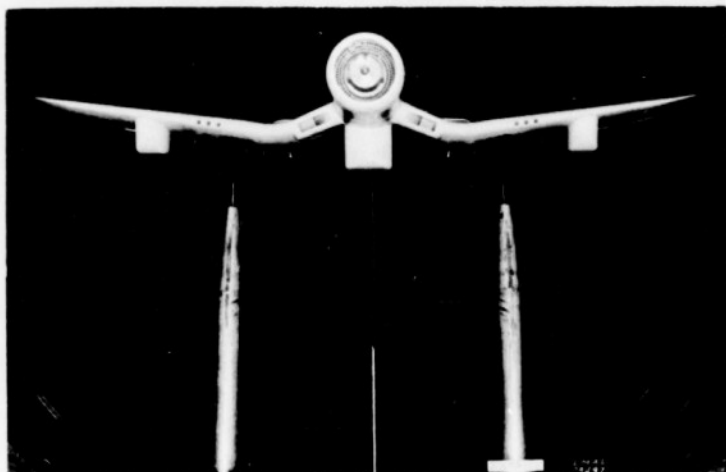
Figure 1.- Airplane model with the rectangular external auxiliary fuel tanks.
