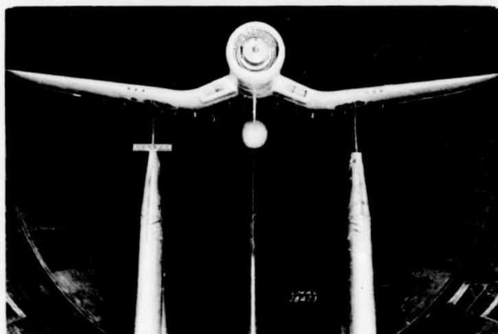
Figure 2.- Airplane model with the large circular external auxiliary fuel tank under the fuselage.
