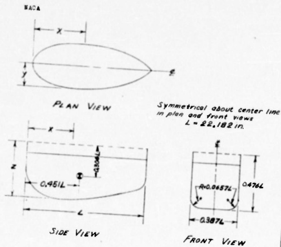
Figure 6.- Plan and elevation views of the small rectangular external auxiliary fuel tanks for the wing
