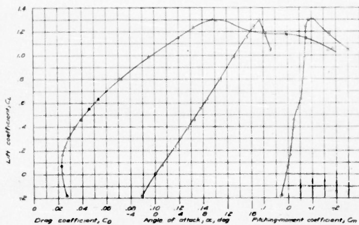
Figure 13- Variation of C_D , \alpha , and C_m with C_L for the airplane model with the rectangular external auxiliary fuel tanks.
