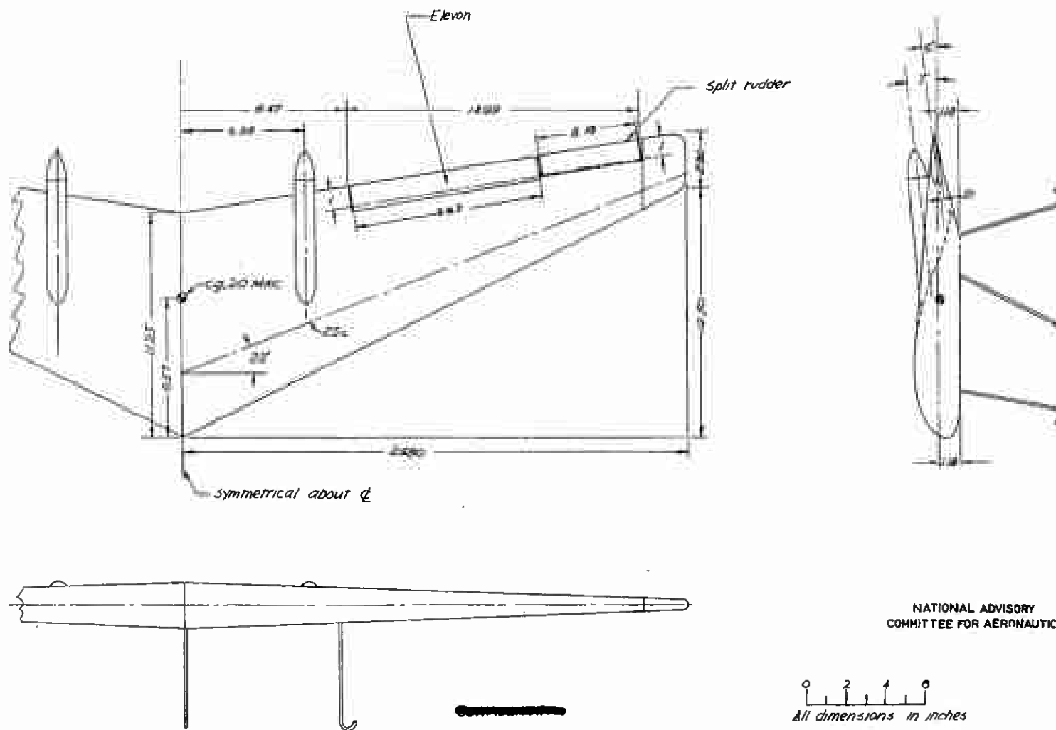
Figure 3.- Tailless airplane model tested in the Langley free-flight tunnel.
