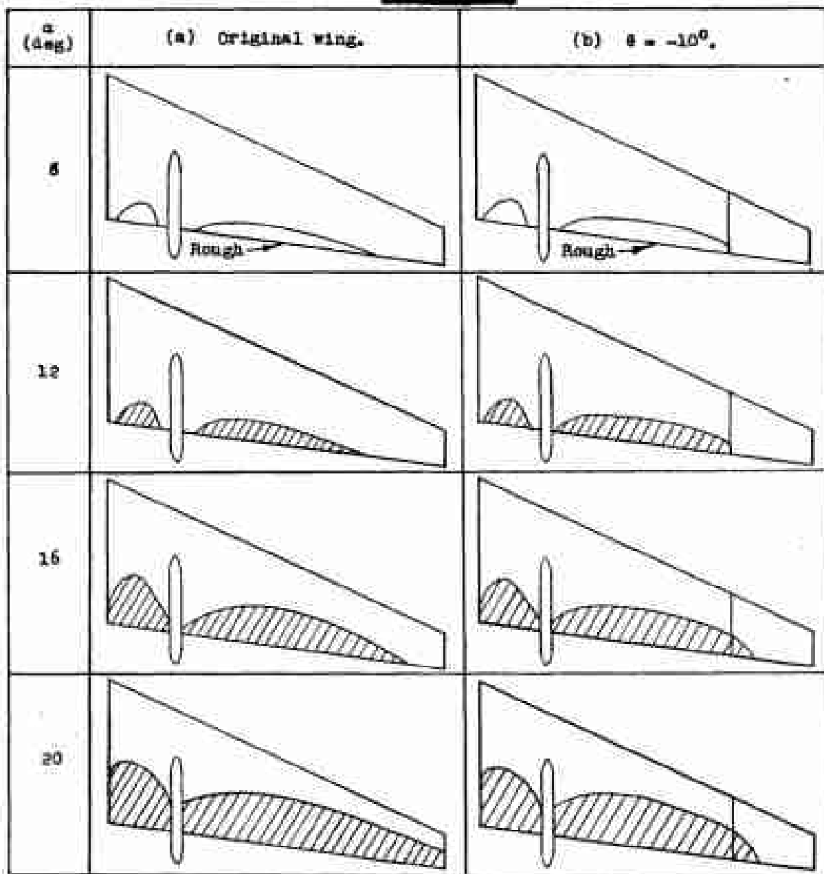
Figure 9.- Results of tuft surveys of tailless airplane model in Langley free-flight tunnel. \delta_o = \delta_r = \beta = 0^\circ ; q = 4.09 pounds per square foot.
