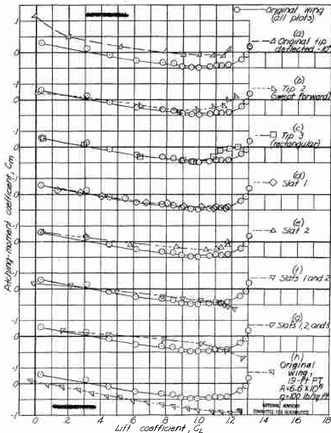
Figure 8.- Pitching-moment characteristics of Langley free-flight-tunnel failless airplane model with various wing modifications. \delta_o = \delta_r = 0^\circ ; flaps retracted; center-of-gravity location, 0.20 M.A.C.; q = 4.09 pounds per square foot except as noted.
