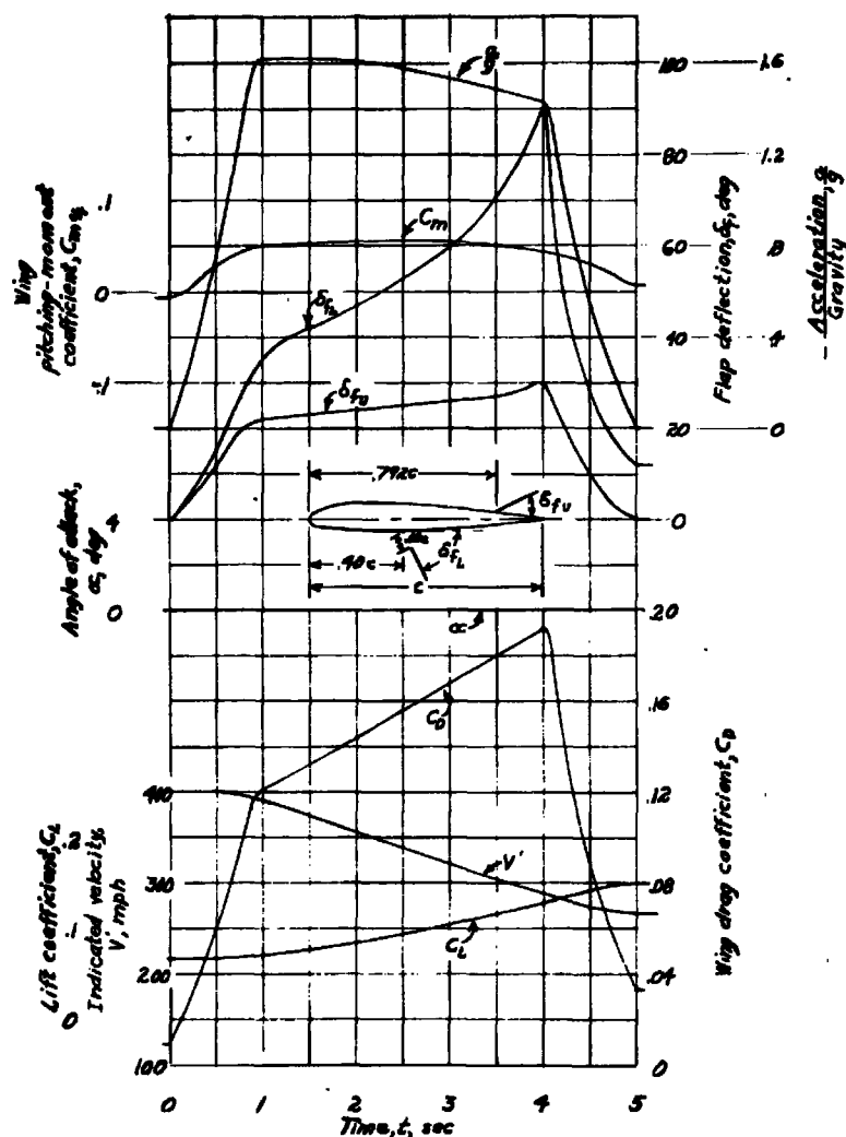
Figure 5.- Computed time-history characteristics during deceleration of the fighter airplane equipped with fighter brakes consisting of 0.208c by 0.525b perforated double split flaps. Upper flap located at 0.792c, lower flap at 0.40c with a 0.10c gap. Flap deflection for constant \alpha . (Computed for sea level)
