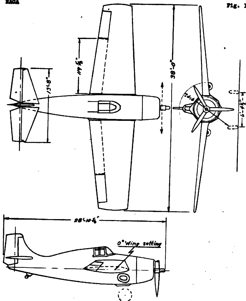
Figure 1.- Three-view drawing of the fighter airplane assumed in the computations.
