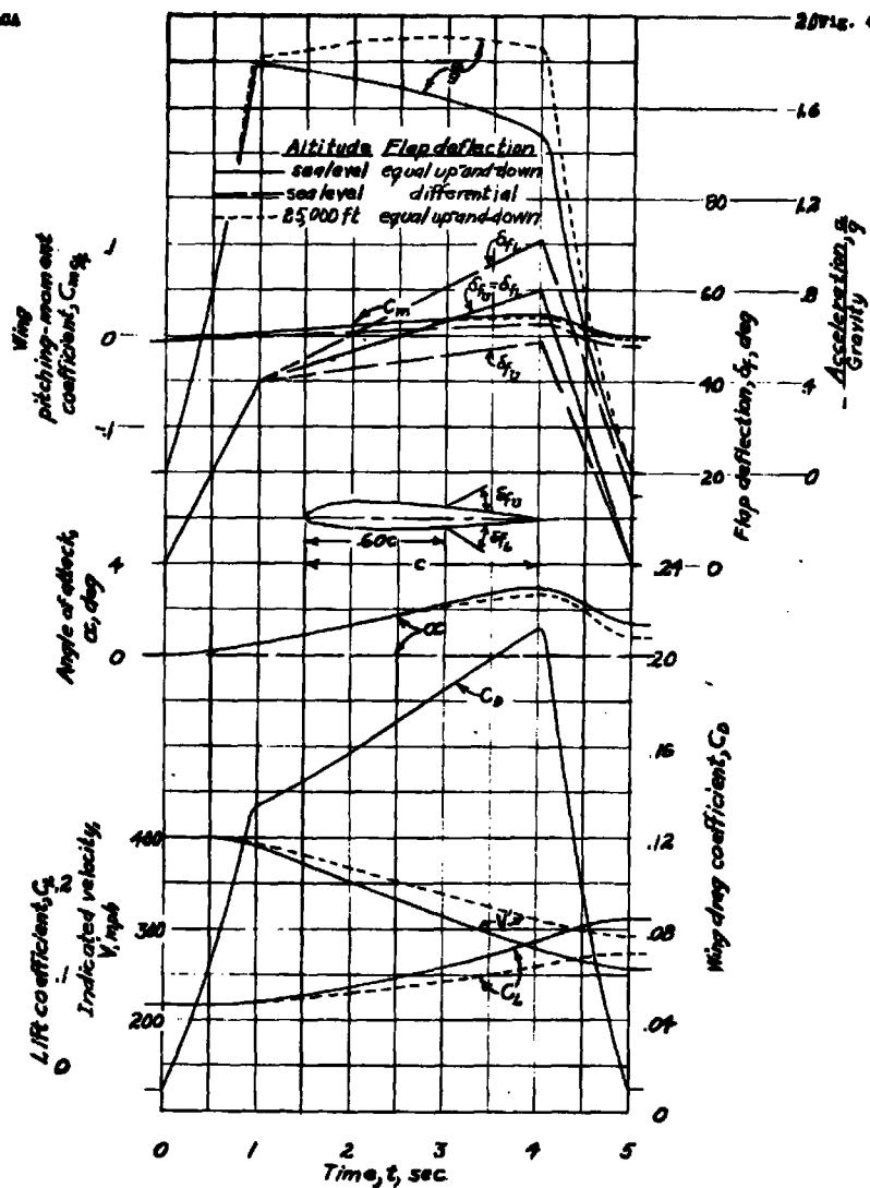
Figure 4.- Computed time-history characteristics during deceleration of the fighter airplane equipped with fighter brakes consisting of 0.208c by 0.525b perforated double split flaps. Flaps located at 0.60c.
