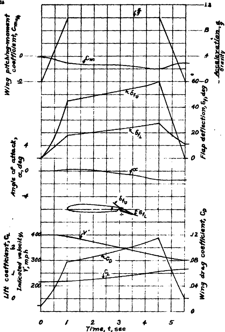
Figure 7 - Computed time-history characteristics during deceleration of the fighter airplane equipped with fighter brakes consisting of a Q208c by Q525b slotted flap and a Q15c by Q525b upper-surface perforated split flap. Computed for sea level. Upper flap located at Q80c. R.3-26-92
