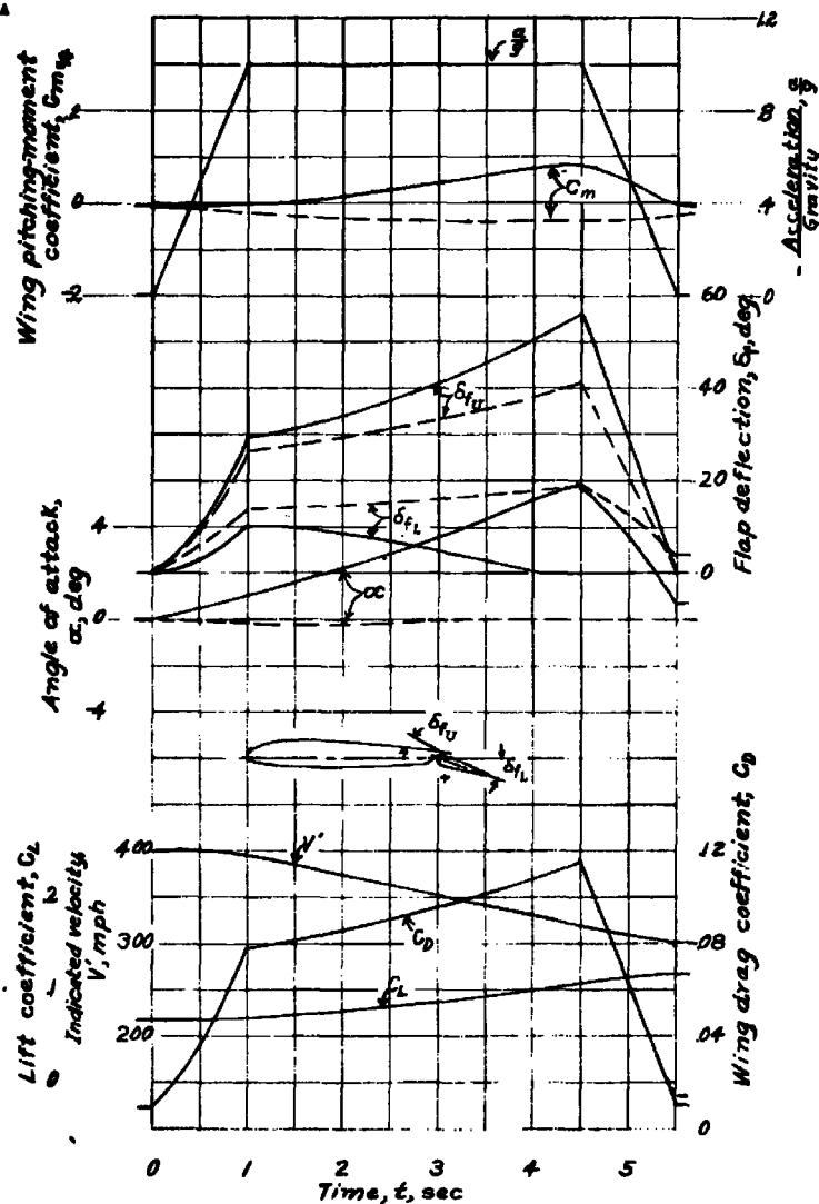
Figure 8 - Computed time-history characteristics during deceleration of the fighter airplane equipped with fighter brakes consisting of a Q208c by Q525b slotted flap and a Q20c by Q525b upper-surface perforated split flap (Computed for sea level). Upper-surface flap located at 0.80c. Two flap deflection systems. 93-4-11
