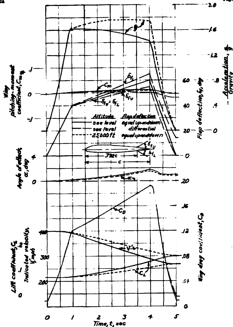
(a) Effects of altitude and differential flap operation.
