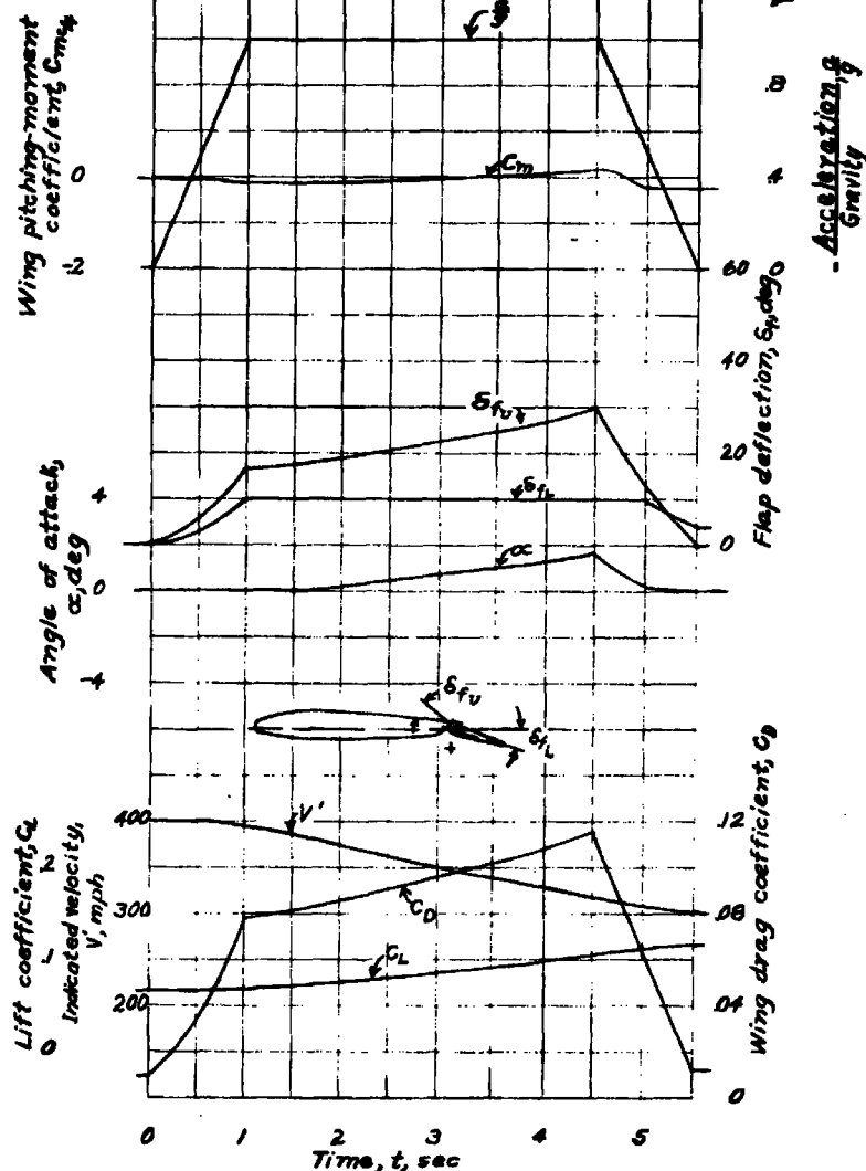
Figure 9 - Computed time-history characteristics during deceleration of the fighter airplane equipped with fighter brakes consisting of a 0.208c by 0.525b slotted flap and a 0.25c by 0.525b upper-surface perforated split flap. (Computed for sea level)
