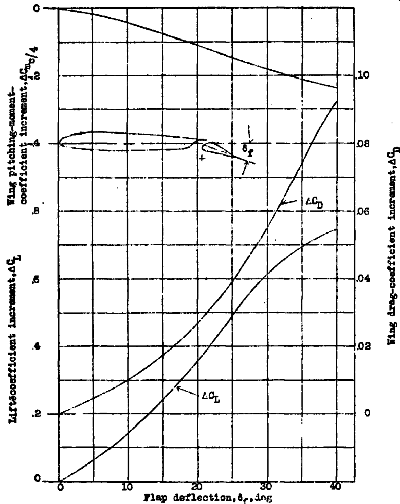
Figure 2.- Estimated increments of lift, drag, and pitching-moment coefficients due to deflecting a) 0.208 c by 0.525 b) slotted flap on the wing of a fighter airplane \alpha = 0^\circ .
