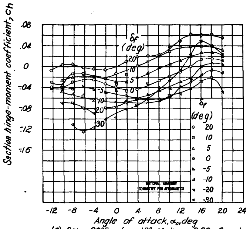
(c) Gaps, 0.005c; \delta_{t_0} = -10^\circ ; \partial \delta_t / \partial \delta_f = -0.20 . Concluded. Figure 6.- Concluded.
