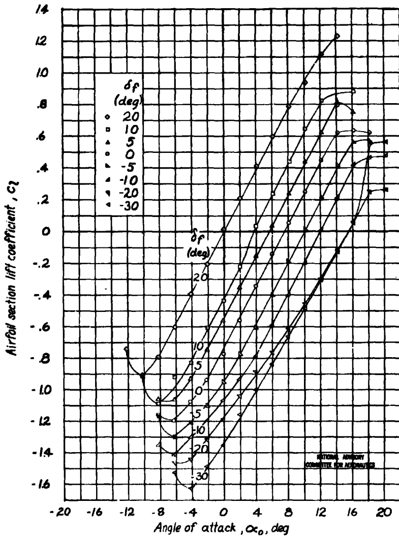
Figure 10.- Aerodynamic section characteristics of an NACA 0009 airfoil having a 0.25c flap and a 2.00c f tab. Gaps sealed; \delta_{t_0} = -10^\circ ; \partial \delta_t / \partial \delta_f = -0.10 .
