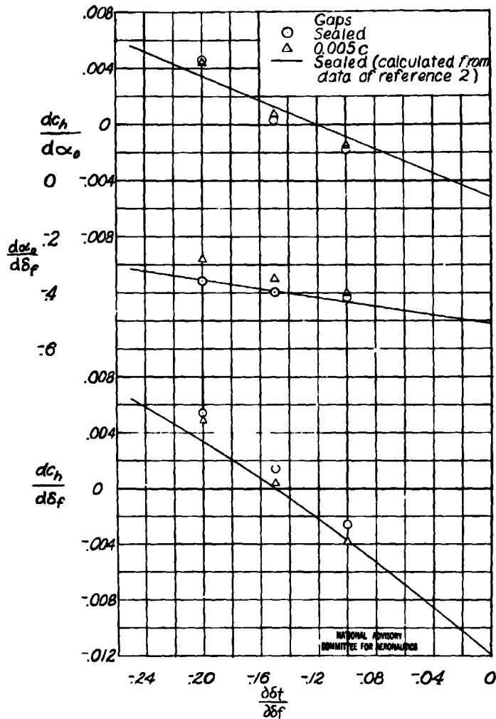
Figure 3 - Comparison of the aerodynamic characteristics of the 2.00c f lab on NACA 0009 airfoil obtained from experiment and from calculations.
