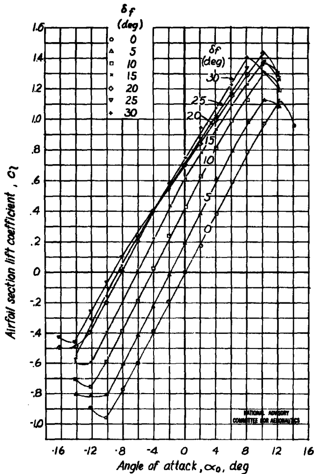
(a) Gaps sealed; \delta t_0 = 0^\circ ; \partial \delta t / \partial \delta_f = -0.10 Figure 8.- Aerodynamic section characteristics of an NACA 0009 airfoil having a 0.25c flap and a 2.00c f tab with various linkages.
