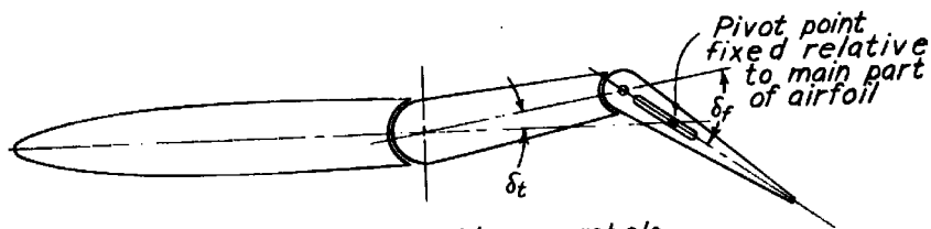
(c) Definition of deflection symbols.
