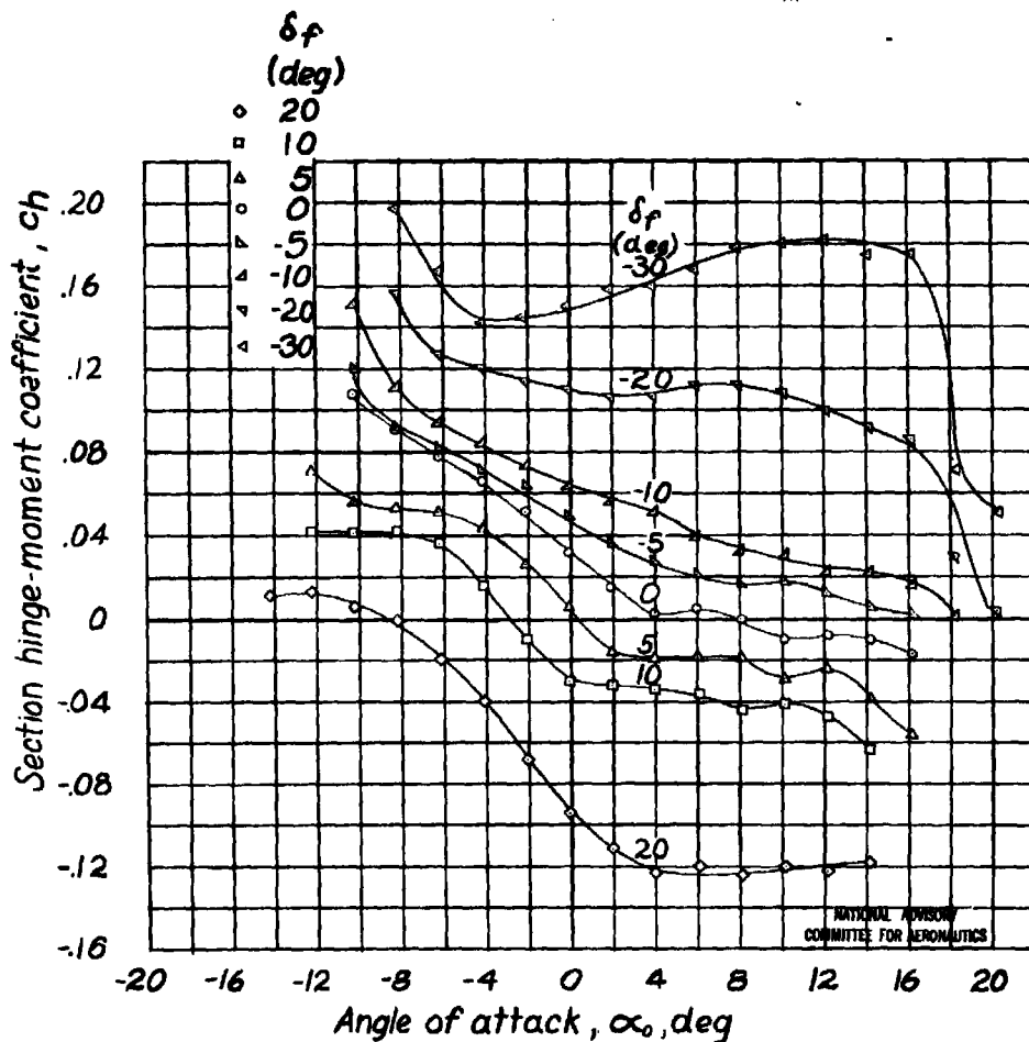
(a) Gaps, 0.005c ; \delta t_0 = -10^\circ ; \partial \delta t / \partial \delta_f = -0.10 . Concluded.
