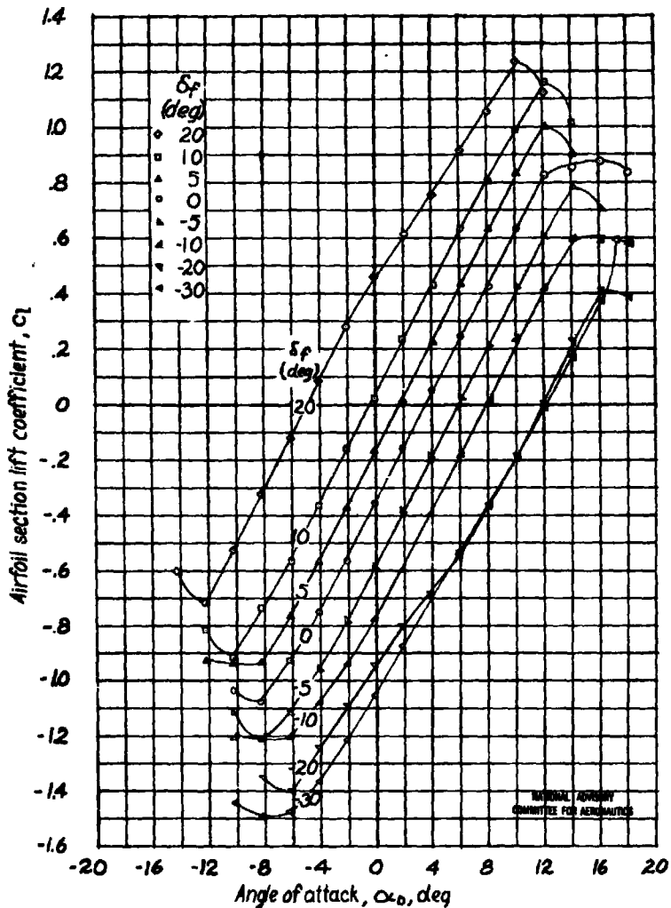
Figure 9.- Aerodynamic section characteristics of an NACA 0009 airfoil having a 0.25c_f flap and a 2.00c_f tab. Gaps sealed; \delta_{t_0} = -5^\circ ; \delta\delta_{t_0}/\delta\delta_f = -0.10 .
