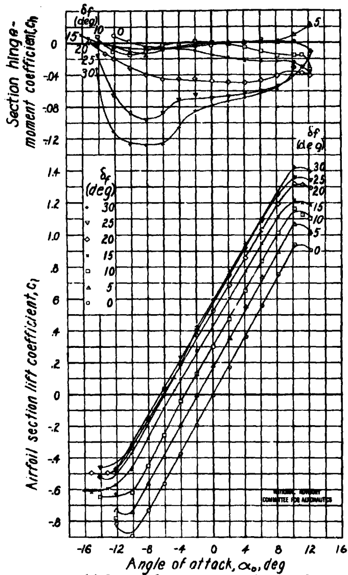
(b) Gaps, 0.005c , \delta\alpha_0 = 0^\circ ; \partial\delta_f/\partial\alpha_f = -0.15 . Figure 4.- Continued.
