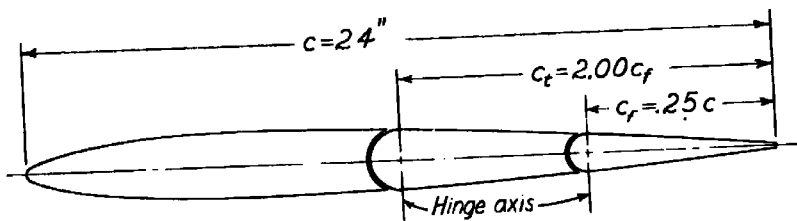
(a) Chord dimensions of airfoil.
