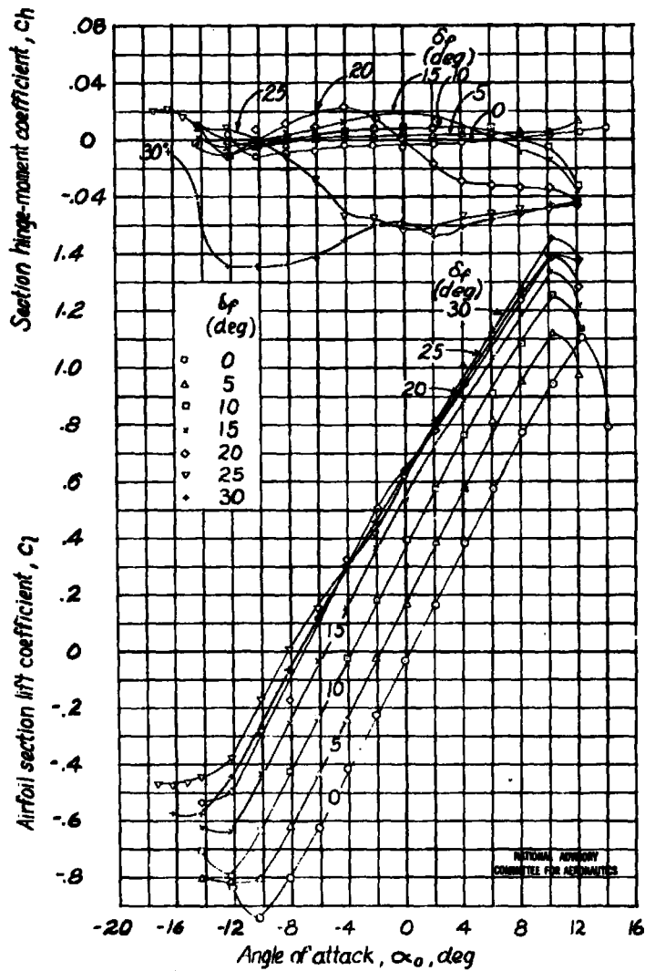
(b) Gaps sealed; \delta t_0 = 0^\circ ; \delta \delta t / \delta \delta f = -0.15 . Figure 8.- Continued.
