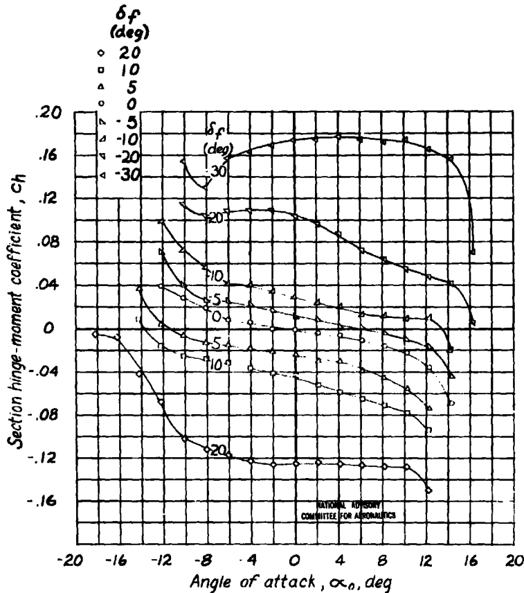
(a) Gaps, 0.005c; \delta_0 = 0^\circ ; \delta_f/\delta_p = -0.10 . Concluded. Figure 4. - Continued.
