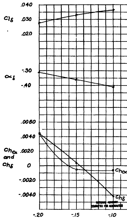
\frac{\partial \delta_t}{\partial \delta_f} (b) \delta_{t_0} = -5^\circ , gaps, 0.005c. Figure 12 - Continued.
