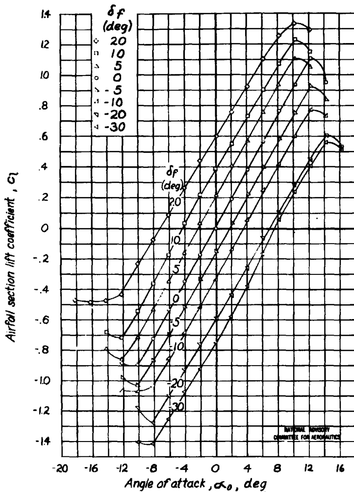
(a) Gaps, 0.005c ; \delta_{t_0} = 0^\circ , \partial \delta_t / \partial \delta_f = -0.10 . Figure 4.- Aerodynamic section characteristics of an NACA 0009 airfoil having a 0.25c flap and a 2.00c_f tab with various linkages.
