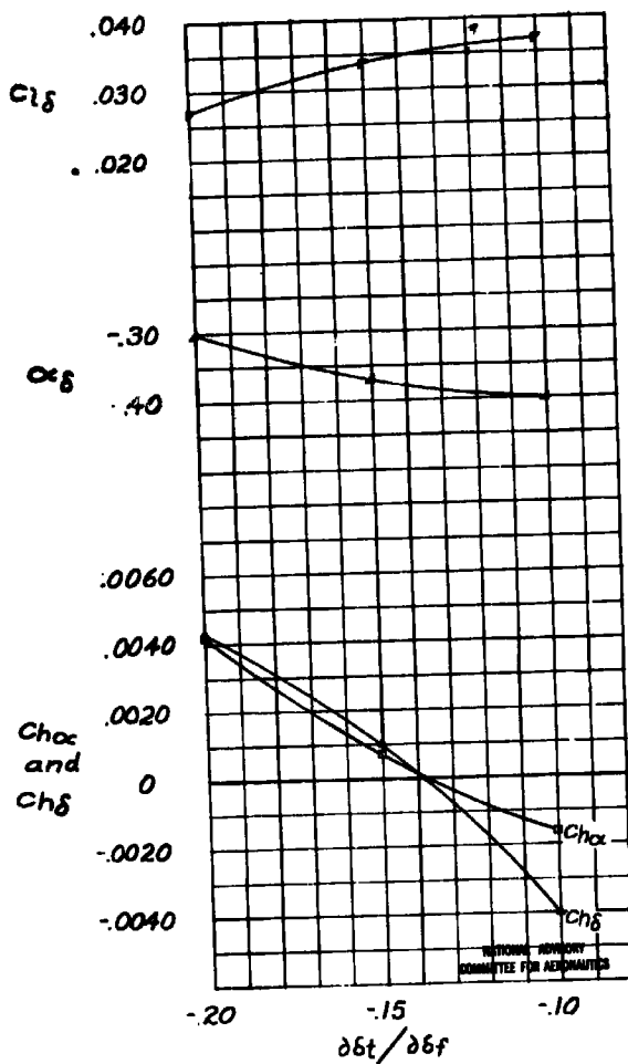
(c) \delta_t = -10^\circ ; gaps, 0.005c. Figure 12. - Continued.
