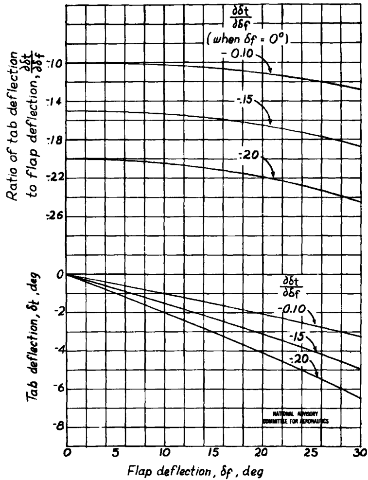
Figure 2.- Characteristics of linkage tested on the NACA 0009 airfoil with a 0.25c flap and a 2.00cf tab.
