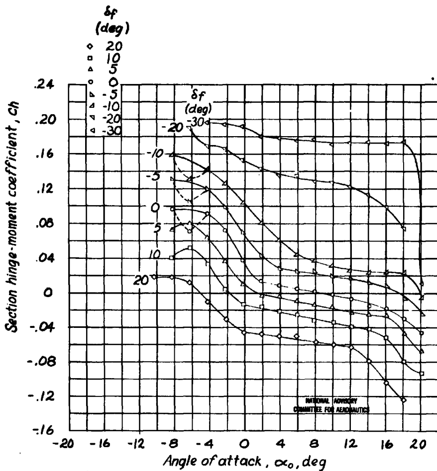
(a) Gaps sealed; St_0 = -15^\circ ; \partial \delta f / \partial \delta f = -0.10 . Concluded. Figure 11.- Continued.
