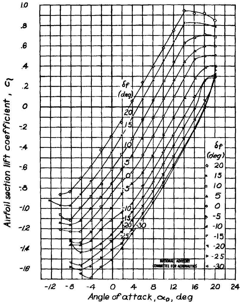
(a) Gaps, 0.005c ; \delta t_0 = -15^\circ ; \delta \delta_f / \delta \delta_f = -0.10 . Figure 7.- Aerodynamic section characteristics of an NACA 0009 airfoil having a 0.25c flap and a 2.00c_f tab with various linkages.
