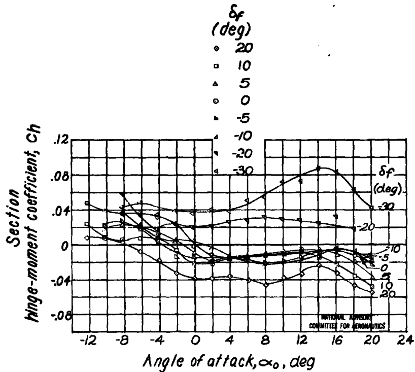
(b) Gaps, 0.005c; \delta_{t_0} = -10^\circ ; \partial \delta_t / \partial \delta_f = -0.15 . Concluded.
