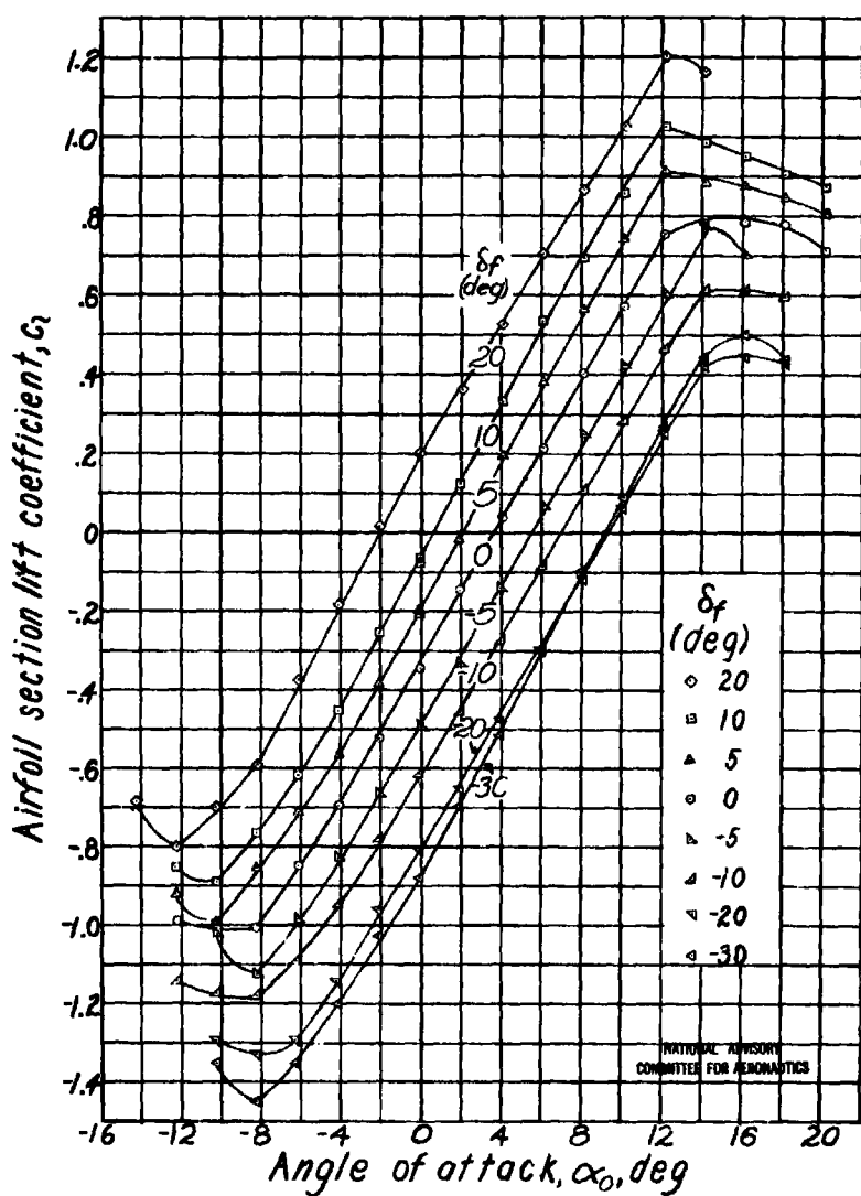
(c) Gaps, 0.005c ; \delta t_0 = -5^\circ ; \partial \delta t / \partial \delta f = -0.20 . Figure 5.- Continued.
