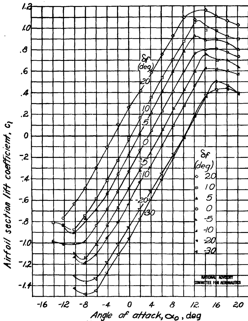
(b) Gaps, 0.005c; \delta t_0 = -5^\circ ; \partial \delta t / \partial \delta_f = -0.15 . Figure 5 - Continued.
