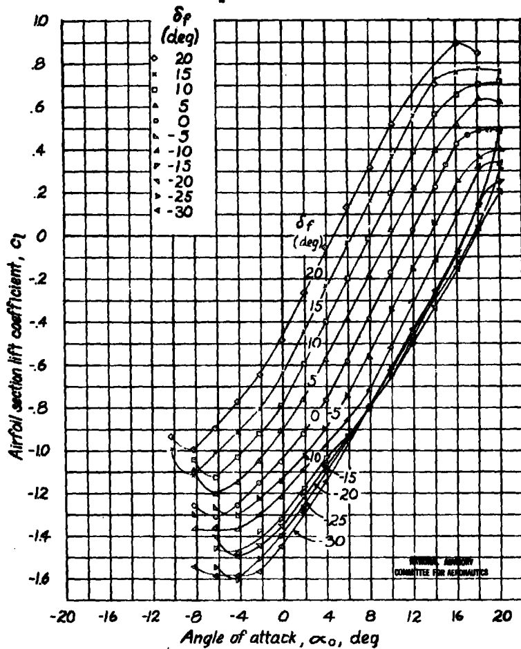
(c) Gaps sealed; \delta t_o = -15^\circ ; \delta \delta_f / \delta \delta_f = -0.20 . Figure 11. - Continued.
