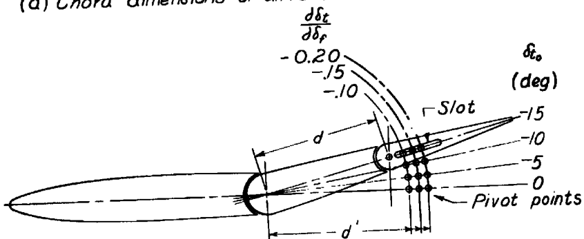
(b) Position of tab when used for trimming. \delta_f = 0^\circ .
