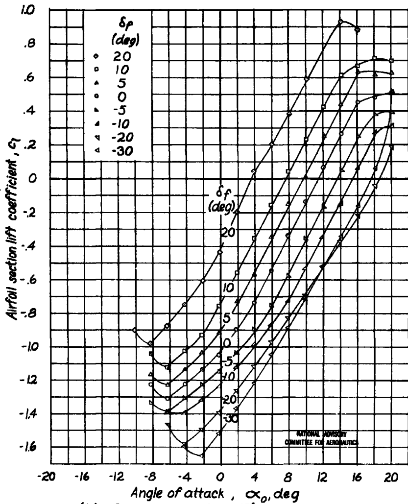
(b) Gaps sealed; \delta t_0 = -15^\circ ; \partial \delta t / \partial \delta f = -0.15 . Figure 11. - Continued.
