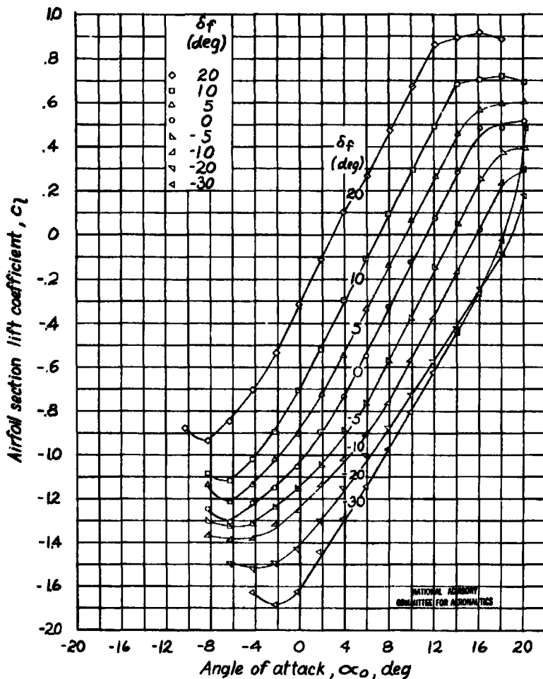
Figure 11. - Aerodynamic section characteristics of an NACA 0009 airfoil having a 0.25c flap and a 2.00c f tab with various linkages.
