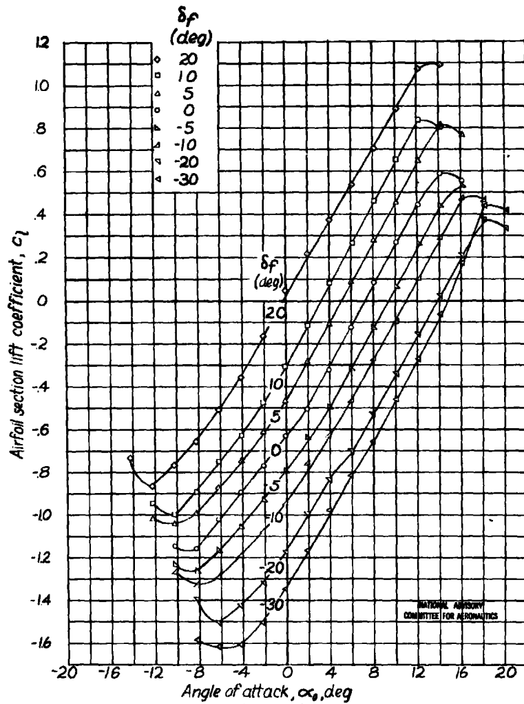
Figure 6.- Aerodynamic section characteristics of an NACA 0009 airfoil having a 0.25c flap and a 2.00c_f tab with various linkages.
