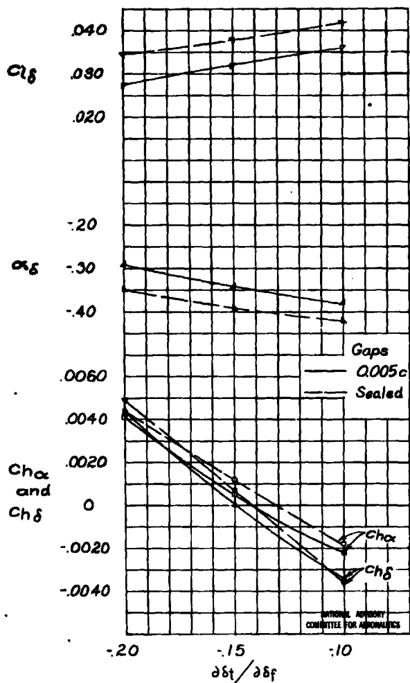
(d) \delta t_0 = -15^\circ ; gaps open and sealed. Figure 12. - Concluded.
