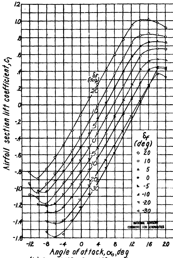
(b) Gaps, 0.005c ; \delta t_0 = -10^\circ ; \partial \delta t / \partial \delta f = -0.15 . Figure 6.- Continued.
