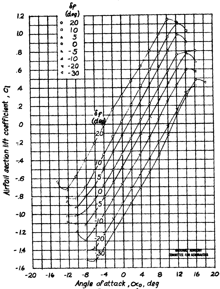
Figure 5.- Aerodynamic section characteristics of an NACA 0009 airfoil having a 0.25c flap and a 2.00c f tab with various linkages.
