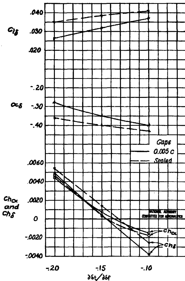
Figure 12. - Variation of parameters with ratio of tab deflection to flap deflection. c_1 = 0 .
