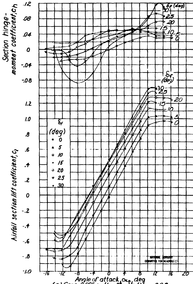
(c) Caps, 0.005c; \delta_{f_0} = 0^\circ ; \delta \delta_f / \delta \delta_f = -0.20 . Figure 4. - Concluded
