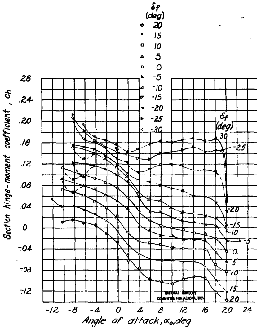
(a) Gaps, 0.005c; \delta t_0 = -15^\circ ; \delta t / \delta \delta_f = -0.10 . Concluded. Figure 7.-Continued.
