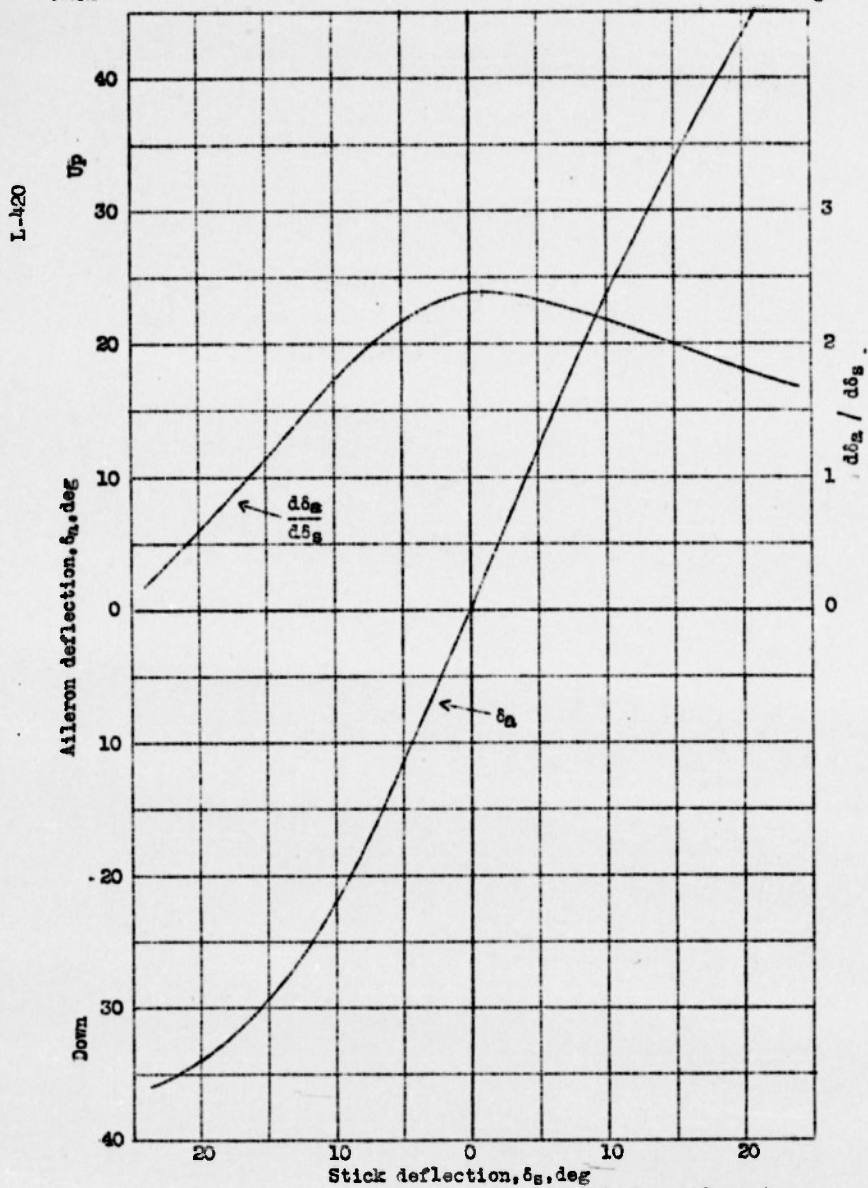
Figure 14.-- Spoiler-slot aileron-control linkage characteristics for a pursuit-type airplane. Effective stick length, 21 inches; maximum stick deflection \pm 24^\circ .
