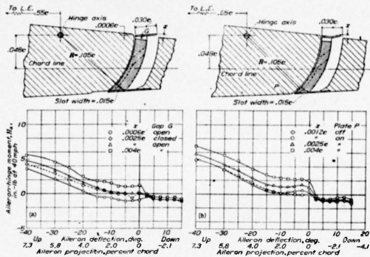
Figure 7.- The effect on the hinge-moment characteristics of tilting or bending the upper surface plate of an 0.37 b/2 spoiler-slot aileron on an NACA 23012 wing with a 0.2566c full-span slotted flap. Arrangement B, \alpha , 10^\circ , C_L , 0.15. Flap neutral.
