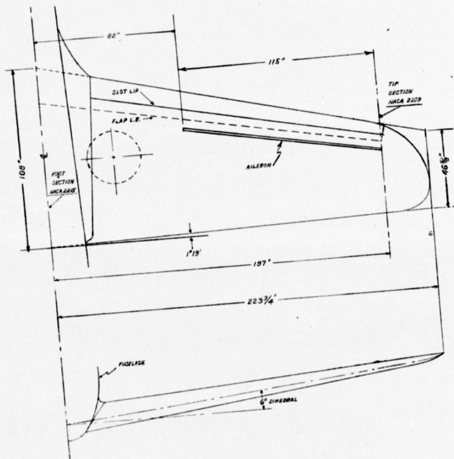
Figure 11.- Wing arrangement of the spoiler-slot aileron control system for a pursuit-type airplane.
