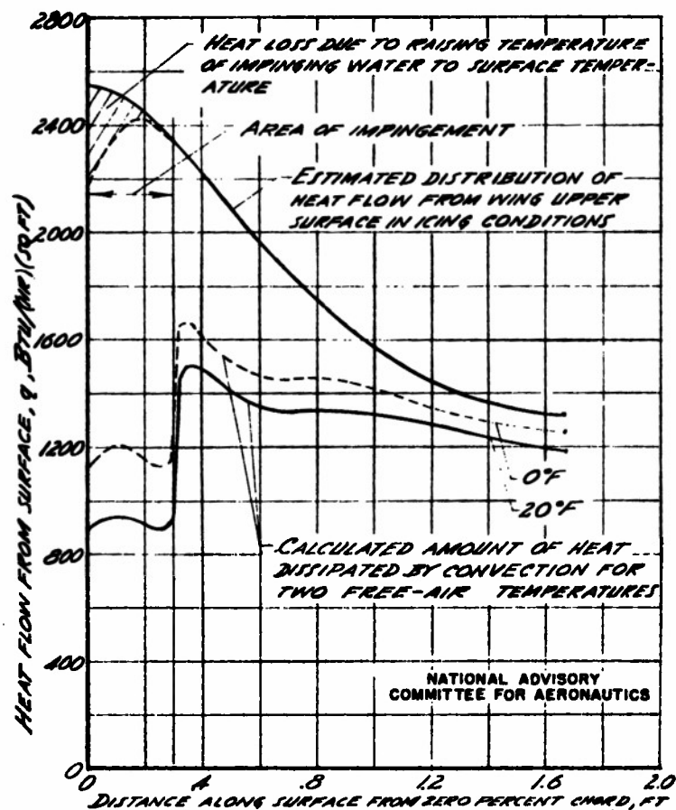
FIGURE 28.-ESTIMATED HEAT FLOW FROM UPPER SURFACE OF C-45 HEATED WING LEADING EDGE AT STATION 157 IN ICING CONDITIONS, AND CALCULATED CONVECTIVE HEAT LOSS, USED IN DETERMINATION OF RATE OF EVAPORATION OF WATER. PRESSURE ALTITUDE, 8,000 FT.; TRUE AIRSPEED, 180 MPH.
