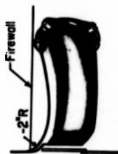
Original duct for shutter exit
