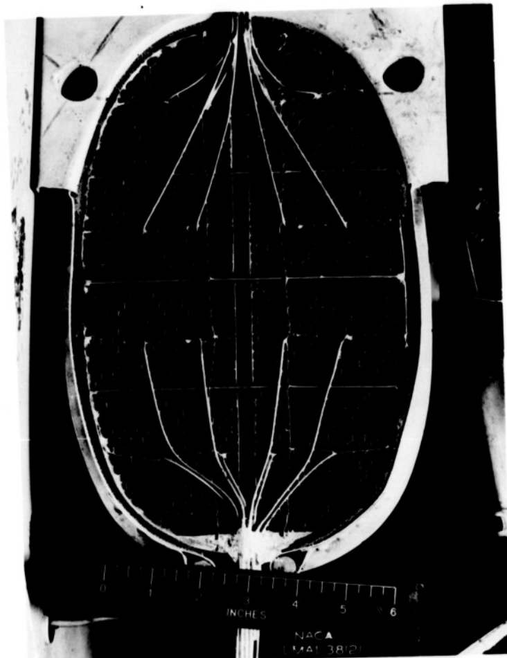
Figure 11.- View of rear face of oil cooler.
