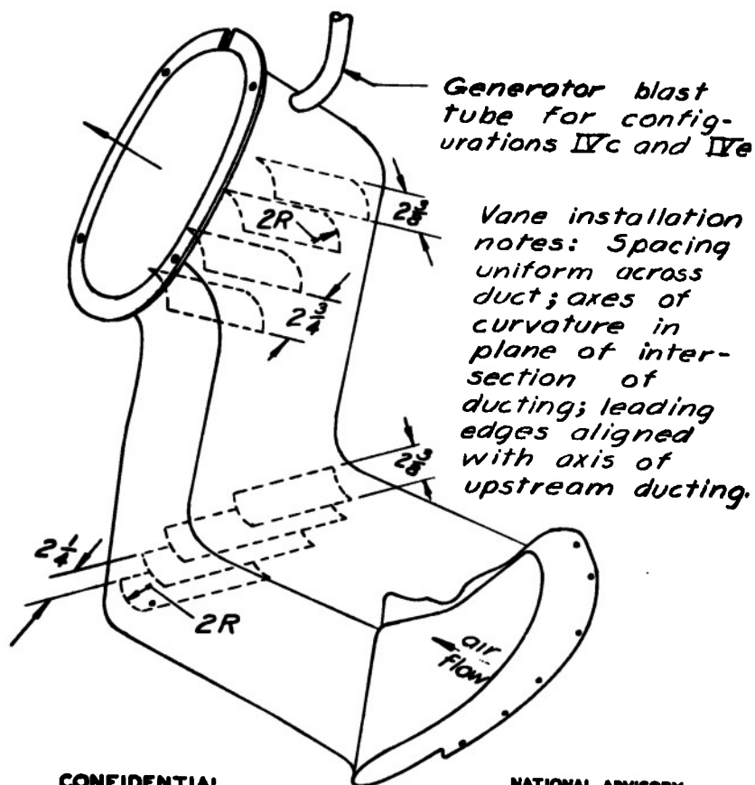
Figure 13. - Oil-cooler-inlet duct showing vanes and generator-blast-tube inlet.
