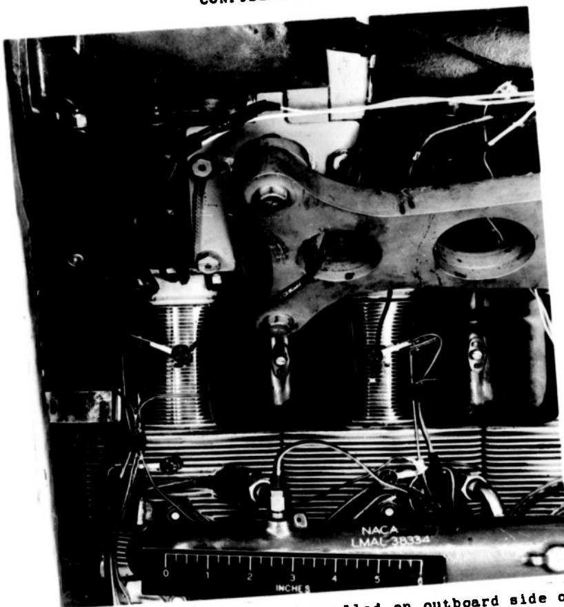
Figure 6.- Baffle installations.
