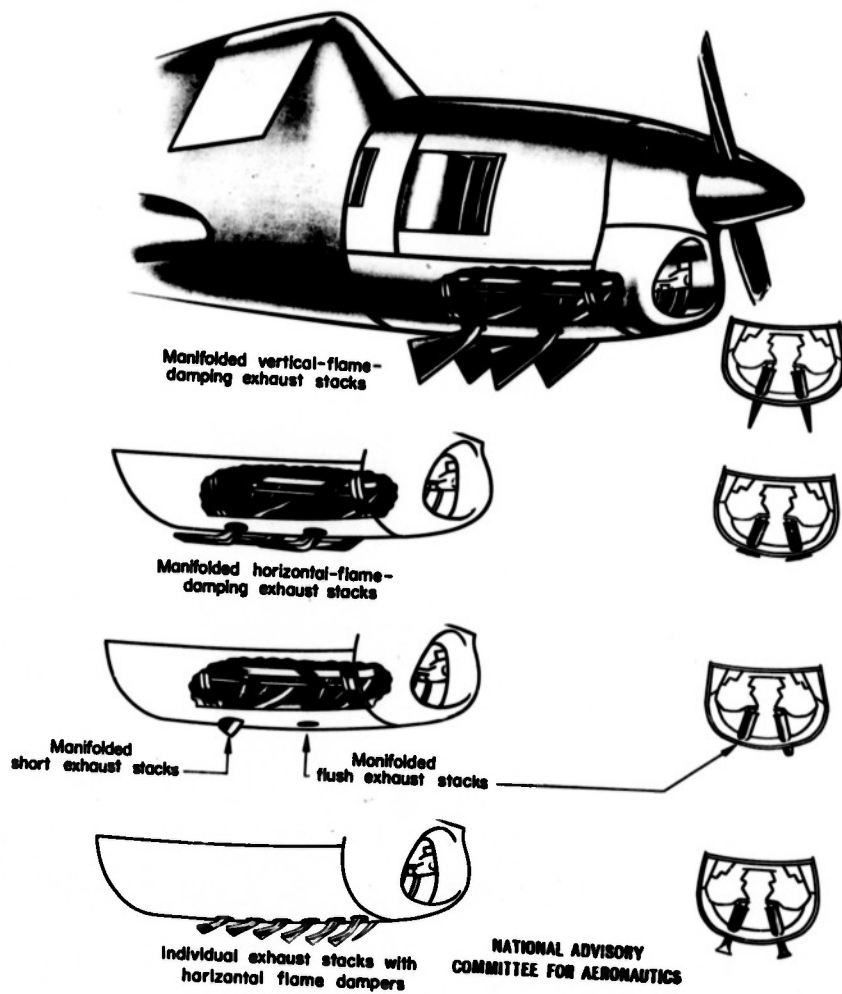
FIGURE 7.- EXHAUST STACK CONFIGURATIONS
