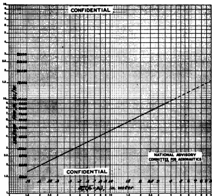
Figure 26.- Ground-stand calibration of leakage through cowl seams downstream of engine and from gap between cowl and firewall. Cowl flaps flush, taking strip removed from accessory compartment exit.
