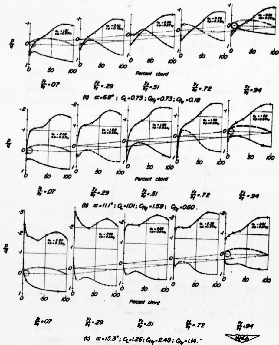
Figure 4.—Pressure distribution over a leading-edge flap for several angles of attack, R = 5,120,000 .
