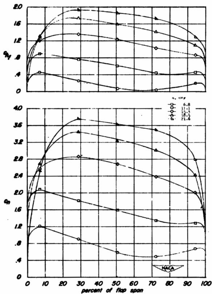
Figure 3.- Variation of flap normal-force coefficient and flap moment coefficient with angle of attack.
