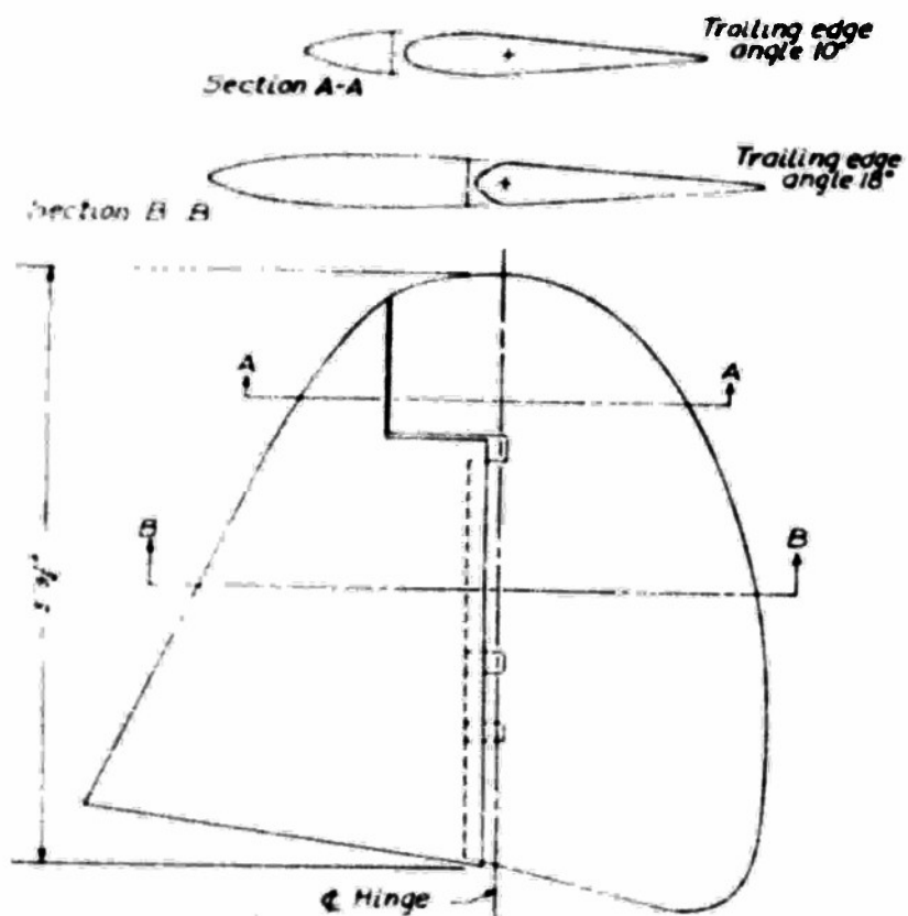
Figure 4.- Flap configuration number one. Brewster B2A-1 airplane.
