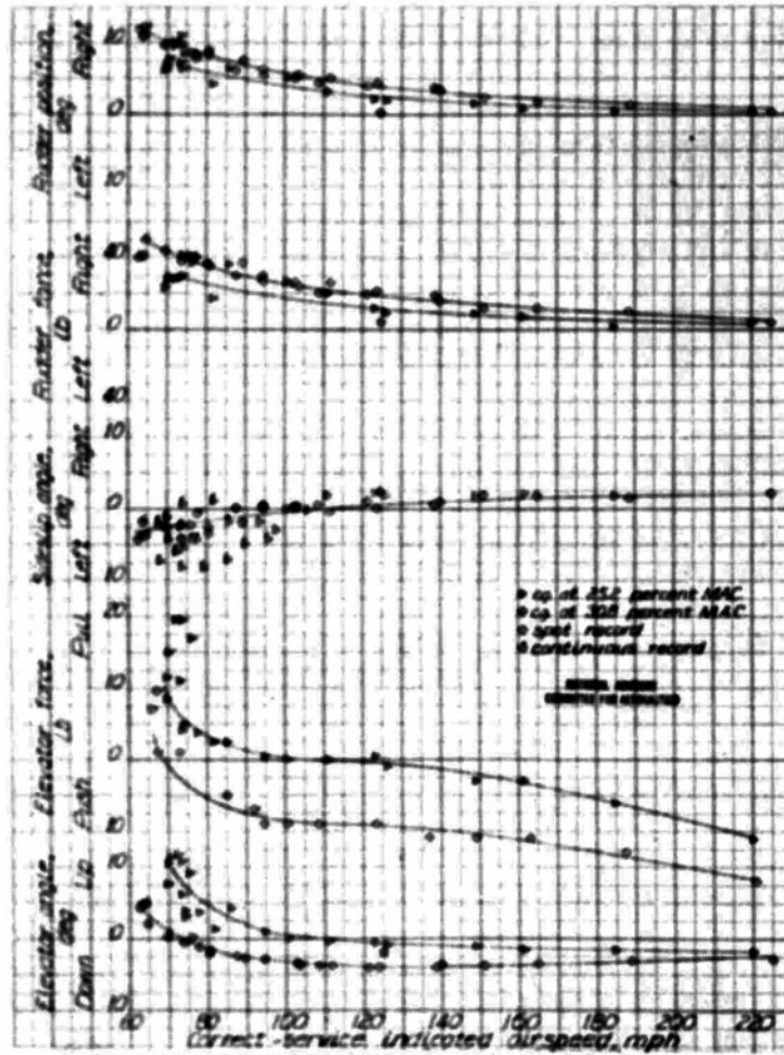
Figure 1. Data simplified statistics characteristic of the trial airplane with tail configuration 9 in the steady condition.
