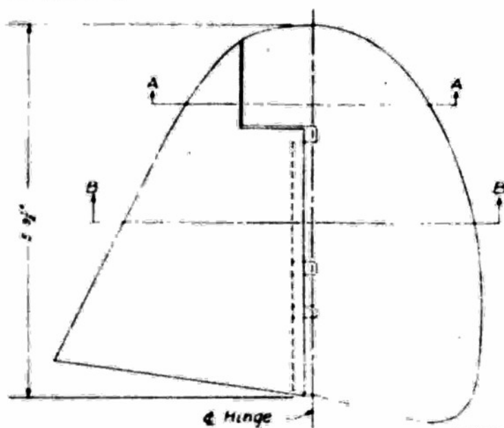
Figure 4.- Vertical tail configuration under way. Brewster BNA-1 airplane.
