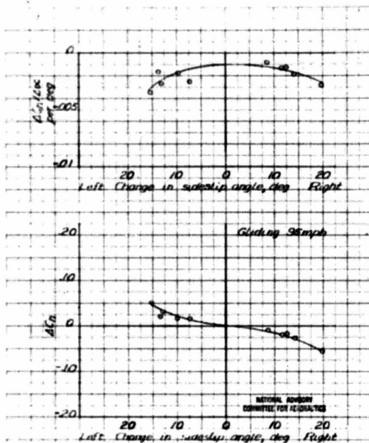
Figure 55.- Plots of \Delta C_{l, \text{ per deg}} and \Delta C_{D, \text{ per deg}} against change of sideslip angle during rudder kicks; XSA-1 airplane with tail configuration 2.
