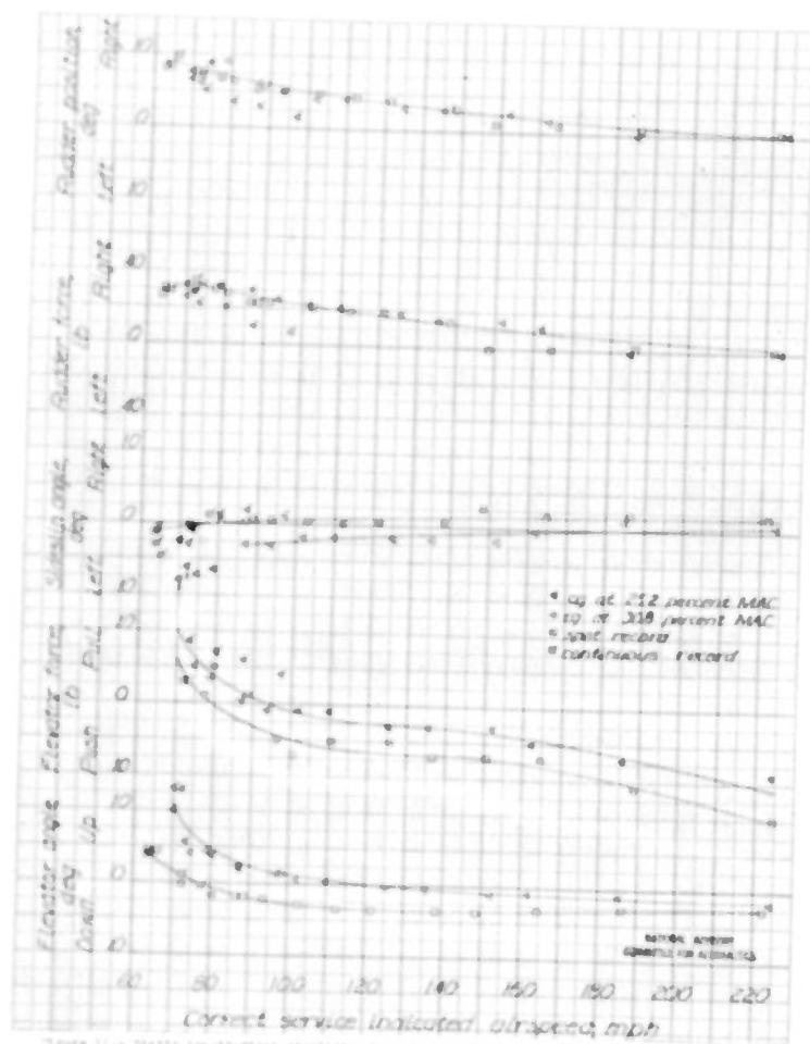
Figure 11. Static longitudinal stability characteristics of the F-4 Phantom II aircraft with full multi-spanning 1 to 100 percent control.
