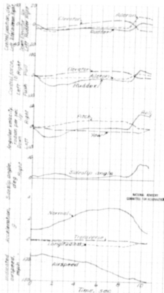
Figure 21. Time history of an abrupt left turn at 2 1/4 rolls per hour. Elevator 100A-1 airplane with tail configuration 3; rad. at 50,000 feet, 10,000 ft.
