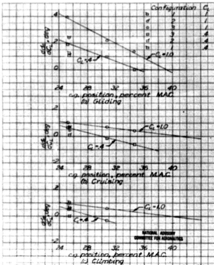
Figure 21. Plots showing stick-fixed neutral points in various flight conditions for the XRB-1 airplane.
