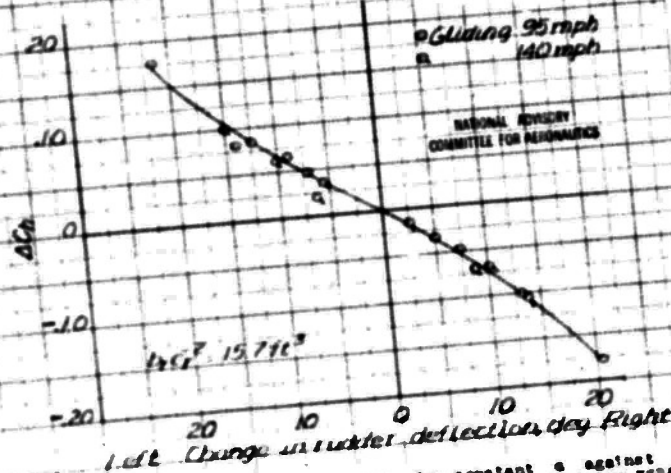
Figure 3.- Plots of aC_n/\delta\delta and \Delta C_n for constant \alpha against change of rudder deflection during rudder kicks; XPA-1 airplane with tail configuration 5.
