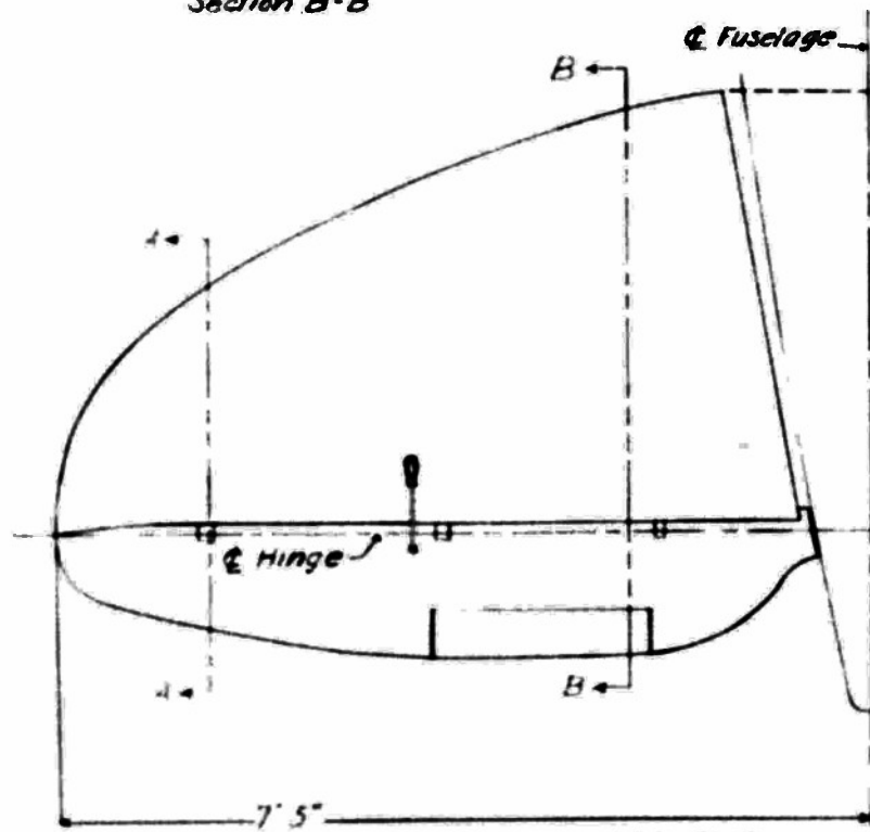
Figure 7.- Horizontal tail configuration of Brewster B2A-1 airplane.
