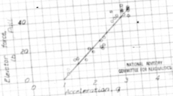
Figure 30.- Variation of elevator control force with normal acceleration, and variation of elevator position with lift coefficient in turns; Brewster XNNA-1 airplane with tail configuration 51 a.g. at 25.2 percent W.L.C.
