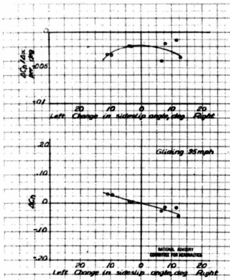
Figure 56.- Plots of \Delta C_n / \Delta \alpha and \Delta C_n against change of sideslip angle during rudder kicks; XRA-1 airplane with tail configuration 3.
