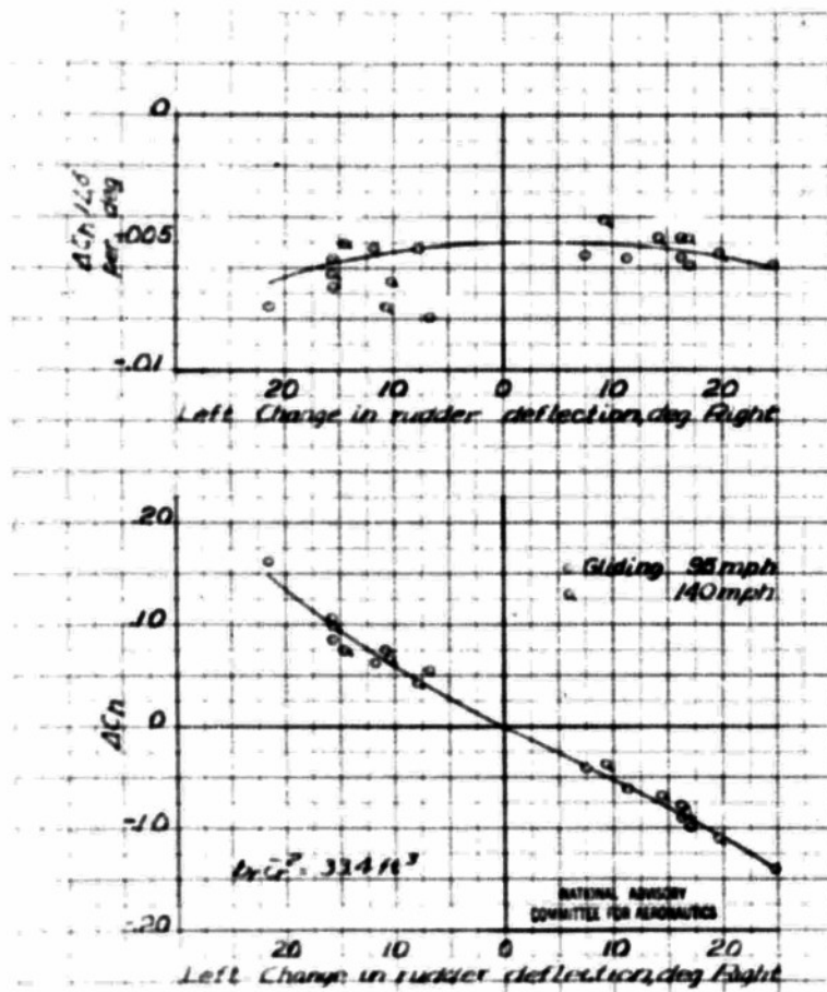
Figure 55.- Plots of \Delta C_n / \Delta \delta and \Delta C_n for constant \alpha against change of rudder deflection during rudder kicks; XSB-1 airplane with tail configuration 2.
