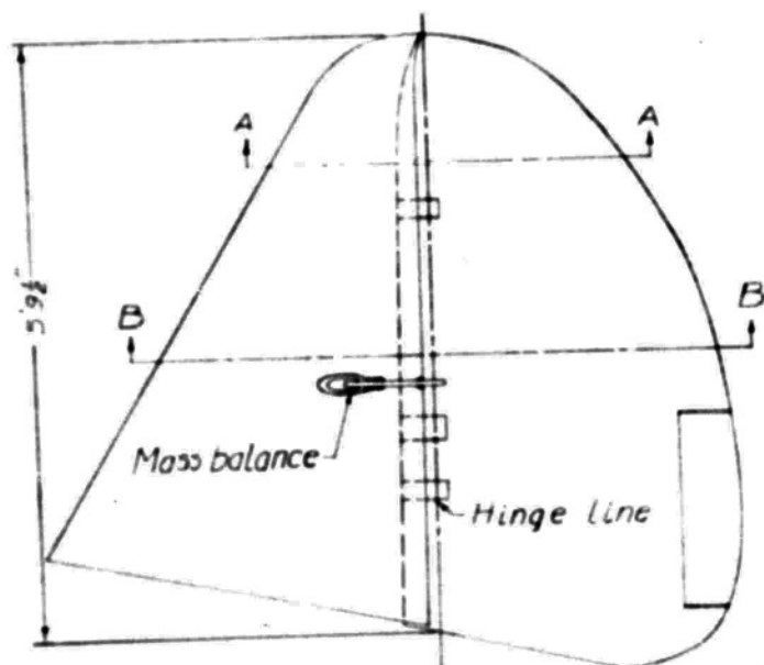
Figure 6.- Vertical foil configuration number ten. Brewster BSB-1 airplane.
