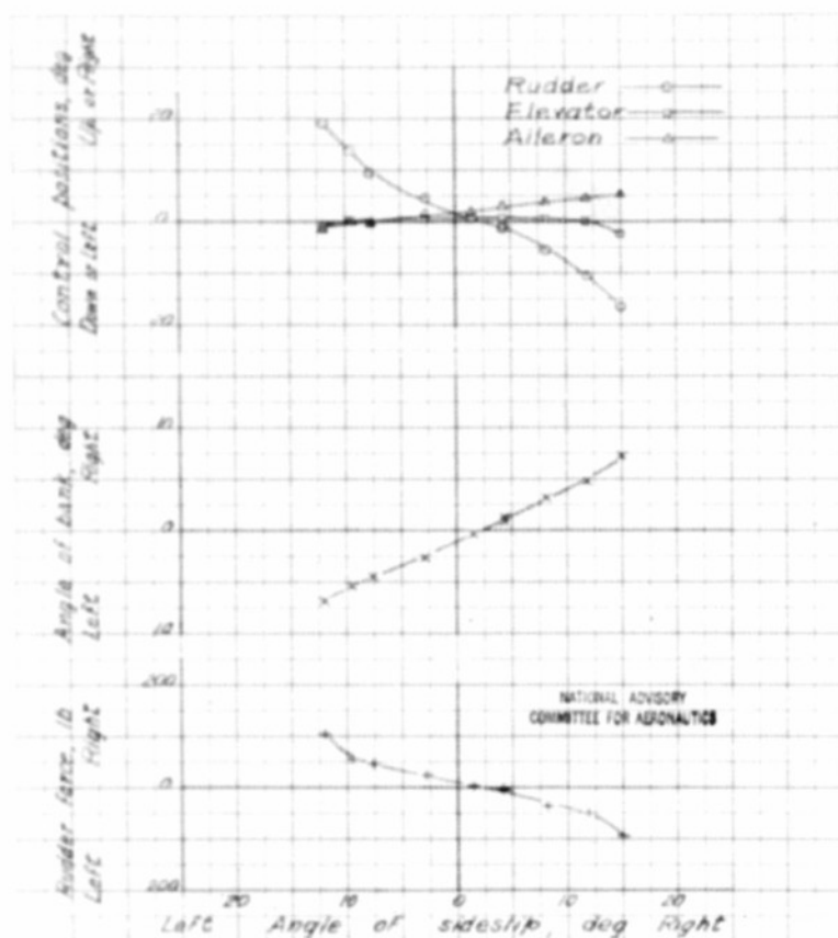
Figure 44.- Steady sideslip characteristics in the landing condition at 112 miles per hour (flaps down, landing gear down, power off); Brewster BSA-1 airplane with tail configuration 3.
