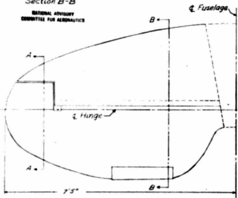
Figure 1.- Horizontal tail configuration number one. Brewster XB3A-1 airplane.
