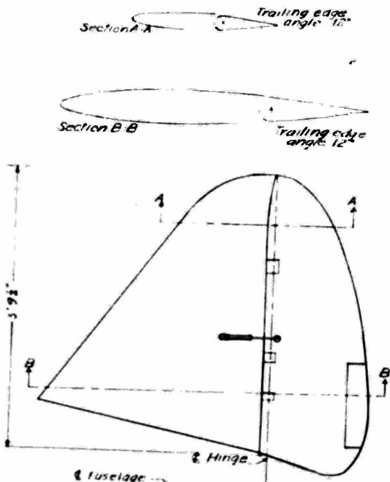
Figure 2.- Vertical tail configuration of biplane ANS-1 airplane.
