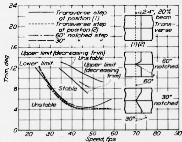
Figure 10.- Effect of position and plan form of step on trim limits of stability. Model 6, 1/5 full-size. \Delta_0 , 63.4 lb; C_{D0} , 1.01.
