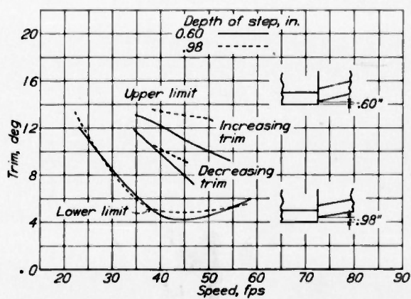
Figure 7.- Effect of depth of step on trim limits of stability. Model 6, 1/5 full-size. \Delta_0 , 63.4 lb; C_{A_0} , 1.01.
