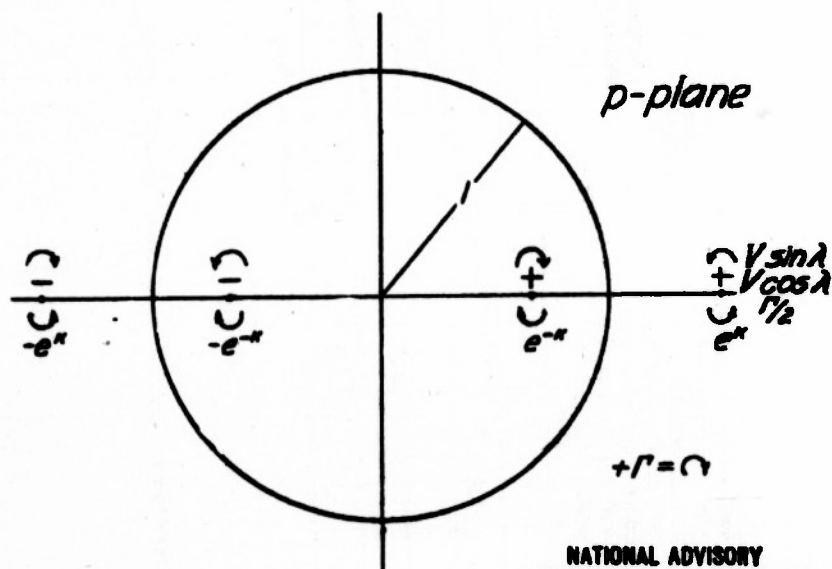
Figure 3.—Source-vortex system for cascade flow.
