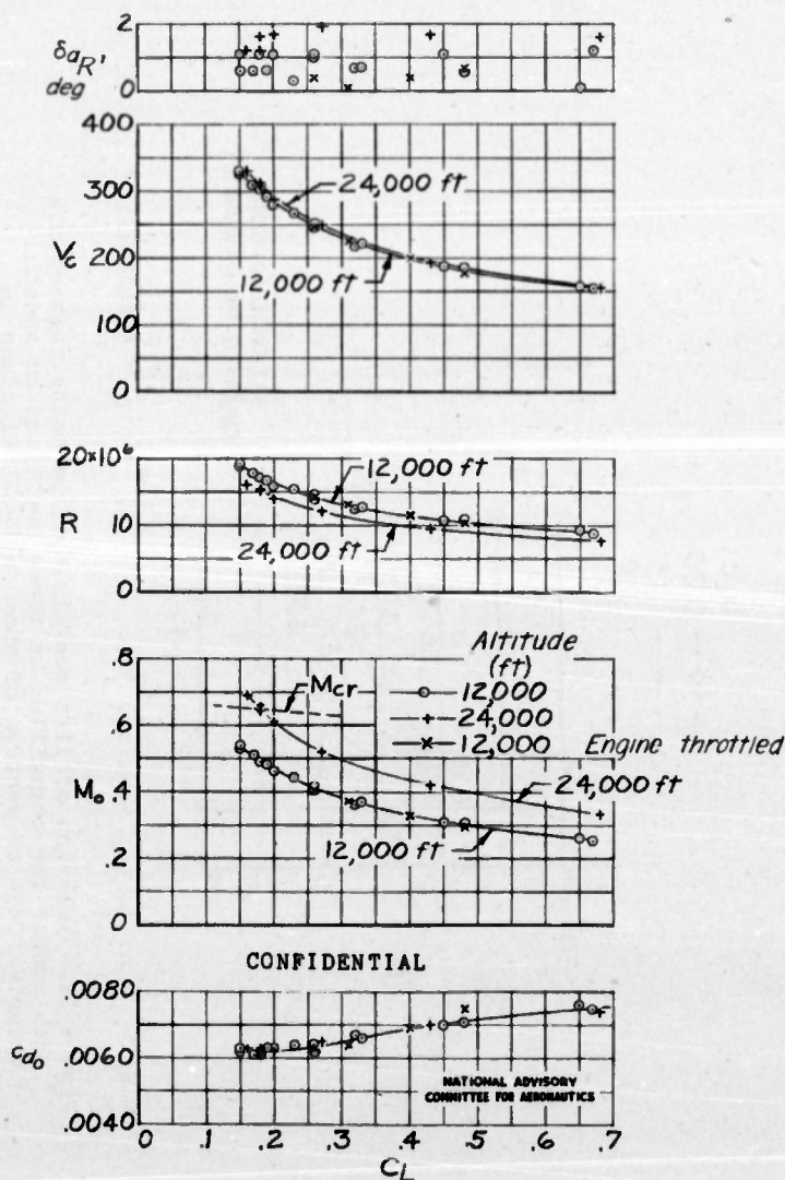
Figure 12.- Profile-drag coefficient of smooth section on right wing of F-47D airplane as obtained in straight flight. Mach number, Reynolds number, calibrated airspeed, and deflection of right aileron are plotted above c_{d_o} -curve. M_{cr} -curve is from results of left-wing tests.
