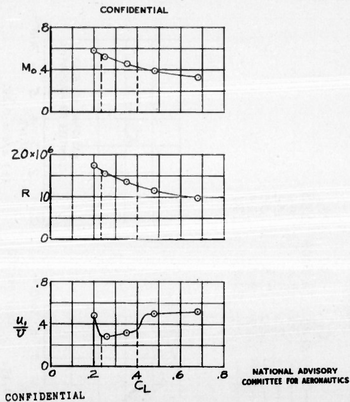
Figure 9.- Method of determining lift coefficient, Reynolds number, and Mach number corresponding to transition at a given chord-wise position. (Example shown is for 15 percent chord. Effective-pressure center of total-pressure tube at 0.01 in. above surface.)
