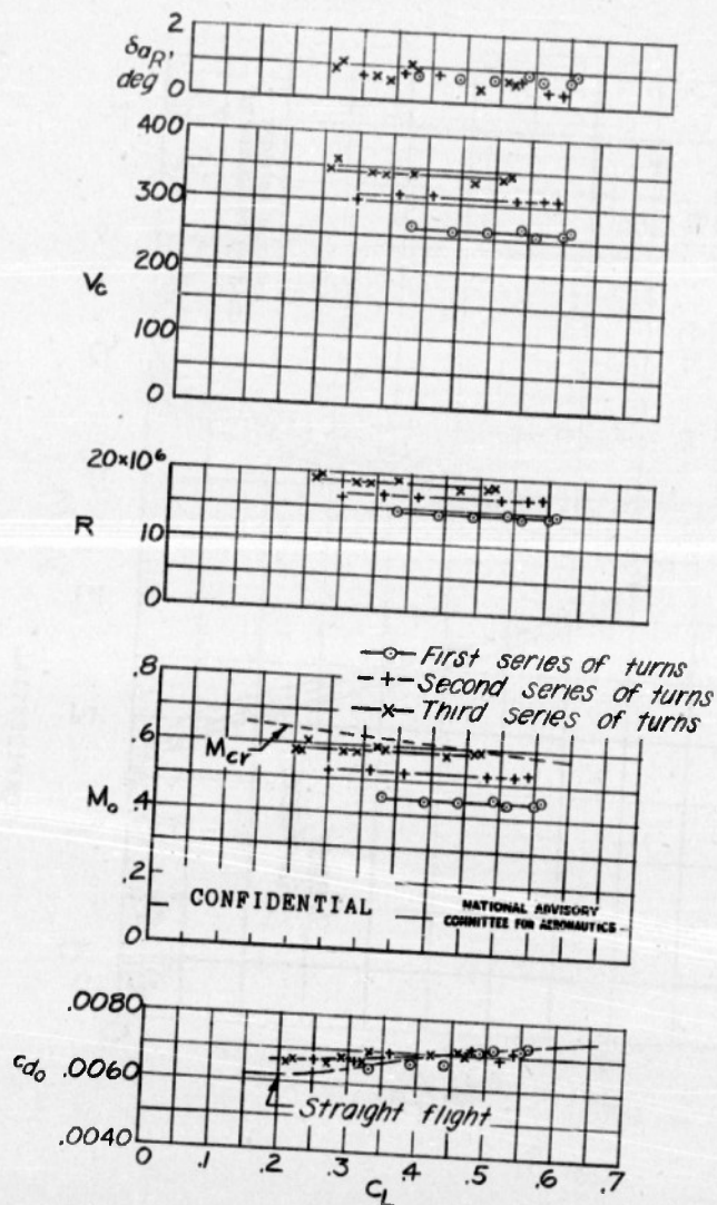
Figure 13.- Profile-drag coefficient of smooth section of right wing on P-47D airplane as obtained in turns. Mach number, Reynolds number, calibrated airspeed, and deflection of right aileron are plotted above c_{d0} -curves. M_{CR} -curve is from results of left-wing tests.
