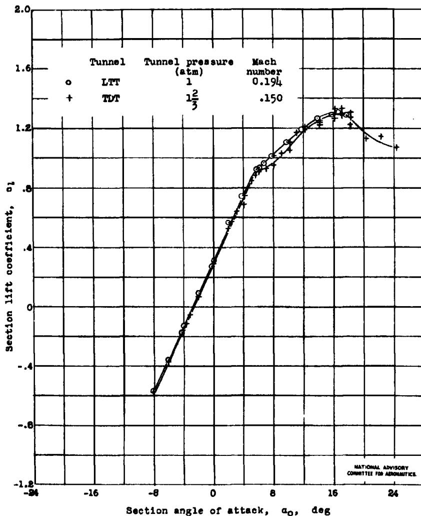
Figure 1.- Lift characteristics of 24-inch-chord model of NACA 653-418, a = 1.0 airfoil section in NACA two-dimensional low-turbulence tunnel (designated LTT) and NACA two-dimensional low-turbulence pressure tunnel (designated TDT). R = 2.77 \times 10^6 .
