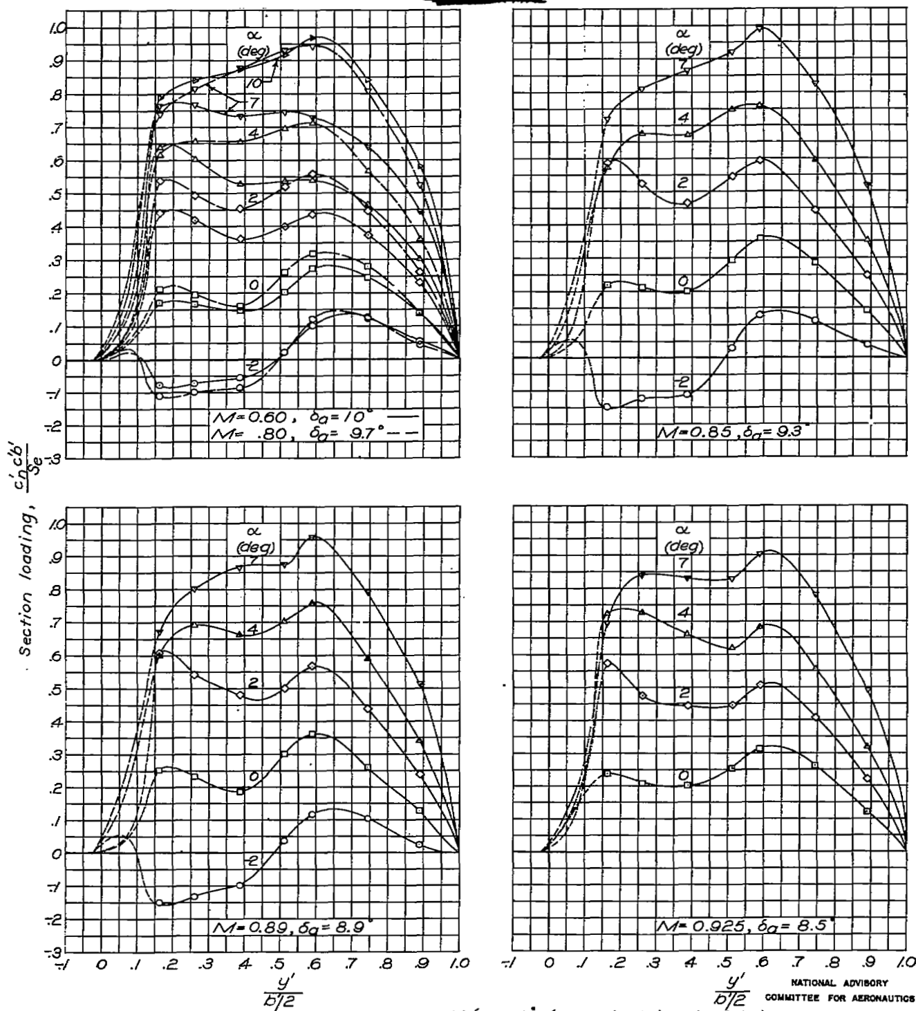
Figure 15. — Concluded. \Lambda_r = -30^\circ
