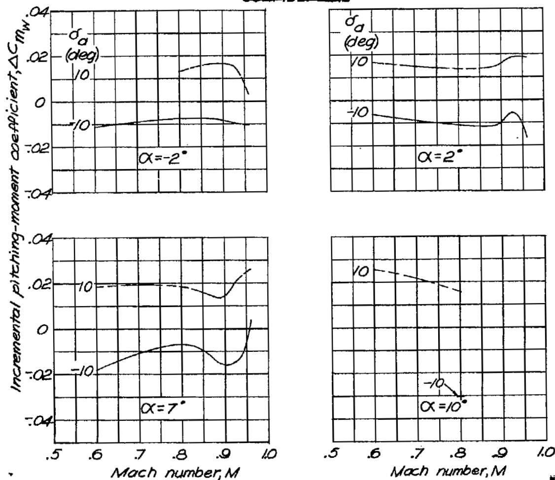
Figure 19.—Variation of change in wing pitching-moment coefficient resulting from aileron deflection with Mach number.
