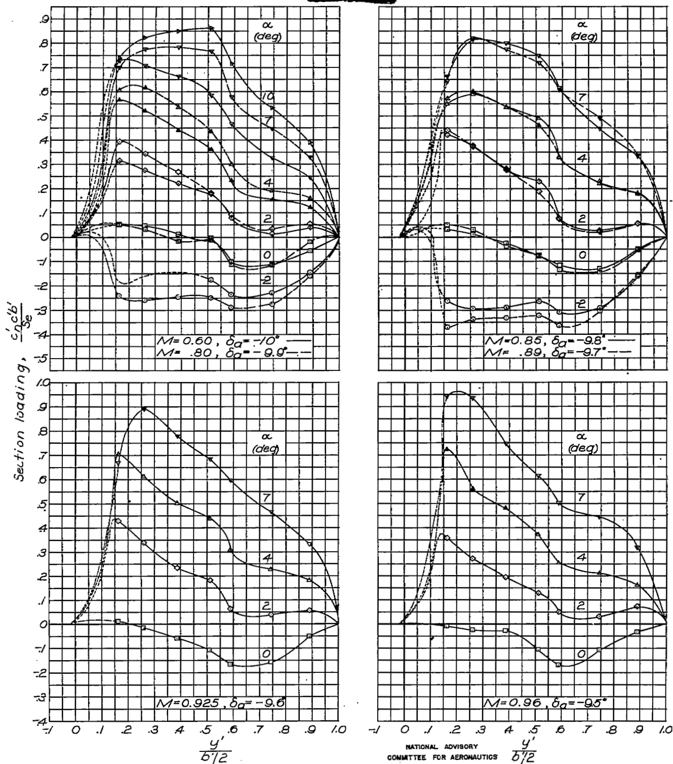
Figure 15. — Spanwise variation in section loading along Y-axis. \alpha_r \approx -10^\circ . (Note individual plots.) \alpha_r \approx -30^\circ .
