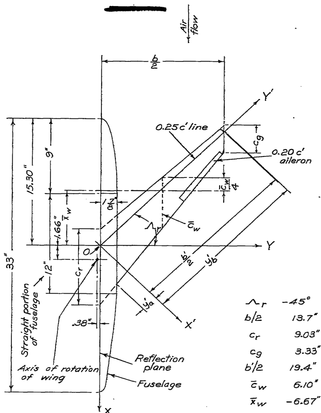
Figure 1.—Plan form and general dimensions of model wing-fuselage configuration with 45^\circ sweepforward.
