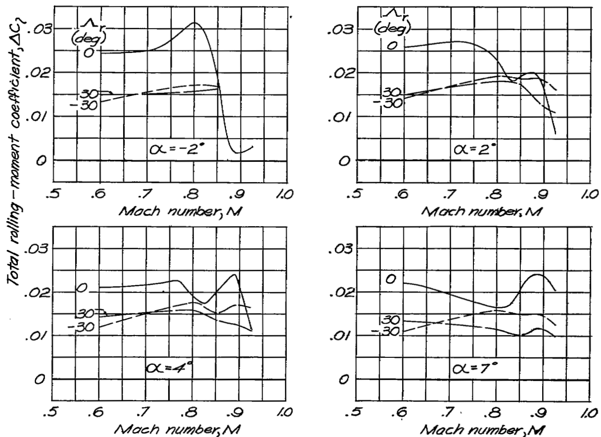
Figure 8.—Variation of total rolling-moment coefficient with Mach number. Wing with ailerons at equal positive and negative deflections. Data for \delta_r = 0^\circ from reference 3.
