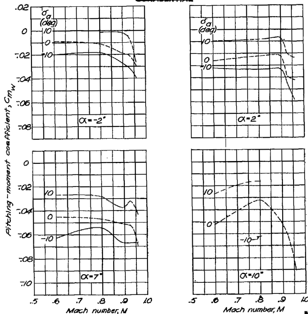
Figures 18. - Variation of wing pitching-moment coefficient with Mach number. Data for \delta_a = 0 from reference 1.
