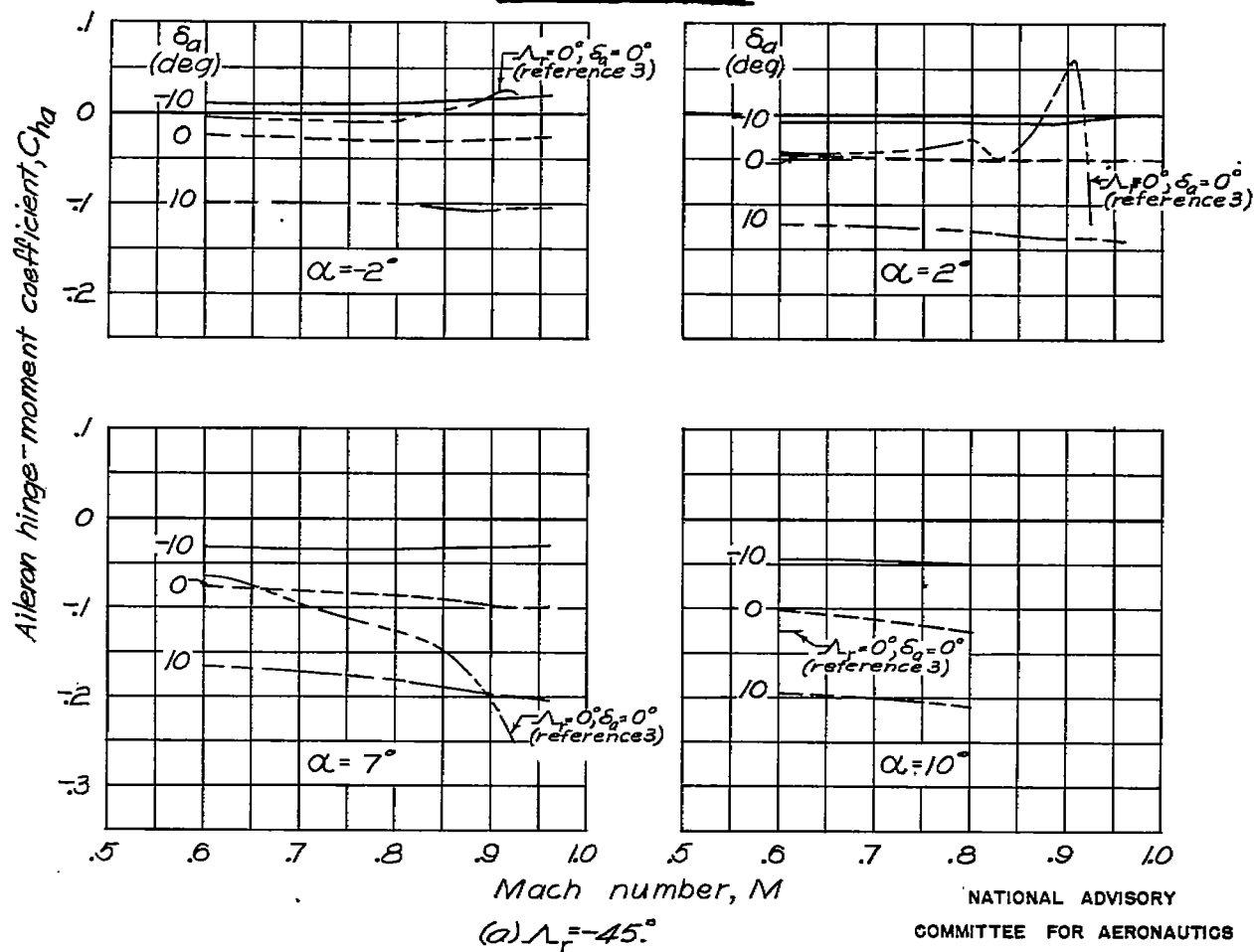
Figure 9.—Variation of aileron hinge-moment coefficient with Mach number. Unsealed aileron. Data for \Lambda_r = 0^\circ, \delta_a = 0^\circ from reference 3.
