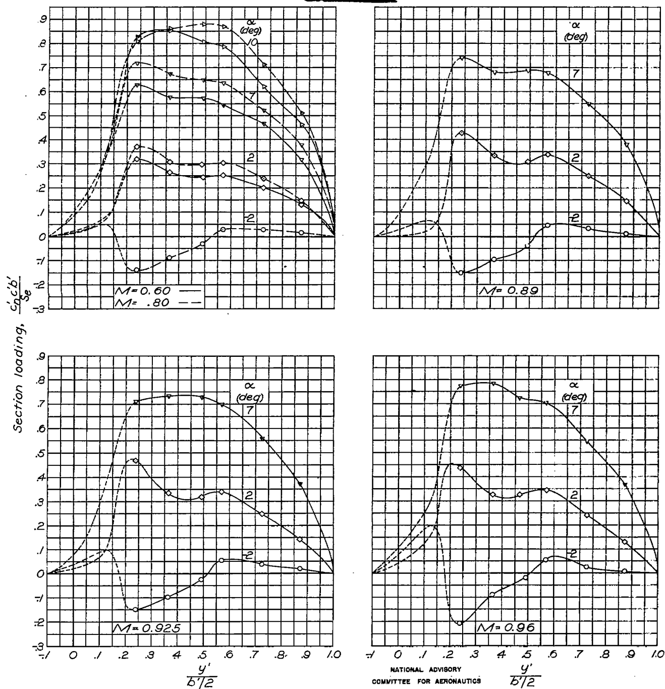
Figure 14. — Concluded. \Lambda_r = -45^\circ . (c) \delta_0 = 9.8^\circ .
