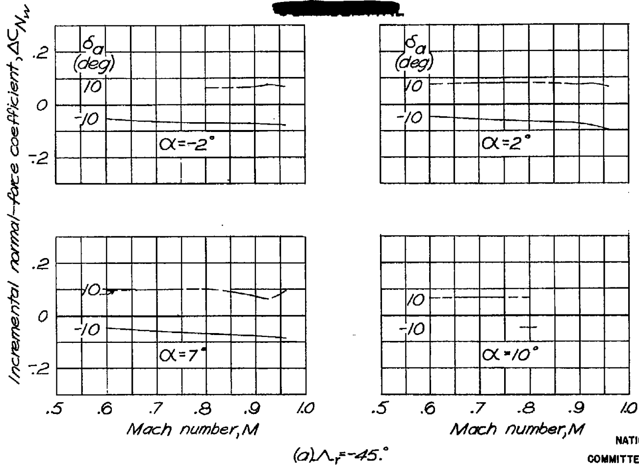
Figure 13.—Variation of change in wing normal-force coefficient resulting from aileron deflection with Mach number.
