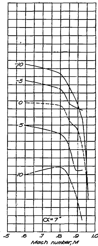
(c) \Lambda_r = 30^\circ Figure 18. -Continued.
