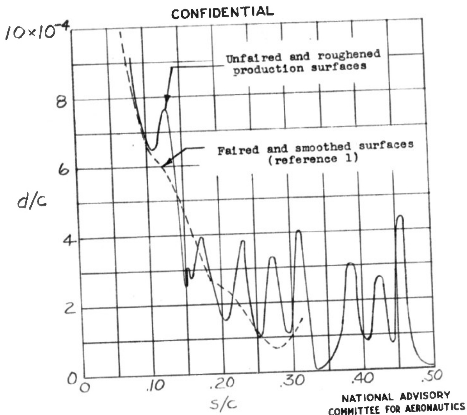
Figure 4.- Surface-waviness index of unfaired and roughened production surfaces and of faired and smoothed surfaces.
