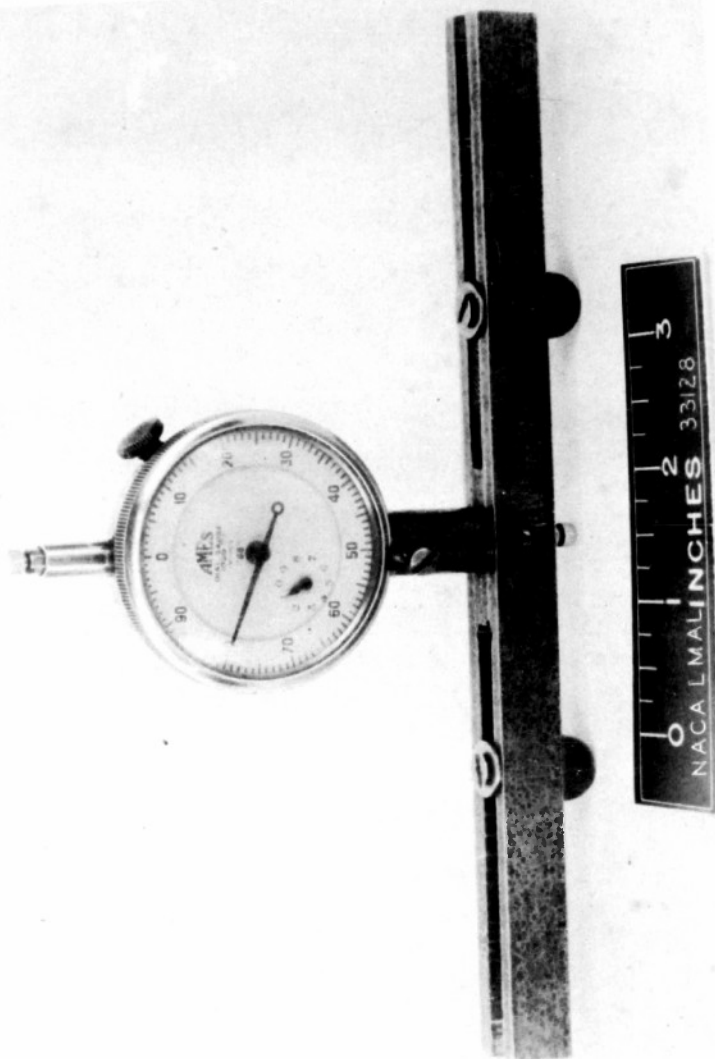
Figure 2.- Curvature gage used in measuring surface waviness.
