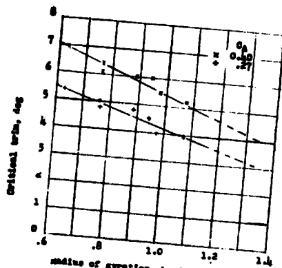
Figure 4.- Variation of critical trim with change in radius of gyration. C_v = 6.0 ; l_1 = 0.38b ; l_2 = 1.26b .
