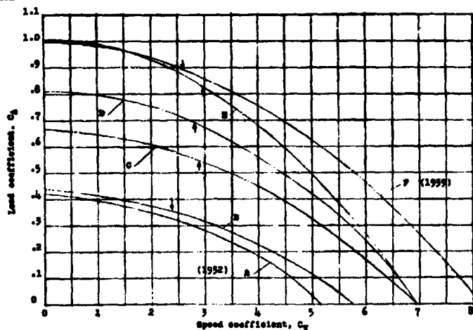
Figure 9.- Comparison of the load coefficient on the water of several flying boats during take-off, assuming the value of C_v to be constant and equal to C_v at get-away.
