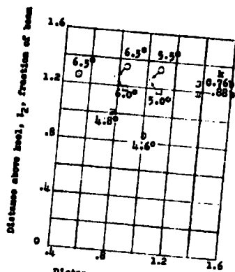
Figure 5.- Variation of critical trim with change in the location of the pivot. C_b = 0.40 ; C_v = 5.0 .
