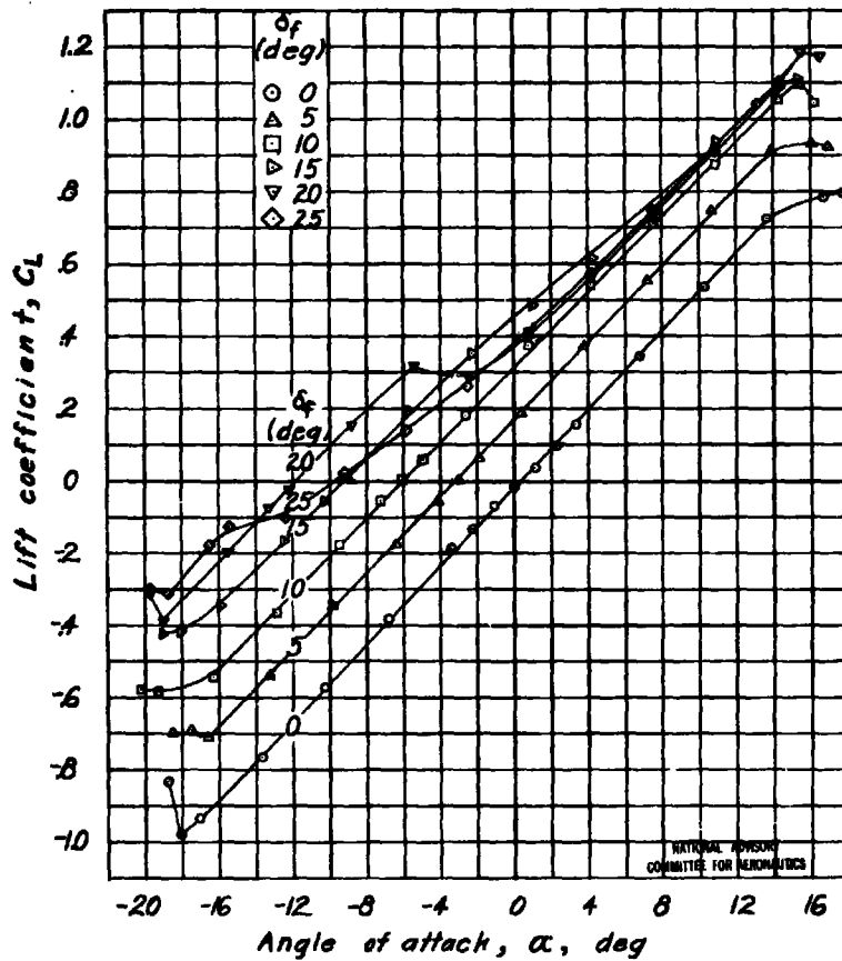
Figure 9.- Aerodynamic characteristics of a rectangular semispan tail surface. Flap with 0.50c blunt overhang; sealed gap; \delta_e = 0^\circ ; 0.30c flap; A=3 .
