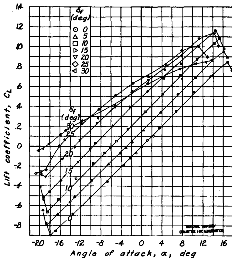
Figure 12.- Aerodynamic characteristics of a rectangular semispan tail surface. Flap with 0.50c_f elliptical overhang; 0.005c gap; \delta_t = 0^\circ ; 0.30c flap; A=3 .
