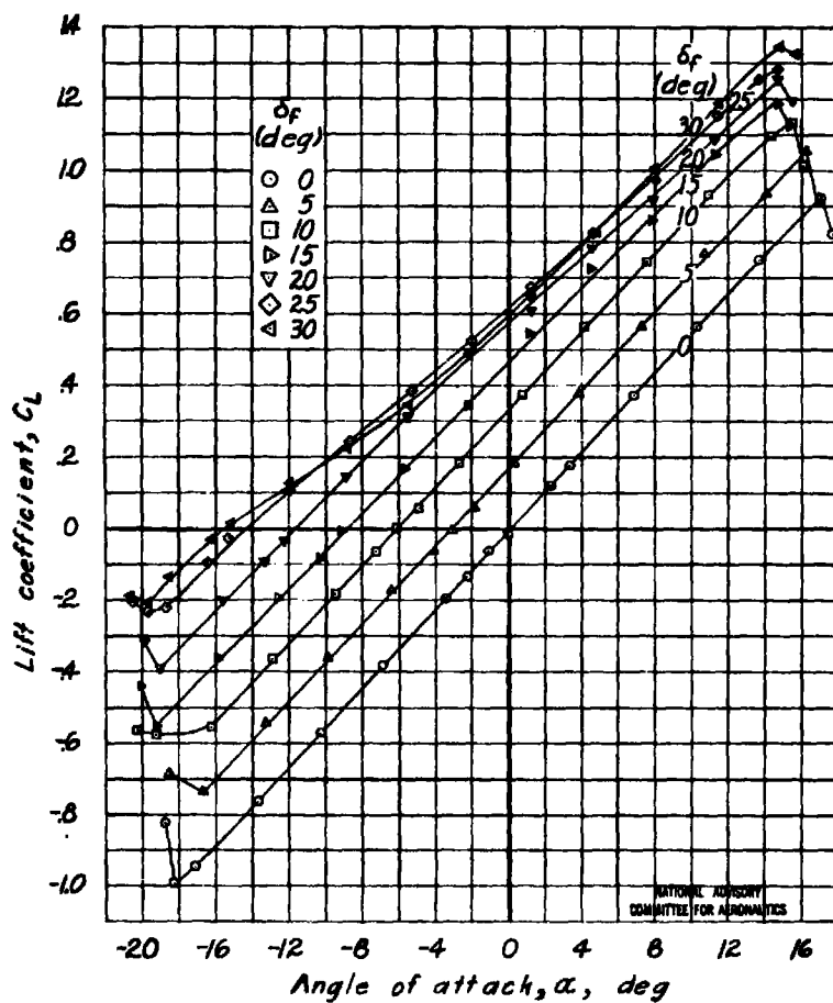
Figure 7.-Aerodynamic characteristics of a rectangular semispan tail surface. Flap with 0.35c_f elliptical overhang; sealed gap; \delta_e = 0^\circ ; 0.30c flap; A=3 .
