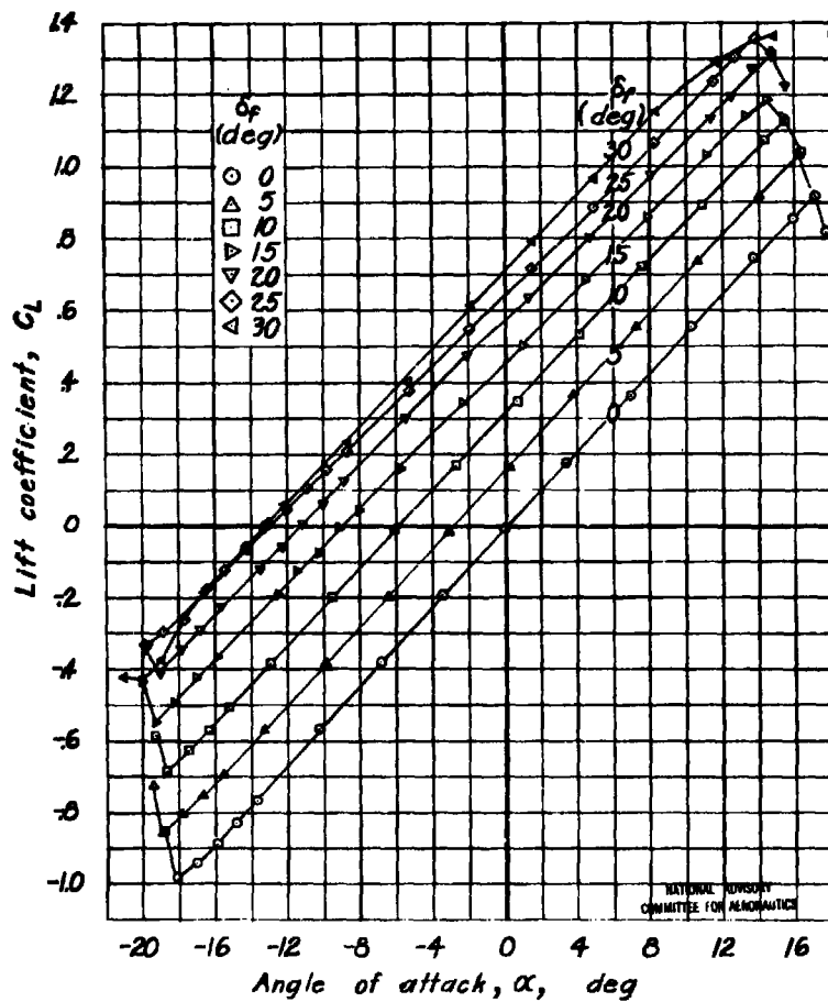
Figure 4.- Aerodynamic characteristics of a rectangular semispan tail surface. Plain flap; 0.005c gap; \delta_t = 0^\circ ; 0.30c flap; \Lambda = 3 .
