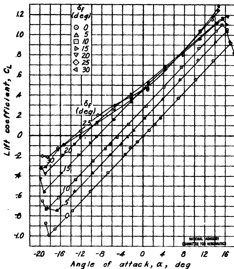
Figure 11.- Aerodynamic characteristics of a rectangular semispan tail surface. Flap with 0.50c_f elliptical overhang; sealed gap; \delta_t = 0 ; 0.30c flap; A=3 .
