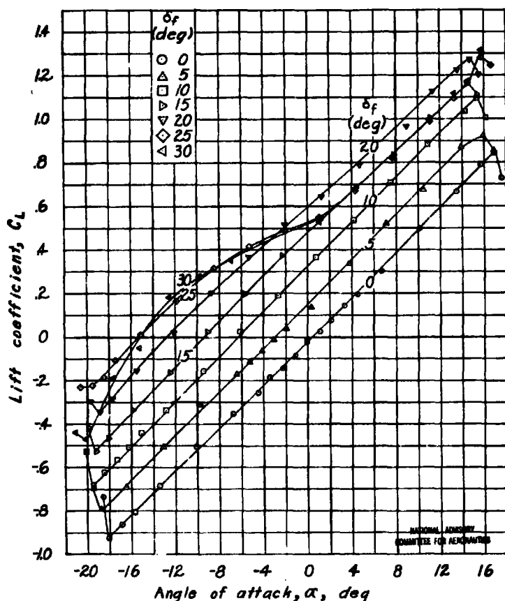
Figure 6.- Aerodynamic characteristics of a rectangular semispan tail surface. Flap with 0.35c_f blunt overhang; 0.005c gap; \delta_c = 0 ; 0.30c flap; A=3 .
