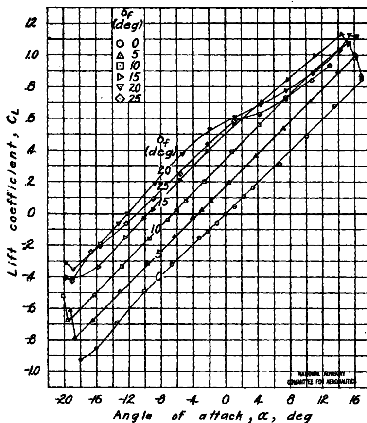
Figure 10.- Aerodynamic characteristics of a rectangular semispan tail surface. Flap with 0.50 c blunt overhang; 0.005 c gap; \delta_t = 0^\circ ; 0.30 c flap; \Lambda = 3 .
