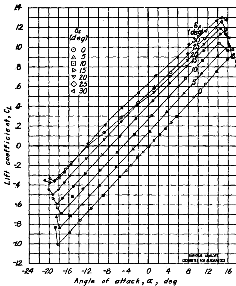
Figure 14.-Aerodynamic characteristics of a rectangular semispan tail surface. Plain flap; sealed gap; \partial \delta_c / \partial \delta_f = -1 ; 0.30c flap; A=3 .
