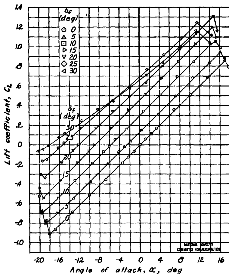
Figure 8.- Aerodynamic characteristics of a rectangular semispan tail surface. Flap with 0.35 c_f elliptical overhang; 0.005 c gap; \delta_t = 0^\circ ; 0.30 c flap; \Lambda = 3 .
