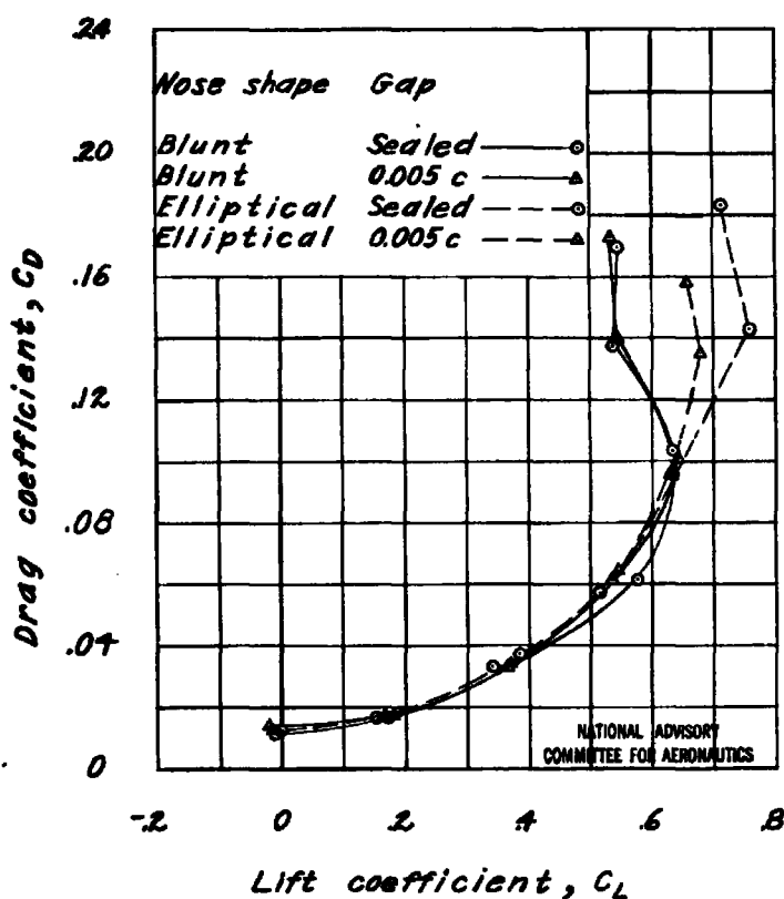
Figure 13.- Drag coefficient as a function of lift coefficient for a rectangular semispan tail surface with a 0.30c flap having a 0.35c overhang. \alpha = 0^\circ ; A = 3 .
