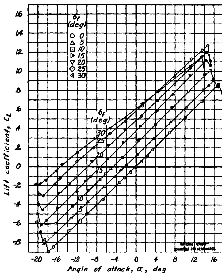
Figure 15.- Aerodynamic characteristics of a rectangular semispan tail surface. Flap with 0.35c_f elliptical overhang; 0.005c gap; \partial\delta_f/\partial\delta_f = -1 ; 0.30c flap; A=3 .
