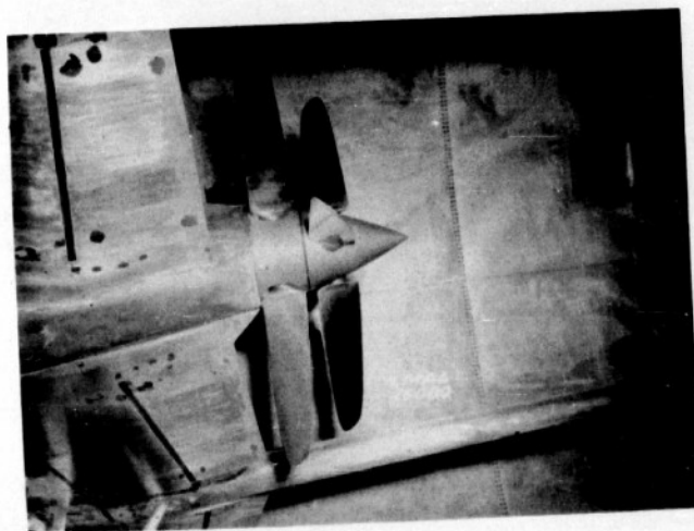
Figure 4.- Assembly of propeller 4-308-045 on model.
