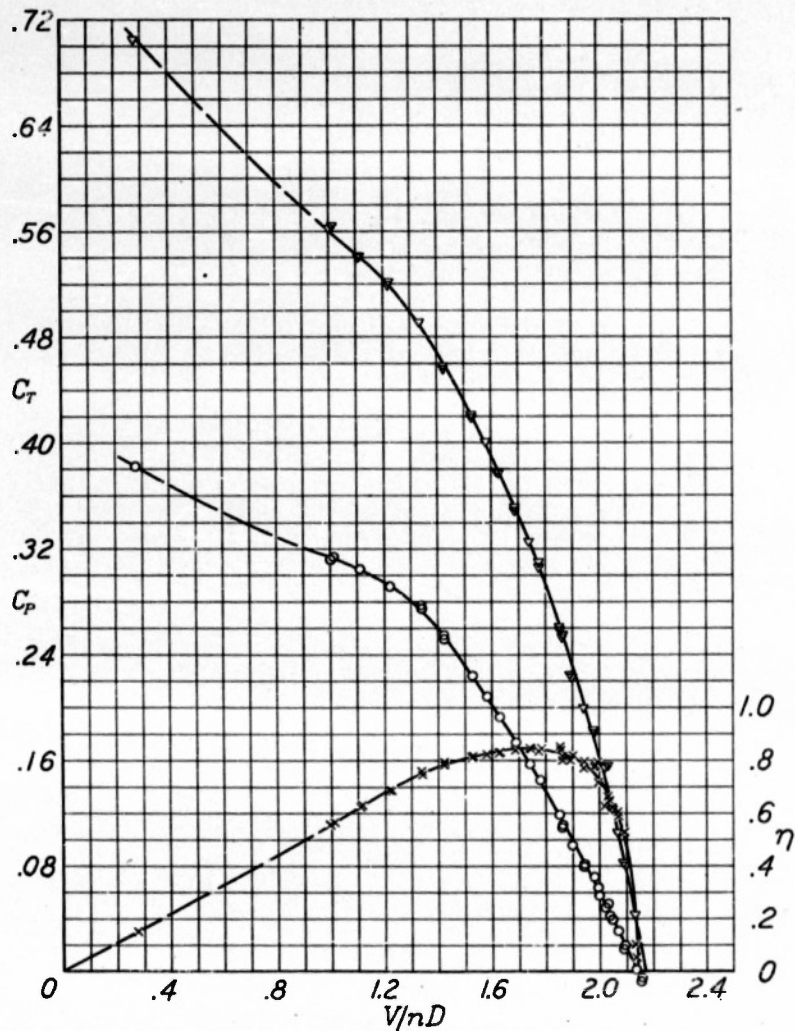
Figure 6.- Typical test results (propeller 512, \beta_P = 40.0^\circ and \beta_R = 40.4^\circ at 0.75R).
