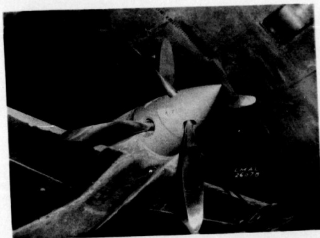
Figure 3.- Assembly of propeller 512 on model.
