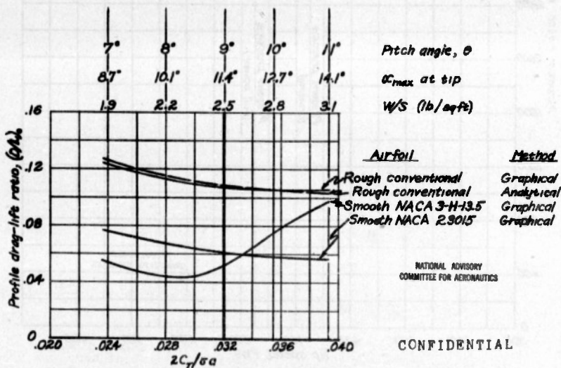
Figure 5.- Rotor profile drag-life ratio as affected by loading. Sample helicopter rotor; \mu=0.2 .
