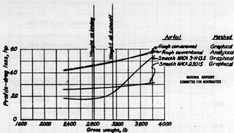
Figure 4.- Rotor profile-drag loss for a range of gross weights. Sample helicopter; \mu=0.2 .
