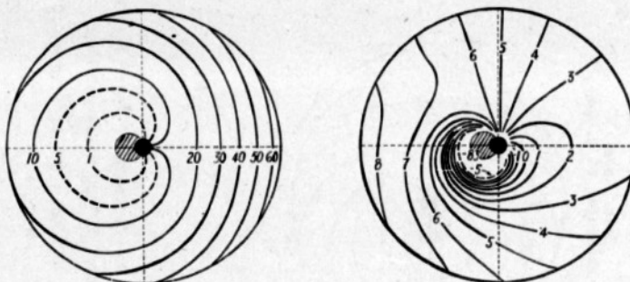
(b) Increased solidity; \lambda = -0.0350 ; \theta = 7^\circ ; \sigma = 0.10 ; \frac{2C_T}{\sigma a} = 0.0225 .
