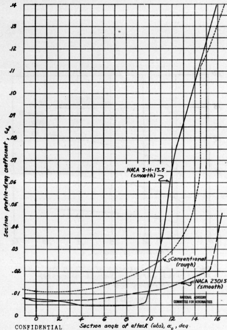
Figure 1.-Profile-drag curves used in the analysis.
