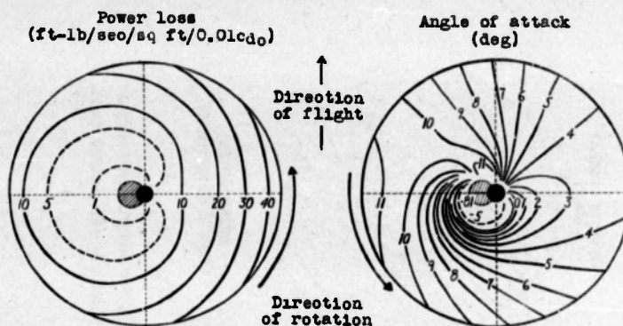
(a) Original solidity; \lambda = -0.0385 ; \theta = 9^\circ ; \sigma = 0.07 ; \frac{2C_T}{\sigma a} = 0.0321 .
