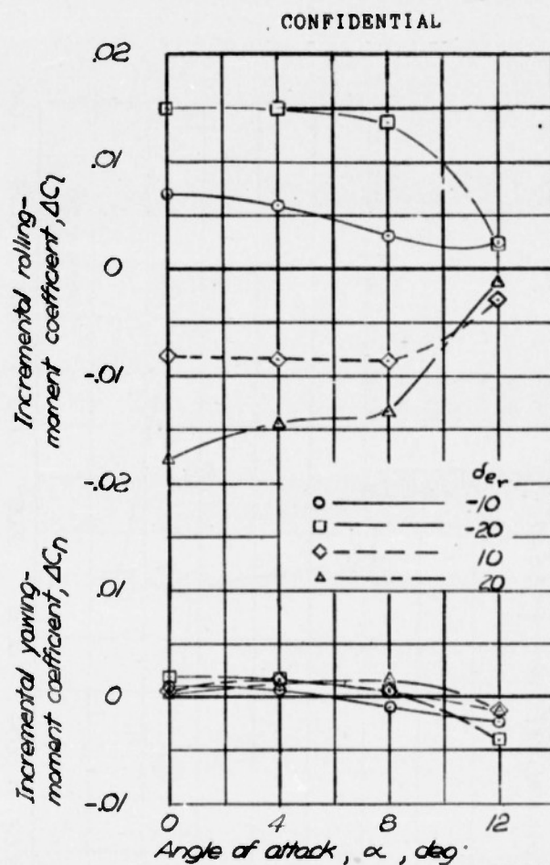
Figure 13.- Variation of elevator effectiveness with angle of attack for Langley free-flight-tunnel model of tailless all-wing airplane with sweepback.
