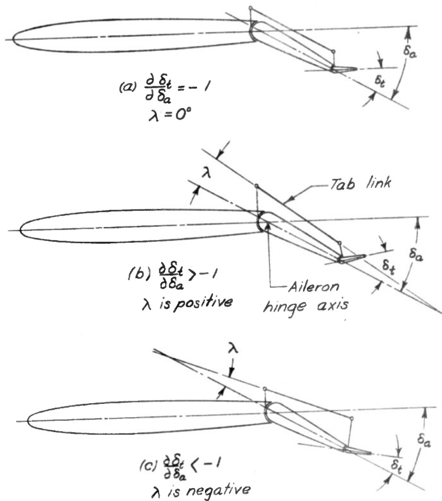
FIGURE 1.-Various balancing-tab linkage systems for ailerons.
