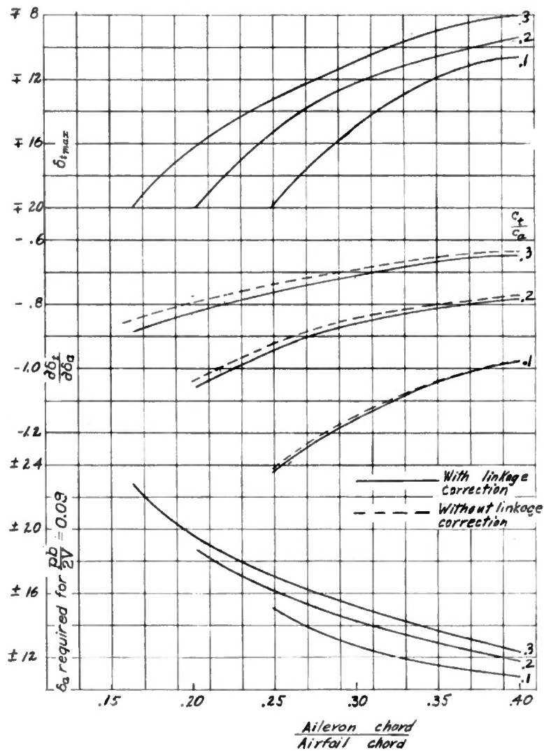
Figure 2. - Characteristics of ailerons with balancing tab deflected to give C_{h\delta_a'} = 0 when airplane is rolling; based on section data for NACA 0009 airfoil.
