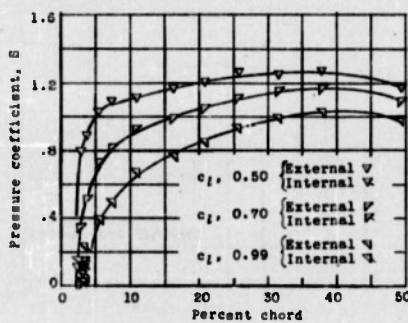
Figure 11.- Pressure distributions on the lower surface and lift characteristics of the wing inlet section with inlet 4, modified exit, and baffle plate in duct: h_p , 0.188 inches; R , 2.0 \times 10^6 ; test, LTT 380.
