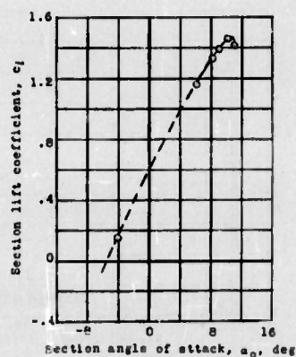
Figure 11.- Pressure distributions on the lower surface and lift characteristics of the wing inlet section with inlet 4, modified exit, and baffle plate in duct: h_p , 0.188 inches; R , 2.0 \times 10^6 ; test, LTT 380.
