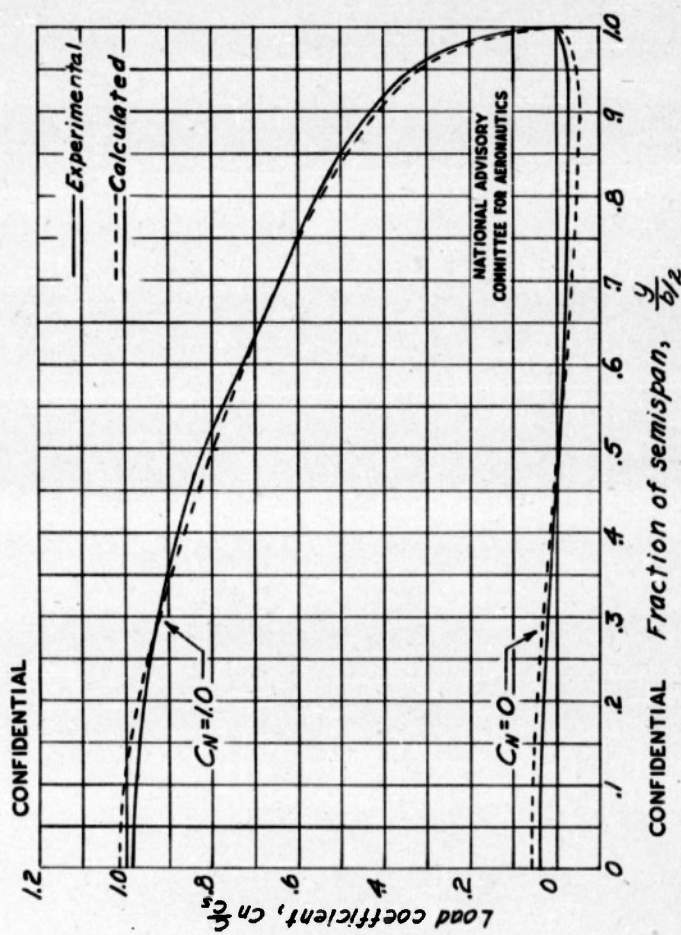
Figure 12. - Comparison of experimental and calculated load distribution curves for wing normal-force coefficients of 0 and 1.0 at M=0.40 .
