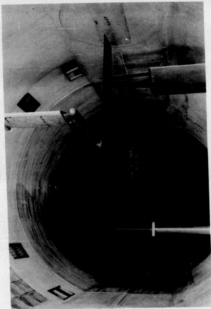
Figure 2.- Rear view of wing showing boom and strut assembly used to conduct pressure tubes to manometers.
