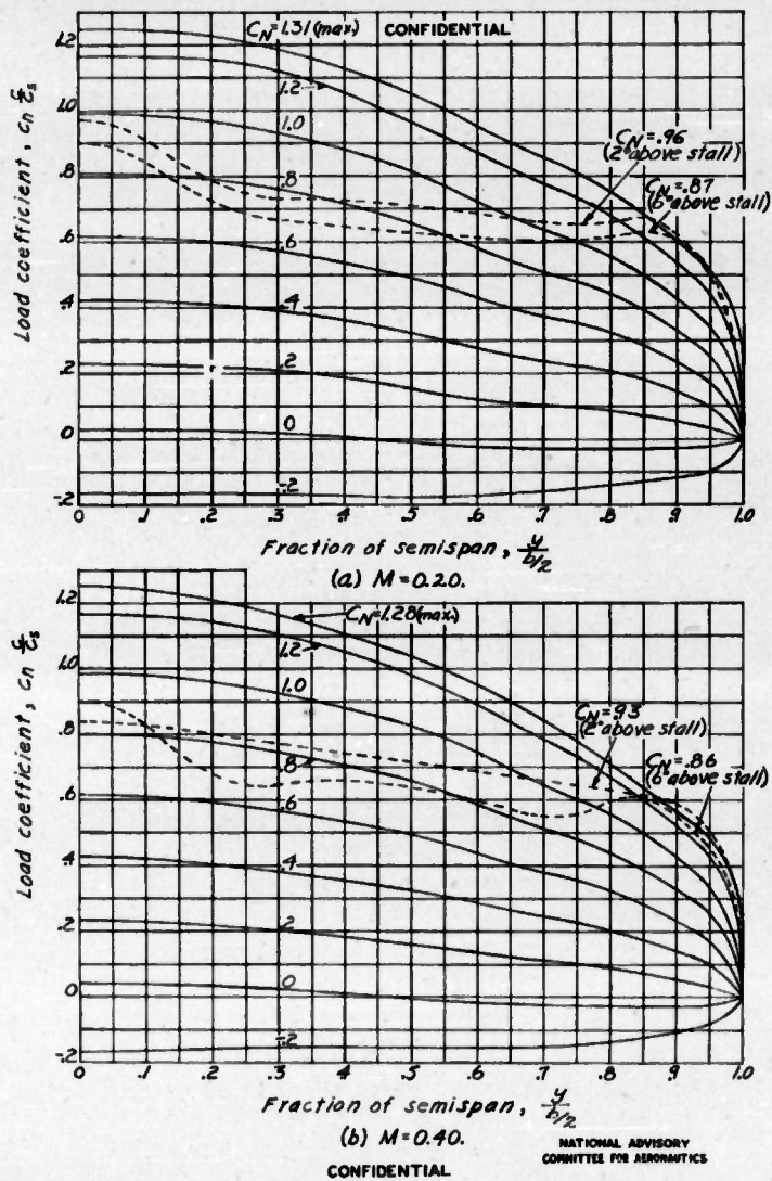
Figure 10. - Spanwise load distribution curves for several values of wing normal-force coefficient and Mach number.
