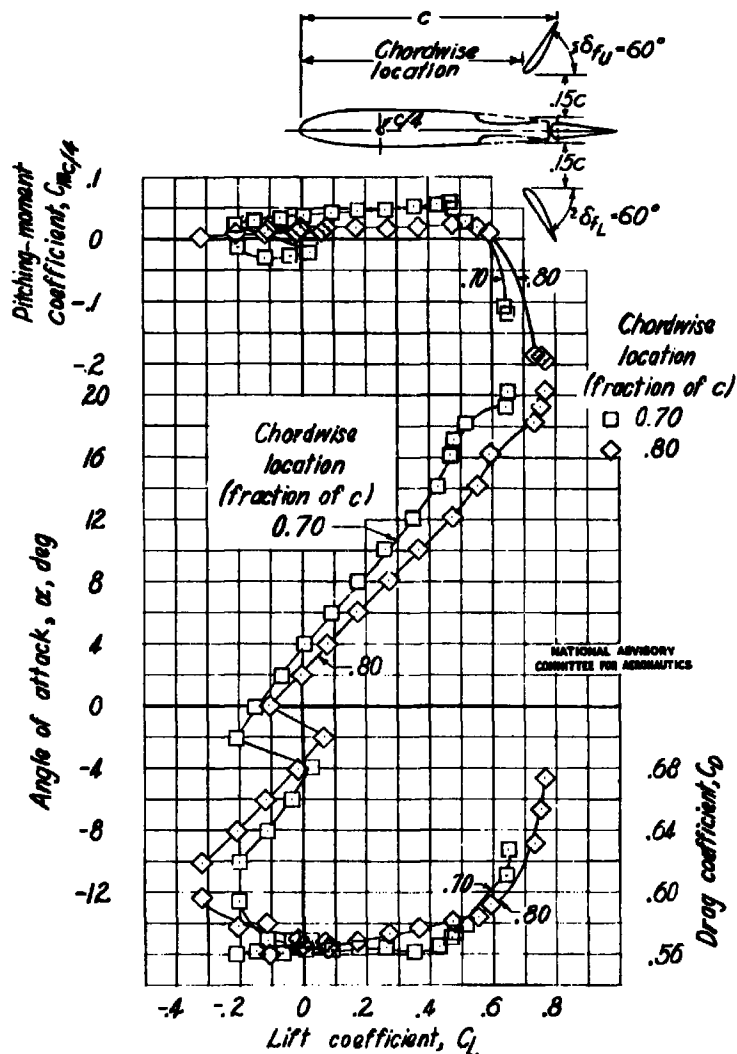
Figure 29—Lift, drag, and pitching-moment characteristics of the NACA 2212 wing model equipped with balanced double split flaps having Clark Y sections. Gaps, 0.15c ; \delta a, 0^\circ ; \delta f_U and \delta f_L, 60^\circ .
