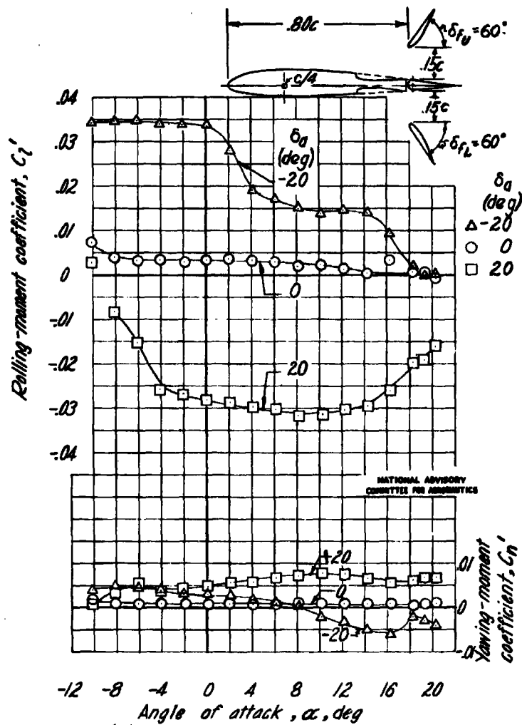
(b) Chordwise location, 0.80c . Figure 30.- Concluded.
