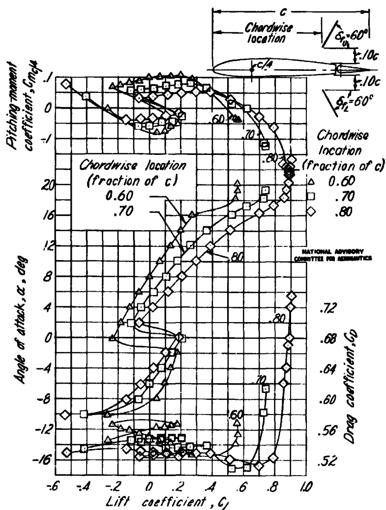
Figure 13.-Lift, drag, and pitching-moment characteristics of the NACA 2212 wing model equipped with balanced double split flaps having flat-plate sections. Gaps, 0.10c ; \delta_{1/2} , 0^\circ ; \delta_{1/2} and \delta_{1/2} , 60^\circ .
