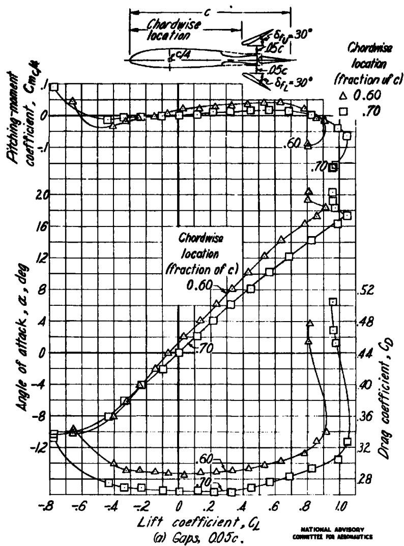
Figure 23- Lift, drag, and pitching-moment characteristics of the NACA 2212 wing model equipped with balanced double split flaps having Clark Y sections. \delta_0 , 0^\circ ; \delta_{f1} and \delta_{f2} , 30^\circ .
