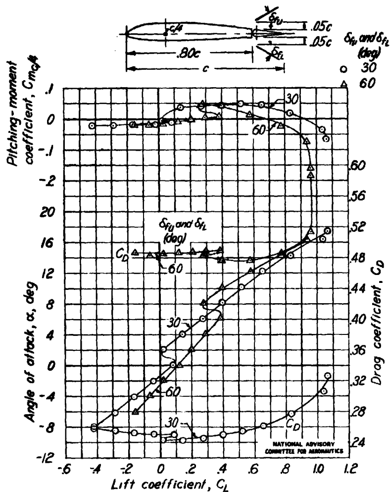
Figure 9.—Lift, drag, and pitching-moment characteristics of the NACA 2212 wing model equipped with balanced double split flaps having flat-plate sections. Chordwise location, 0.80c ; gaps, 0.05c ; \delta_a, 0^\circ .
