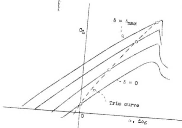
Figure 10.- Simultaneous change in lift and angle of attack produced by a flap on a wing with sweepback.
