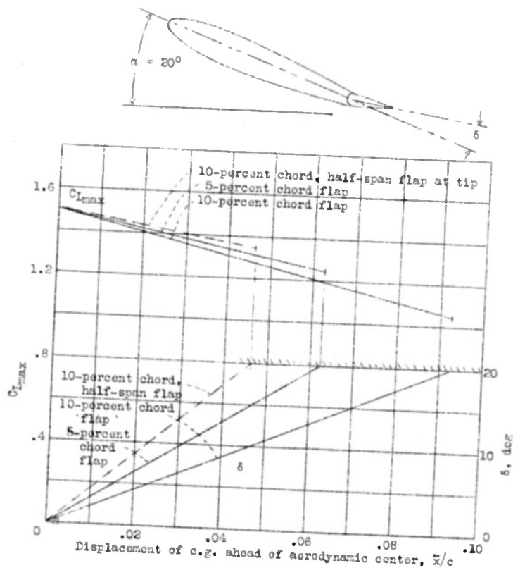
Figure 7.- Elevator deflections and corresponding reductions in C_{Lmax} for trim at \alpha = 20^\circ . Rectangular wing, aspect ratio, 6.
