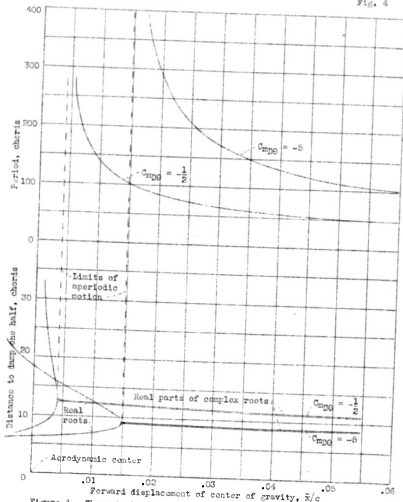
Figure 4.- Characteristics of the short-period longitudinal oscillation.
