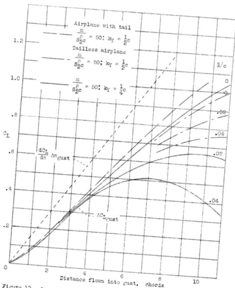
Figure 12.- Gust-alleviating action due to pitching motion and to lag in the development of lift.
