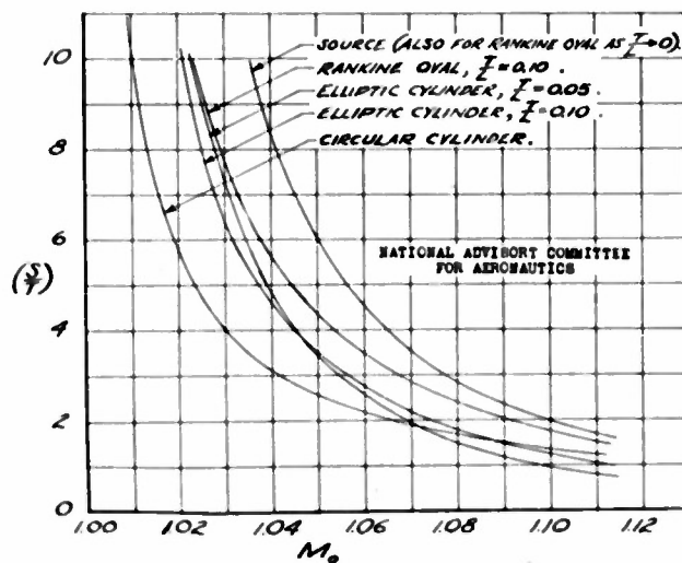
FIGURE 4.—LOCATION OF SHOCK WAVE IN FRONT OF TWO-DIMENSIONAL BODIES.
