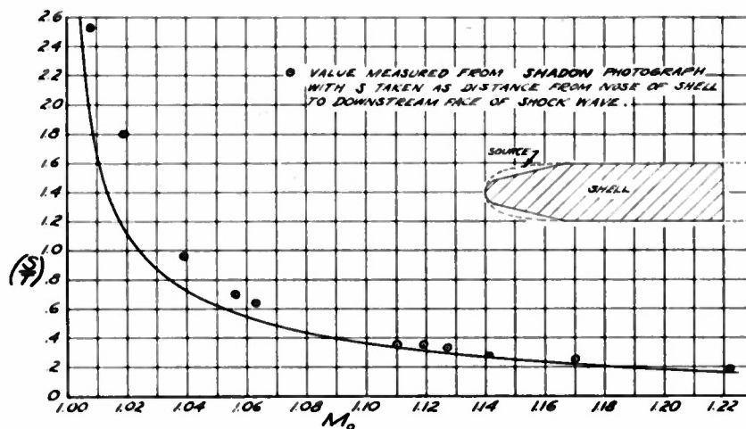
FIGURE 3.—COMPARISON OF MEASURED LOCATION OF SHOCK WAVE IN FRONT OF A 20 MM SHELL WITH THEORETICAL LOCATION FOR A THREE-DIMENSIONAL SOURCE.
