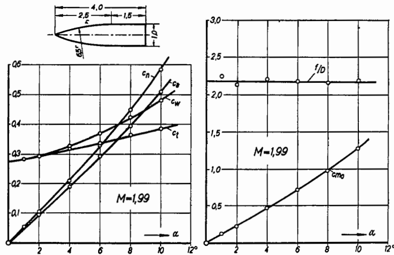
Figure 3. Example of missile test results measured in wind tunnel at M = 1.99 .
