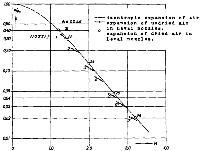
Figure 1. Expansion of dried and undried atmospheric air in Laval nozzles against the isentropic curve.
