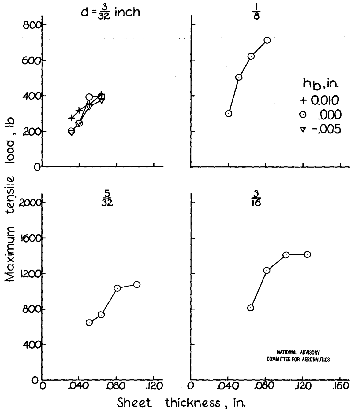
Figure 8. - Variation of maximum tensile load with sheet thickness for conventional machine-countersunk flush rivets; rivet-head angle = 78^\circ .
