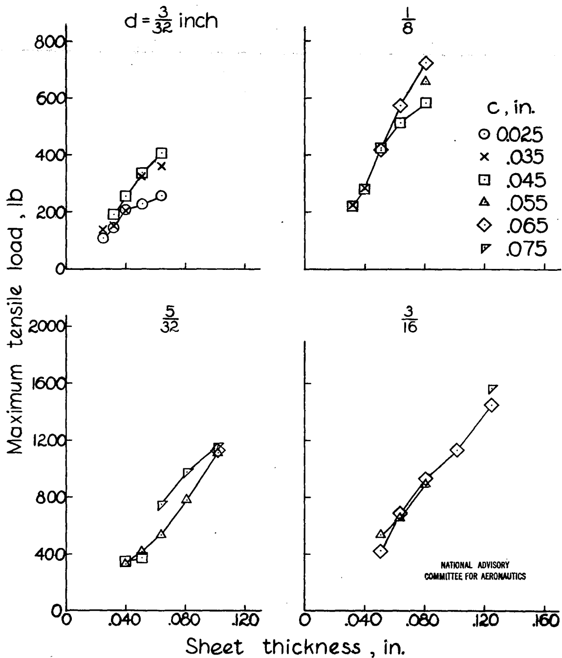
Figure 5. - Variation of maximum tensile load with sheet thickness for NACA machine-countersunk flush rivets ; rivet-head angle = 60^\circ .
