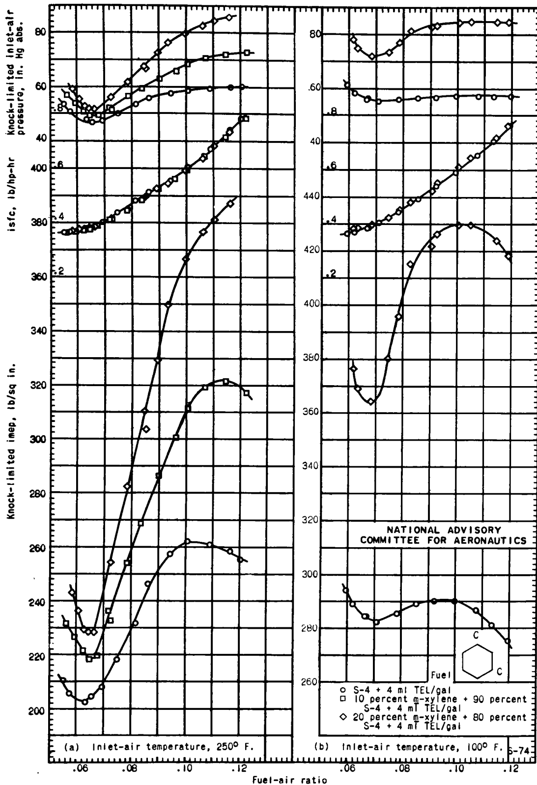
Figure 18. - The knock-limited performance of leaded blends of m -xylene and S-4 reference fuel in a 17.6 engine. Compression ratio, 7.0; engine speed, 1800 rpm; spark advance, 30° B.T.C.; outlet-coolant temperature, 212° F.
