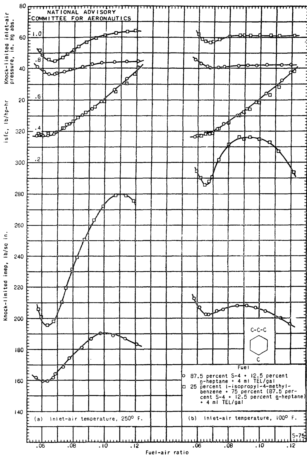
Figure 22. - The knock-limited performance of leaded blends of 1-isopropyl-4-methylbenzene and a base fuel consisting of 87.5 percent S-4 plus 12.5 percent n-heptane in a 17.6 engine. Compression ratio, 7.0; engine speed, 1800 rpm; spark advance, 30° B.T.C.; outlet-coolant temperature, 212° F.
