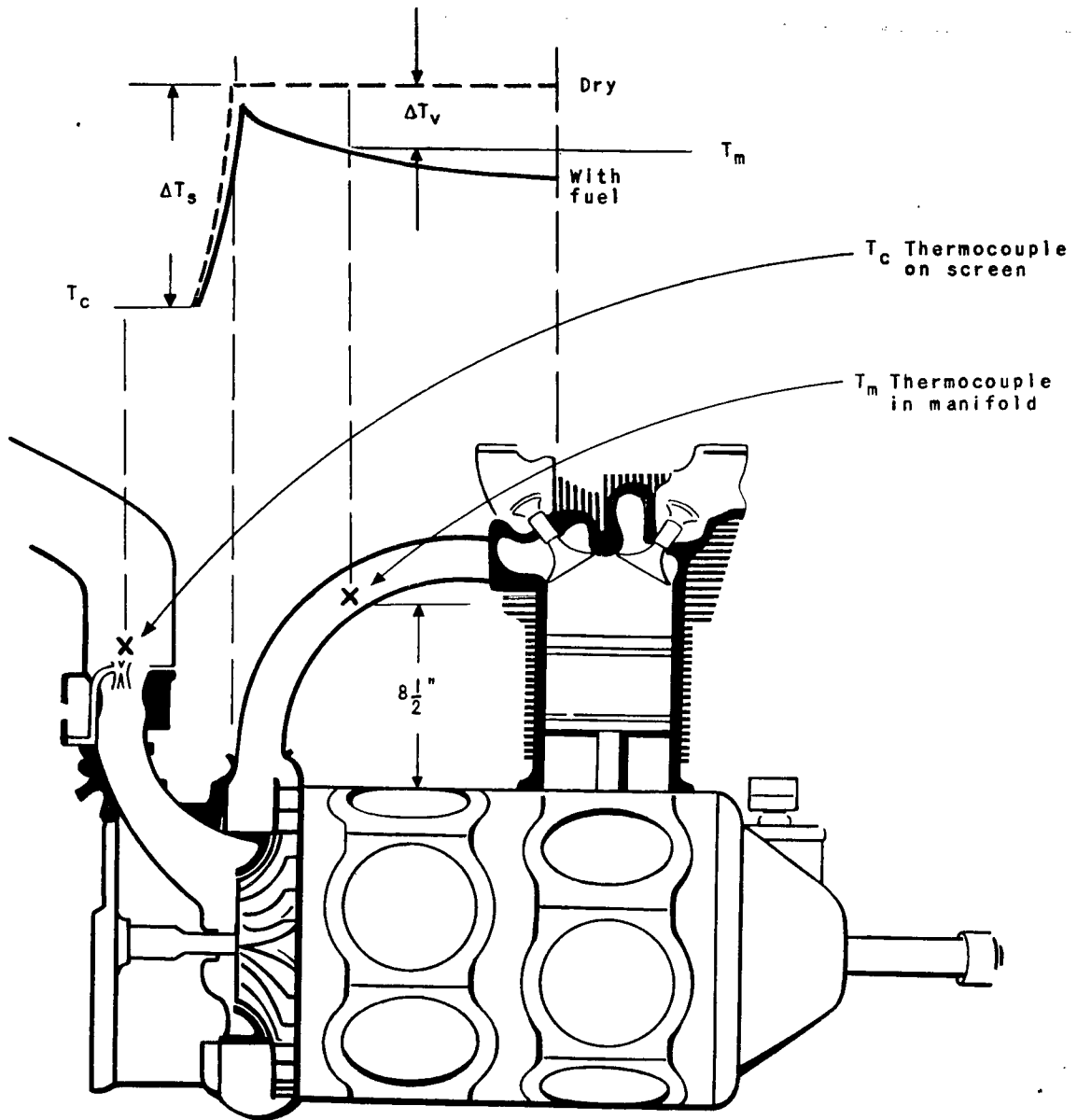
Figure 3. - Schematic section of a typical radial-engine induction system.
