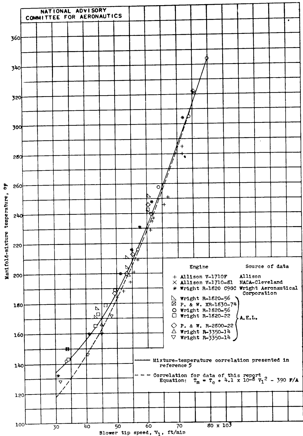
Figure 7. - Correlation of mixture-temperature data from outside sources. Carburetor-air temperature, 100^\circ\text{F} ; fuel-air ratio, 0.05. Plot obtained from plate 4 of reference 5.
