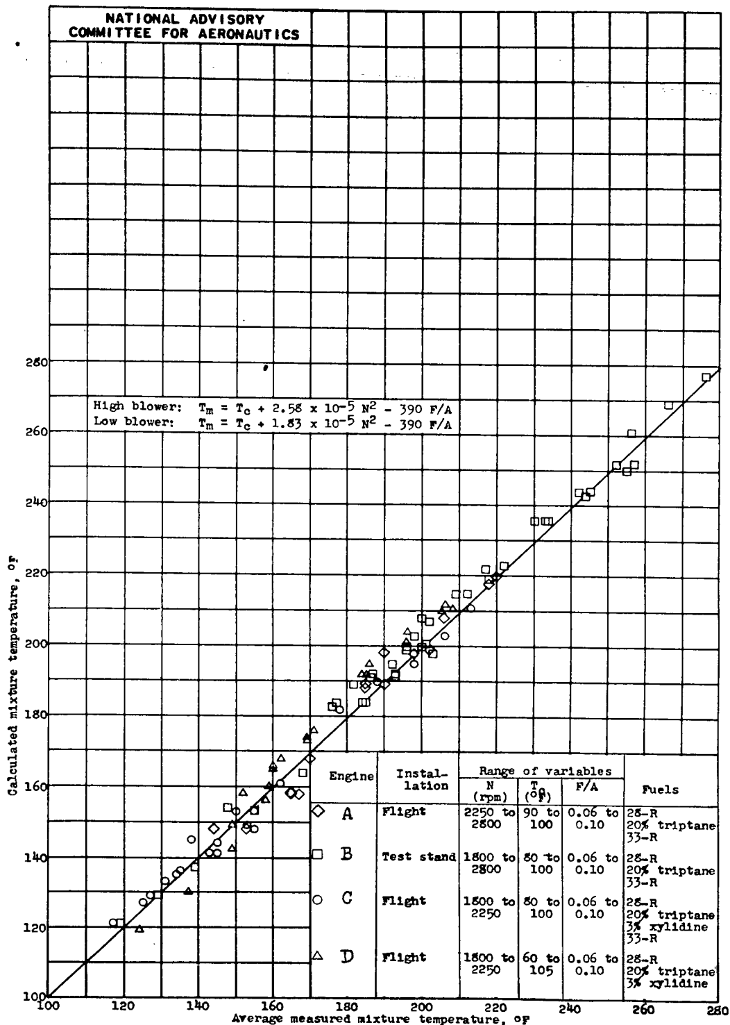
Figure 6. - Relation between calculated and average measured mixture temperature for double-row radial air-cooled engines in flight and test-stand operation.
