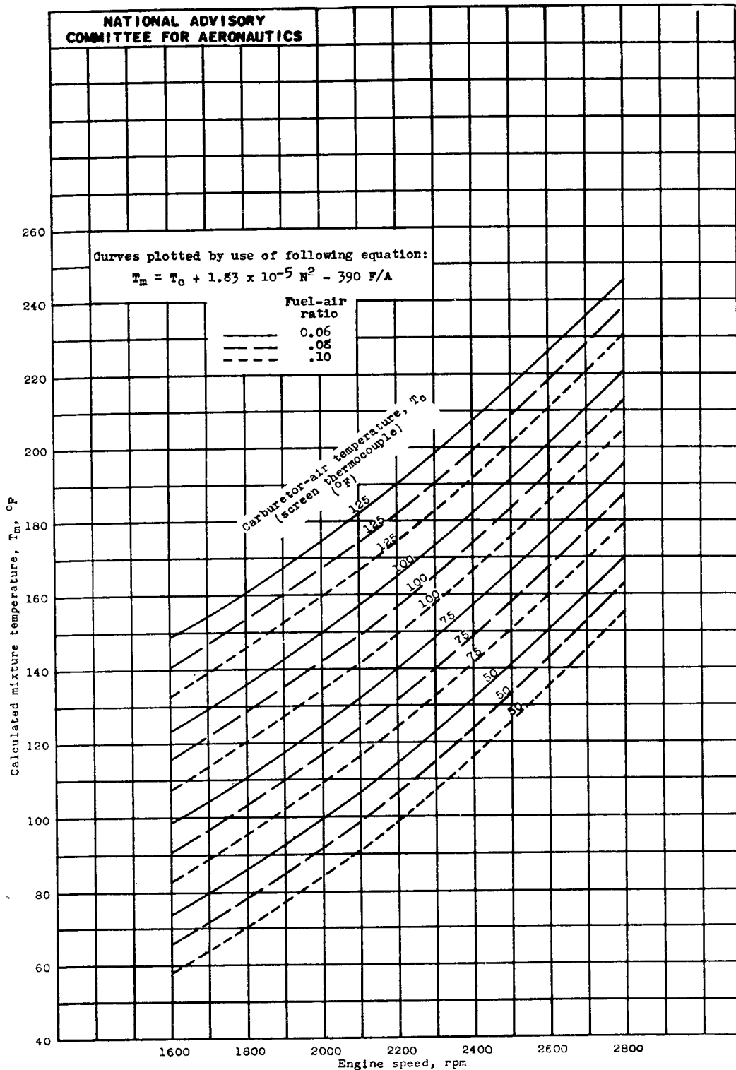
Figure 4. - Calculated relation between engine speed, carburetor-air temperature, fuel-air ratio, and mixture temperature. Impeller diameter, 11.3 inches.
