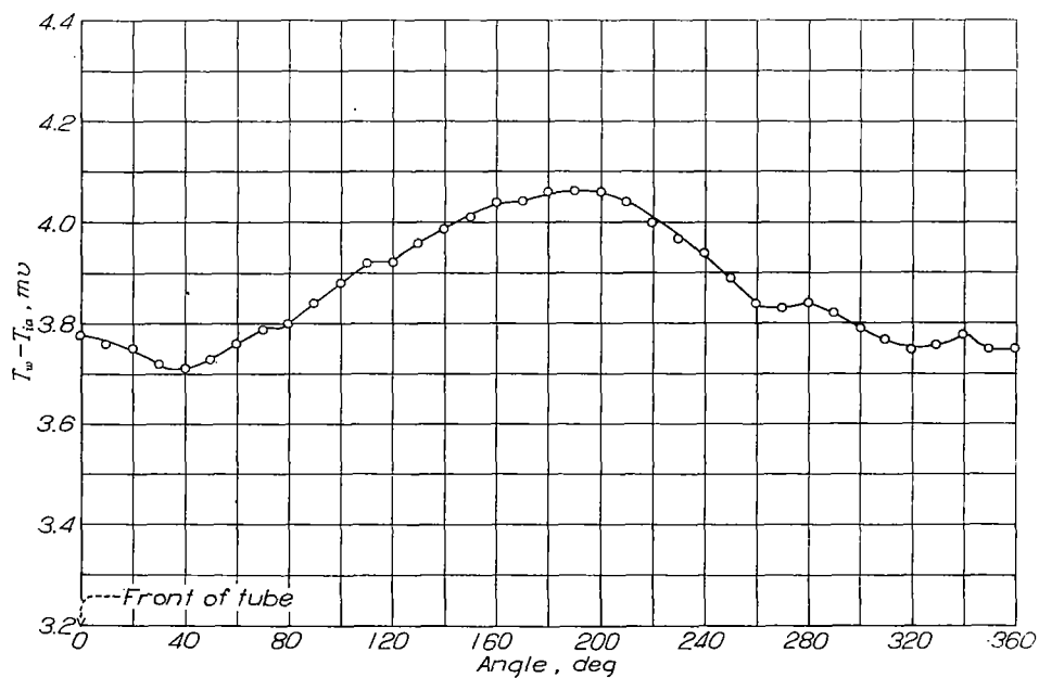
Figure 14.- Thermocouple survey of the surface of a heated brass circular tube in a bank at \rho V D_t / \mu = 42,300 . (T_w - T_a)_{\text{average}} = 128.4^\circ \text{F} , T_{ia} = 68.0^\circ \text{F} .
