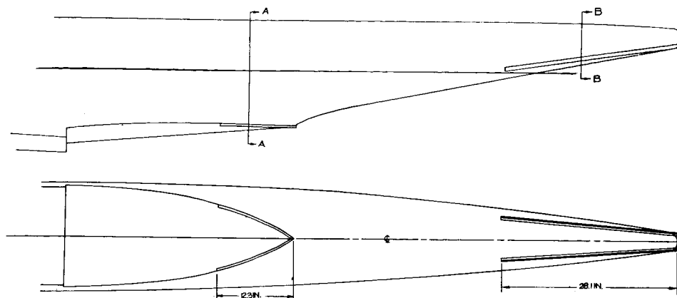
MODEL 183 A-1
