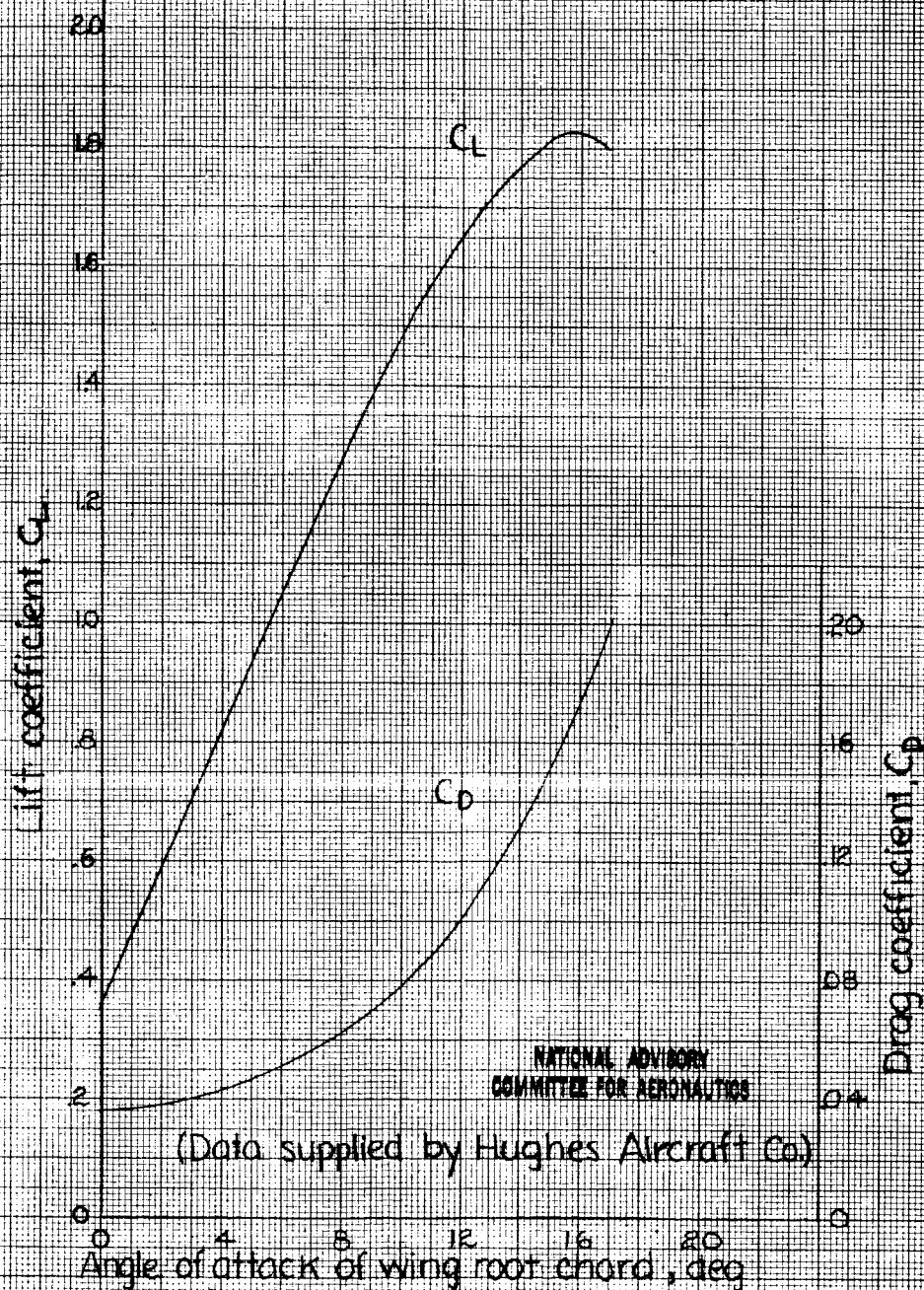
Figure 13.- Lift and drag coefficients for take-off calculations. Power-off, corrected for ground effect. \delta \leq 20^\circ , W, 5^\circ
