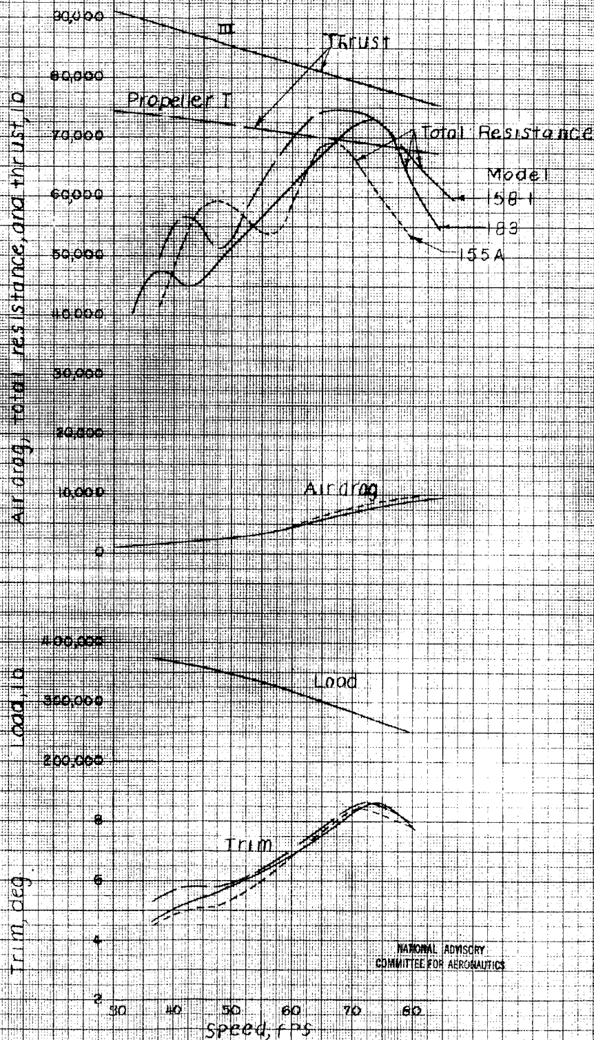
Figure 20- Comparison of take-off performance at hump speeds three models of the Hughes-Kaiser flying boat.
