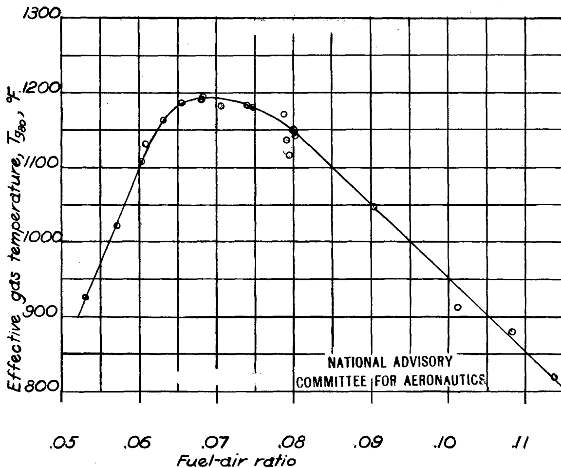
Figure 18. -Variation of mean effective gas temperature with fuel-air ratio, Cylinder heads.
