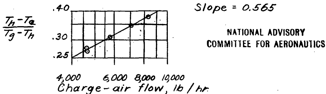
Figure 16. - Variation of (T_h - T_a)/(T_g - T_h) with charge-air flow. Fuel-air ratio, 0.08; \sigma_a \Delta p , 14.2 inches of water. Cylinder heads.
