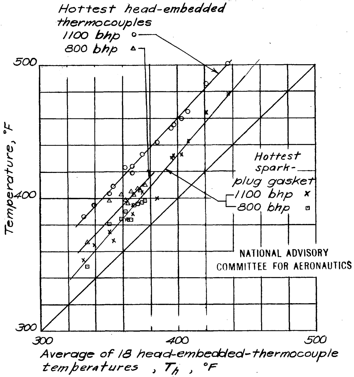
Figure 21. - A comparison of hottest with average head temperatures.
