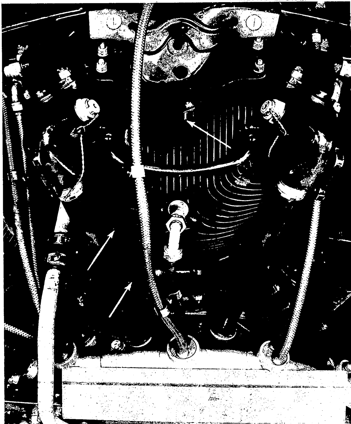
Figure 7.- Pressure-tube locations on front of front cylinders.
