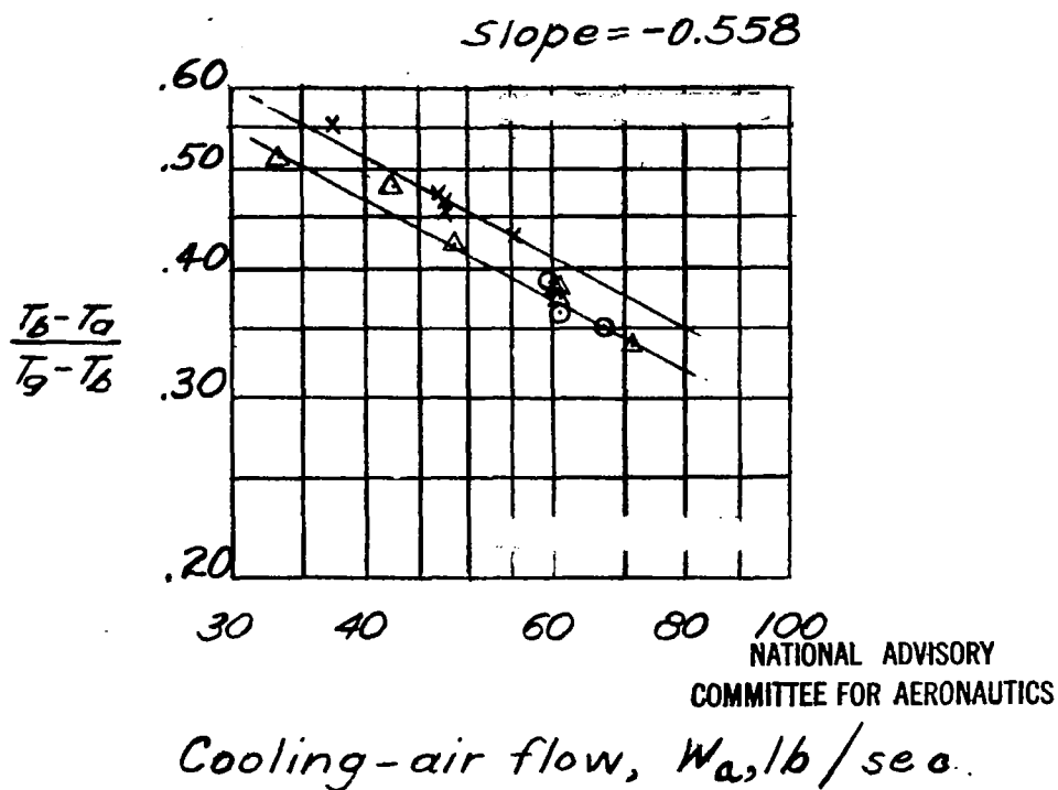
Figure 26.-Variation of (T_b - T_a)/(T_g - T_b) with cooling-air flow. Cylinder bases.
