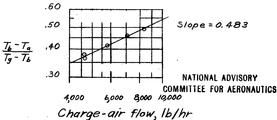
Figure 23.- Variation of (T_b - T_a)/(T_g - T_b) with charge-air flow. Fuel-air ratio, 0.08; \sigma_a \Delta p , 10.5 inches of water. Cylinder bases.
