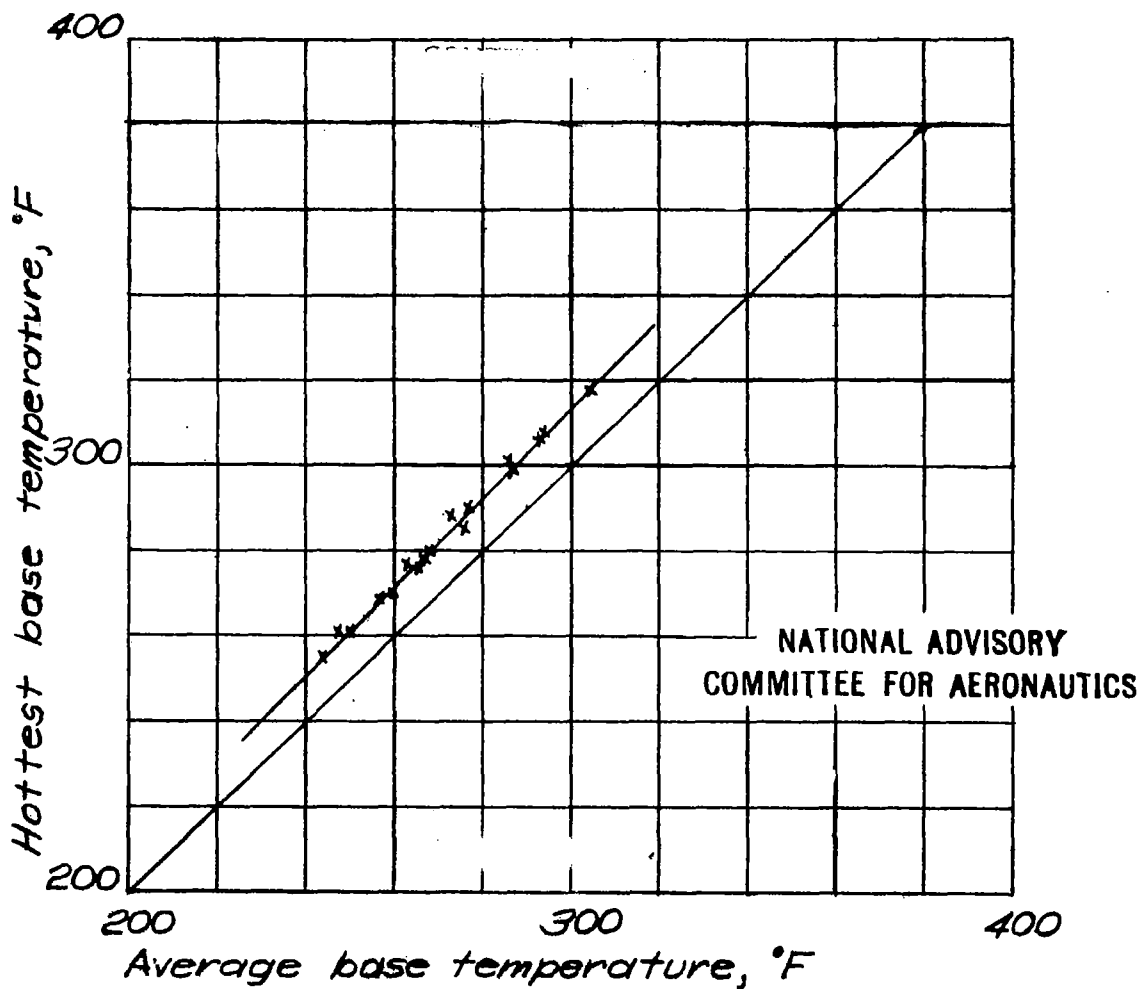
Figure 28.—Comparison of the hottest base temperature with average base temperature.
