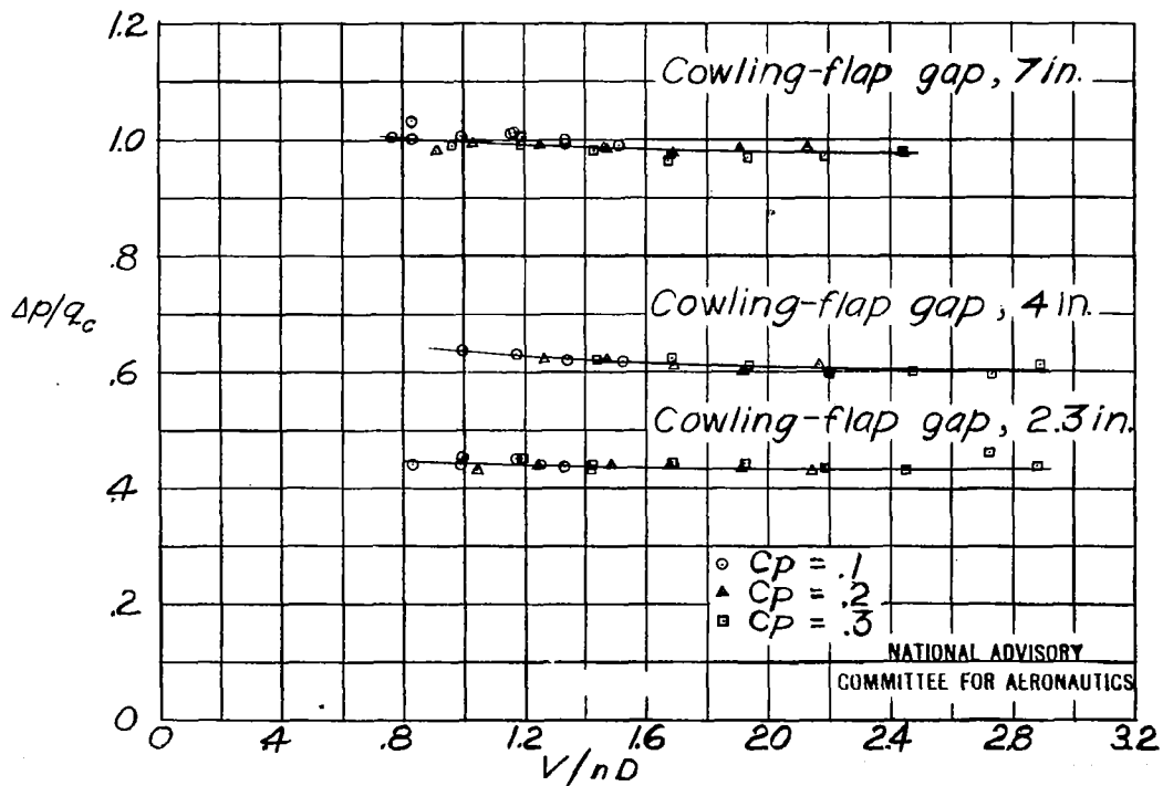
Figure 13.- Variation of available pressure drop across the cylinder barrels with propeller-advance ratio.
