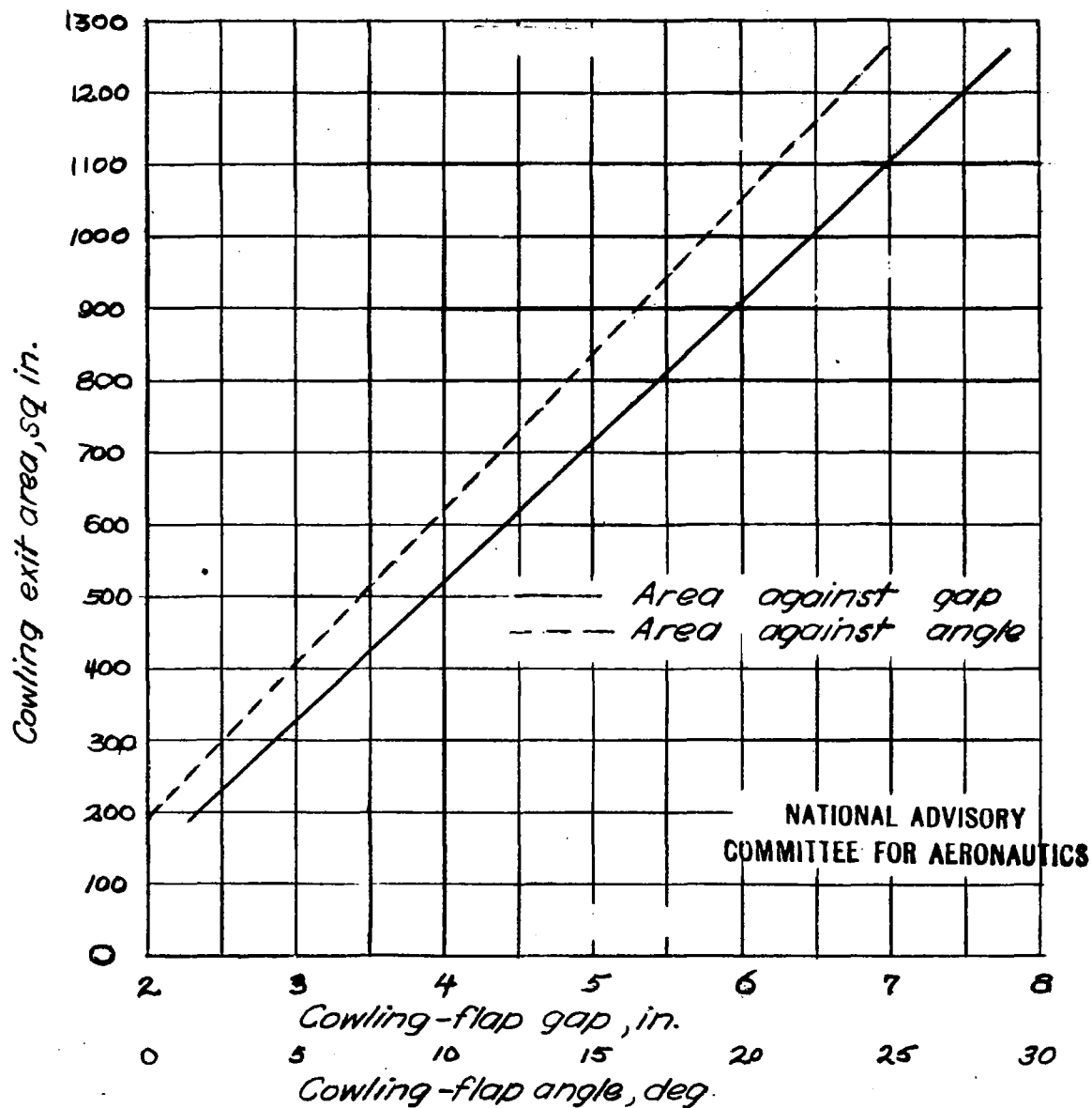
Figure 3. - Cowling - exit - area calibration.
