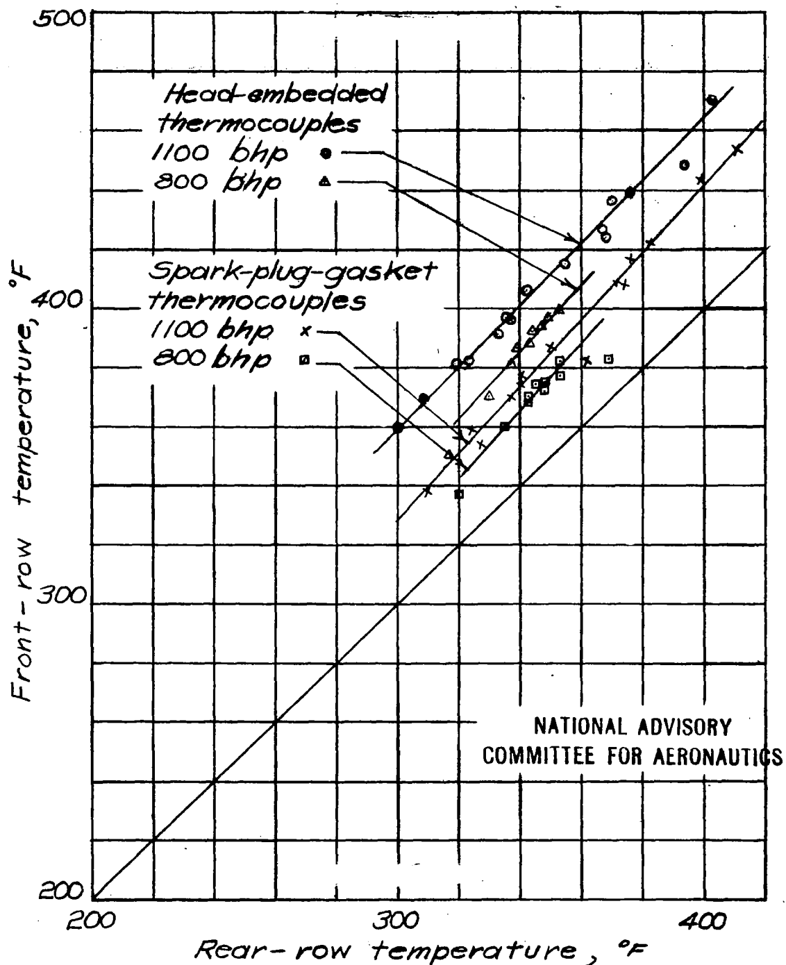
Figure 30.— Comparison of average temperature of front cylinders with average of rear cylinders, Fuel-air ratio, 0.08.
