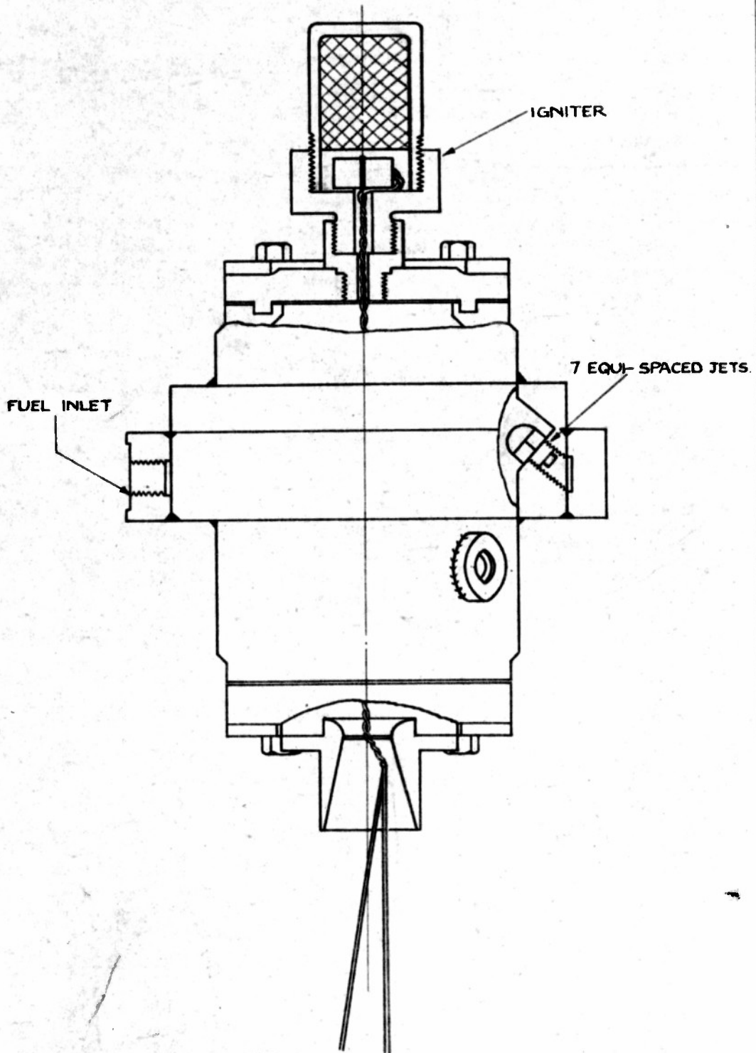
CONTRAFLOW INJECTOR AND COMBUSTION CHAMBER
