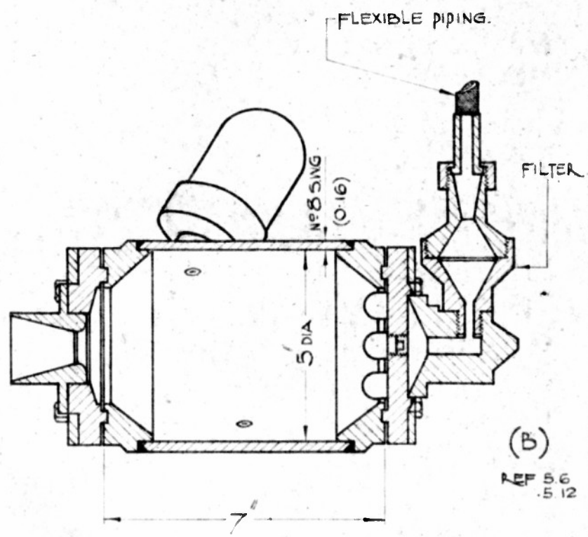
LATER (USED) TYPE COMBUSTION CHAMBER—FABRICATED.
