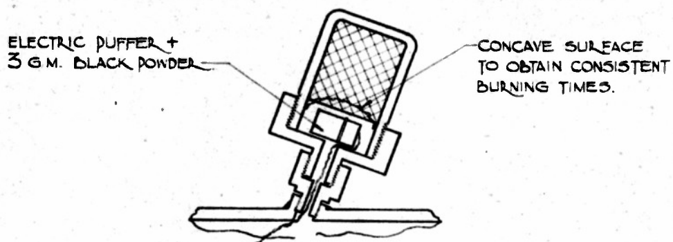
CIGARETTE BURNING PLASTIC PROPELLANT FILLED IGNITER.
