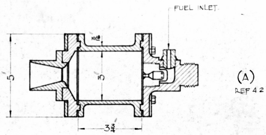
EARLY TYPE COMBUSTION CHAMBER (TURNED FROM SOLID.)
