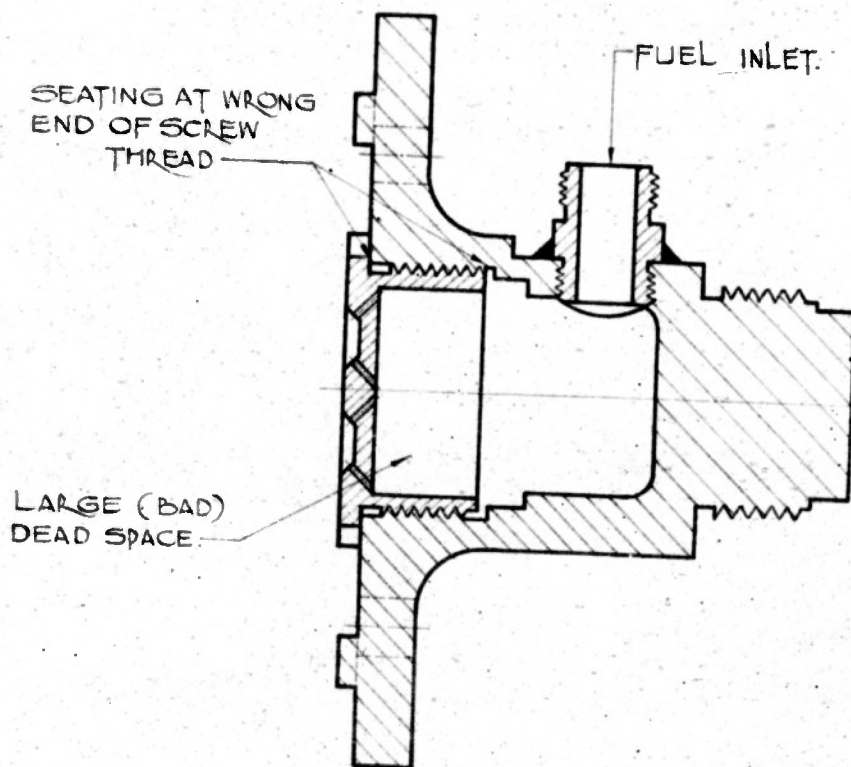
IMPINGING JET SPRAY INJECTOR - FIRST TYPE.
