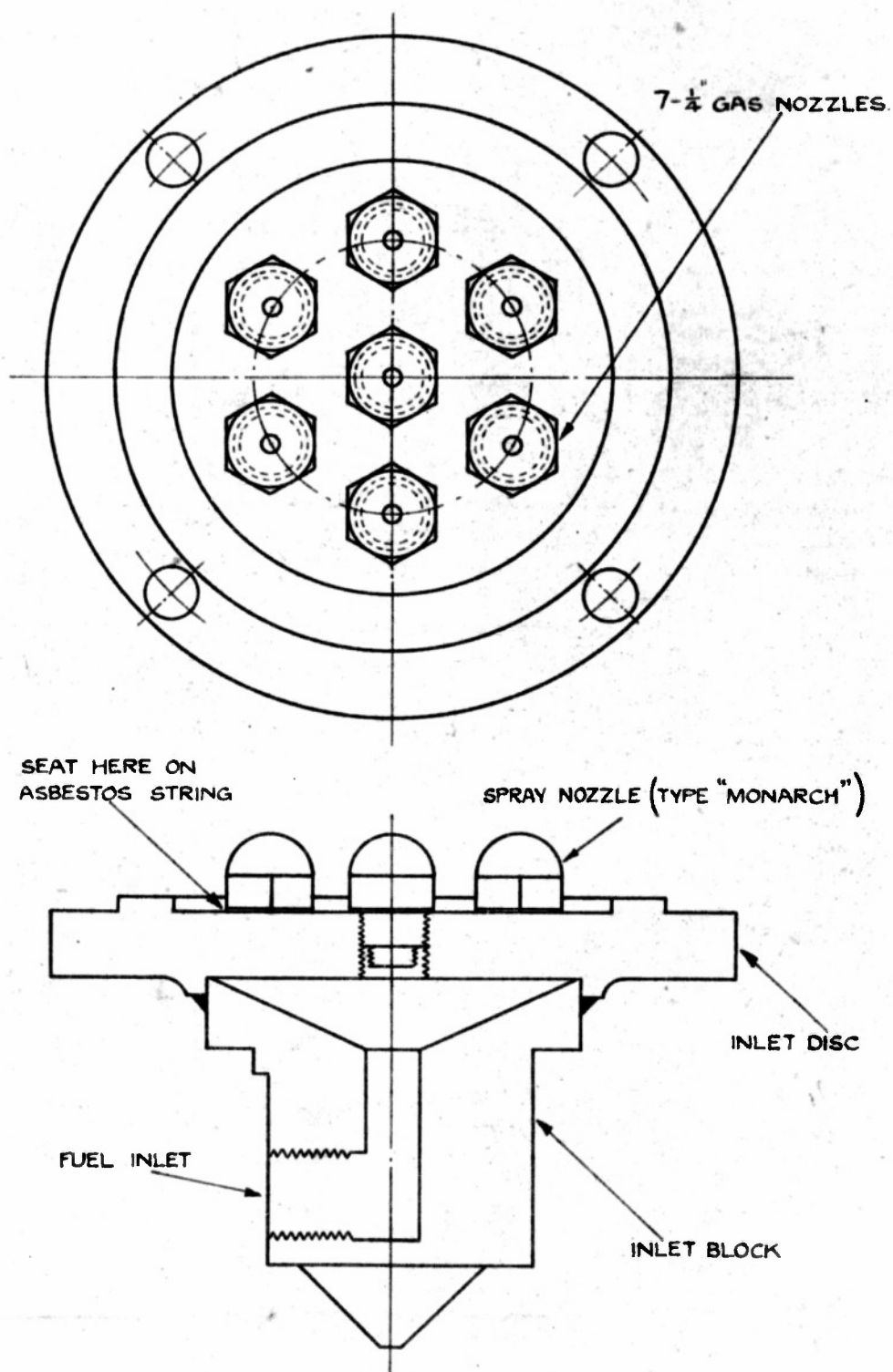
MULTIPLE SWIRL SPRAY INJECTOR
