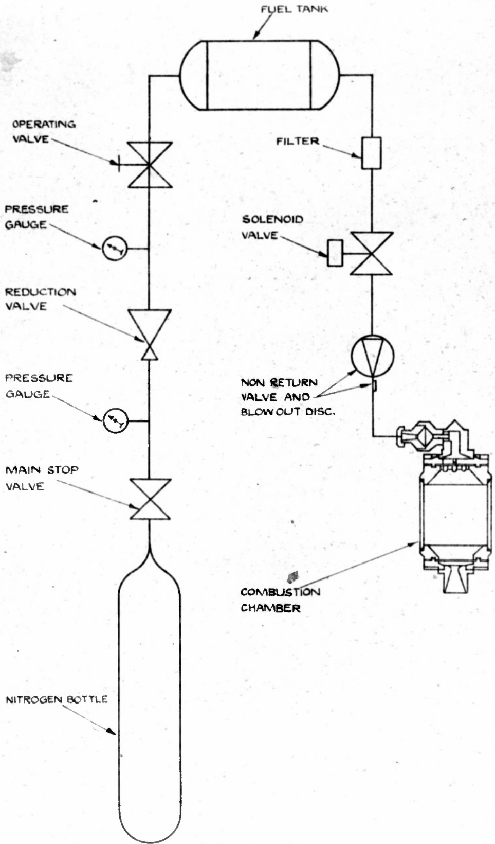
FLOW DIAGRAM
