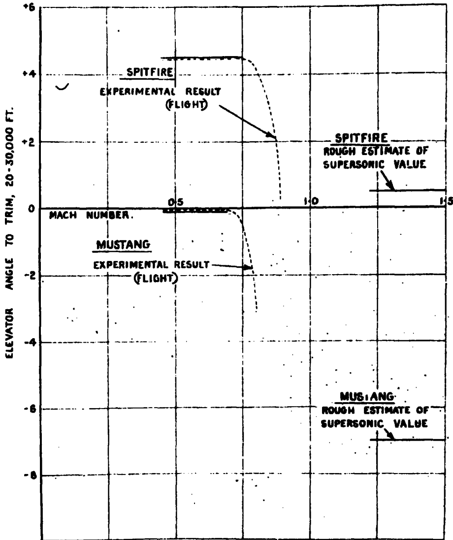
CHANGE OF ELEVATOR ANGLE TO TRIM AT HIGH MACH NUMBERS FLIGHT RESULTS COMPARED WITH ESTIMATED SUPERSONIC VALUE.
