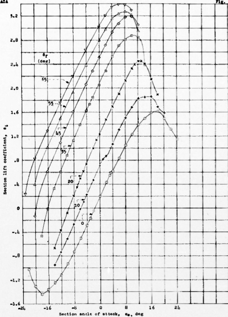
Figure 3.- Section lift characteristics of an NACA 65,3-118, a = 1.0 airfoil with a 0.5090 double-slotted flap at various deflections; R , 6,000,000 (approximately). Tests, M 399, 435, 452.
