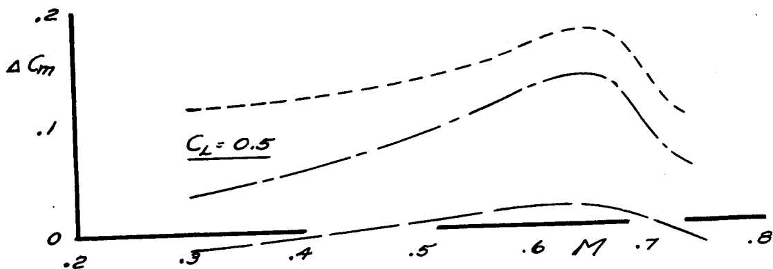
FIGURE 25. - ADDITIONAL PITCHING-MOMENT COEFFICIENT FROM VARIOUS DEFLECTIONS OF THE INBOARD AUXILIARY CONTROL FLAPS AT 30-PERCENT WING CHORD ON THE HIGHLY CAMBERED 66-SERIES WING.
