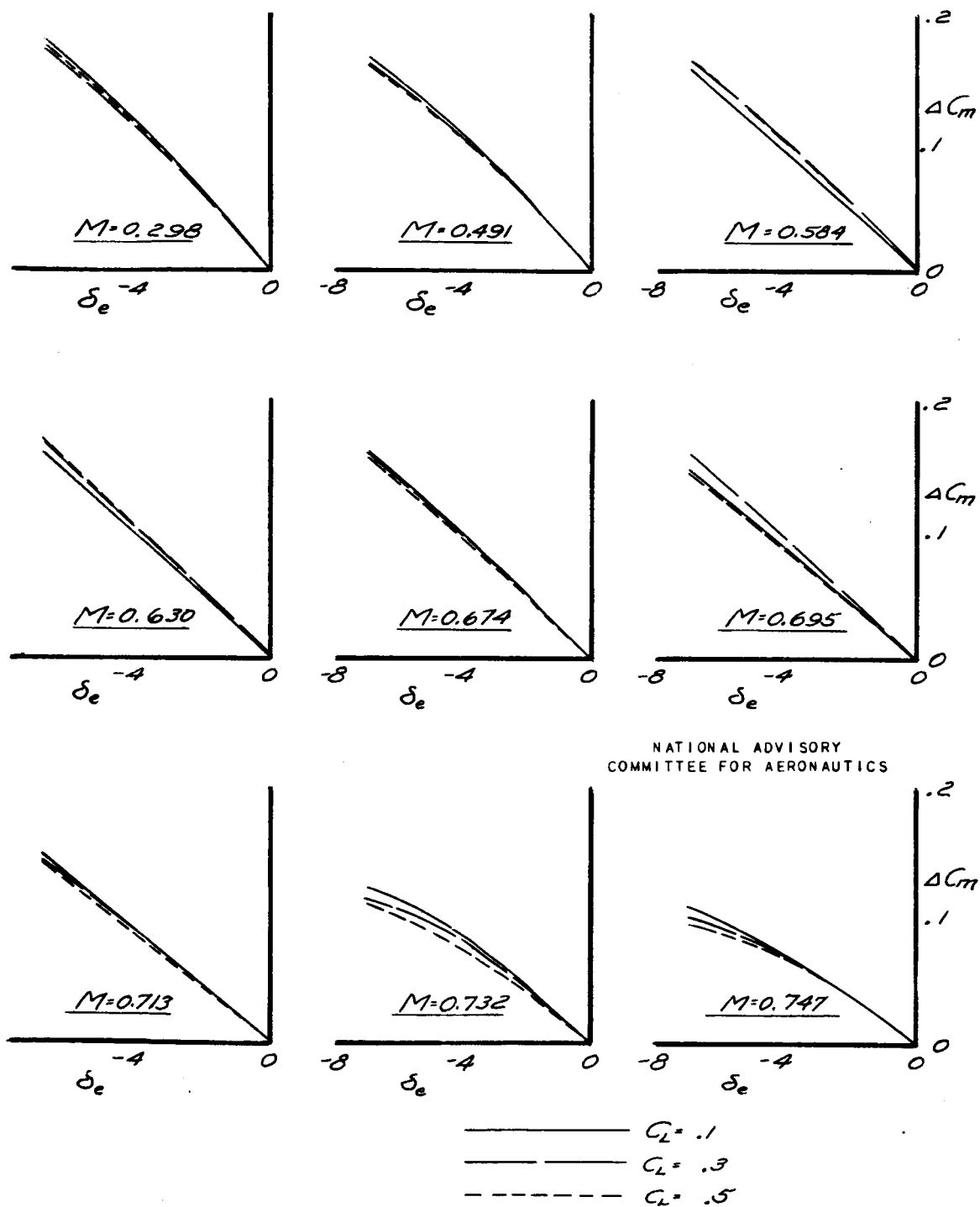
FIGURE 28.- ADDITIONAL PITCHING-MOMENT COEFFICIENT FROM DEFLECTION OF THE ELEVATOR. MODEL WITH THE HIGHLY CAMBERED 66-SERIES WING.
