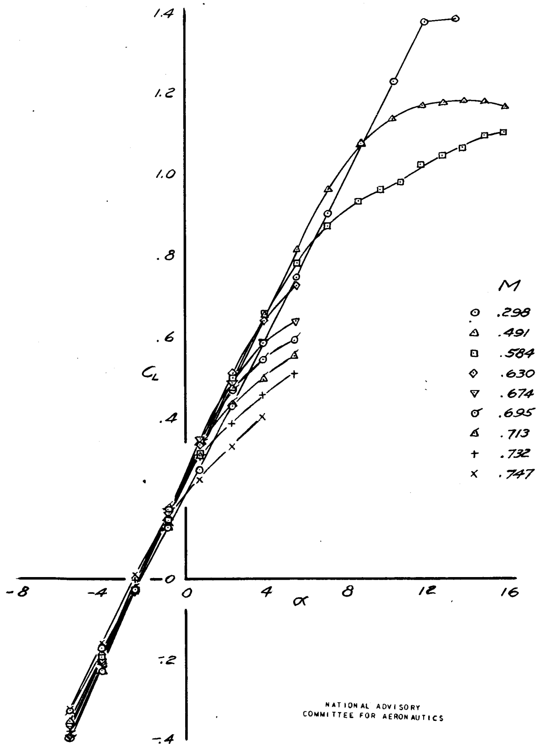
FIGURE 4.6 - LIFT CHARACTERISTICS OF THE MODEL WITH THE NACA 230-SERIES WING.
