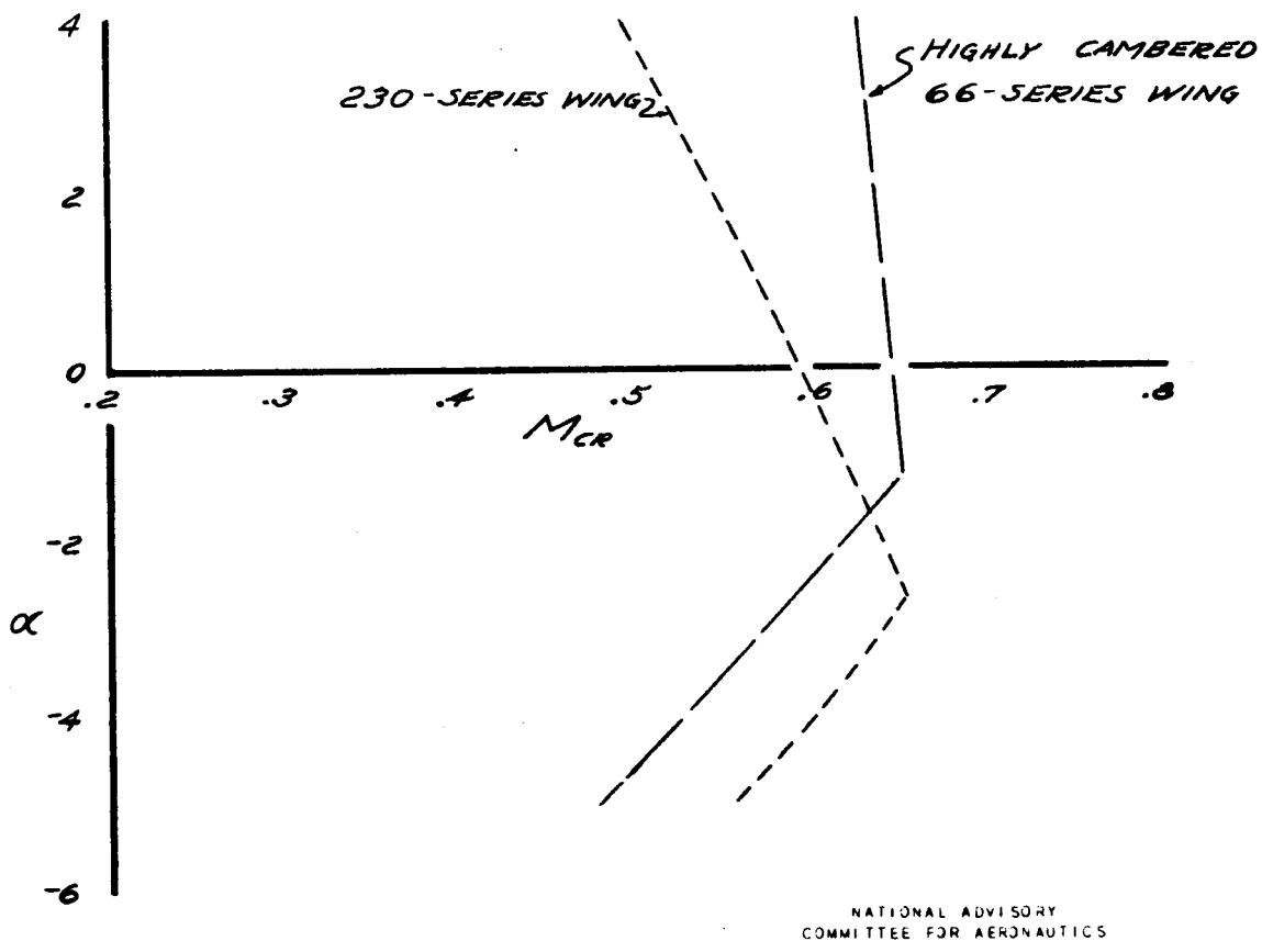
FIGURE 9.- CRITICAL MACH NUMBER OF THE 230-SERIES WING AND THE HIGHLY CAMBERED 66-SERIES WING.
