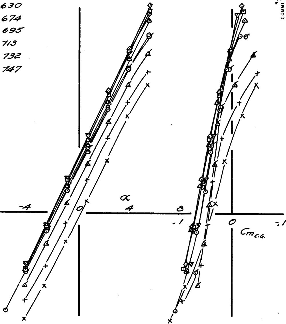
FIGURE 5B LIFT, DRAG, AND PITCHING-MOMENT CHARACTERISTICS OF THE MODEL WITH THE HIGHLY CAMBERED NACA 66-SERIES WING. STABILIZER ANGLE, 0^\circ .
