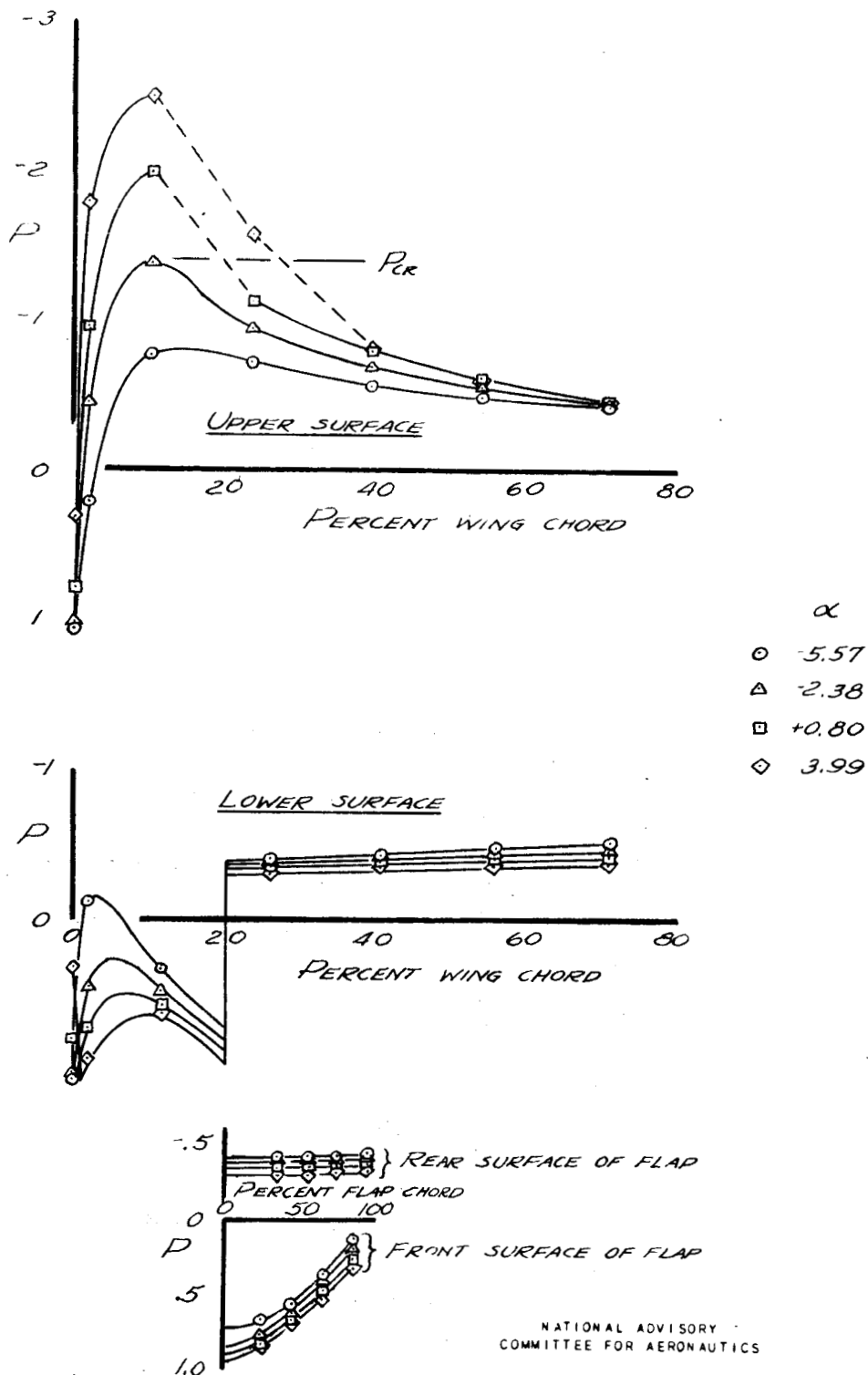
FIGURE 18(a).- WING AND FLAP PRESSURE DISTRIBUTION AT WING STATION 28.85 ON THE 230-SERIES WING WITH OUTBOARD 45° AUXILIARY CONTROL FLAPS AT 20-PERCENT WING CHORD. MACH NUMBER, 0.584.
