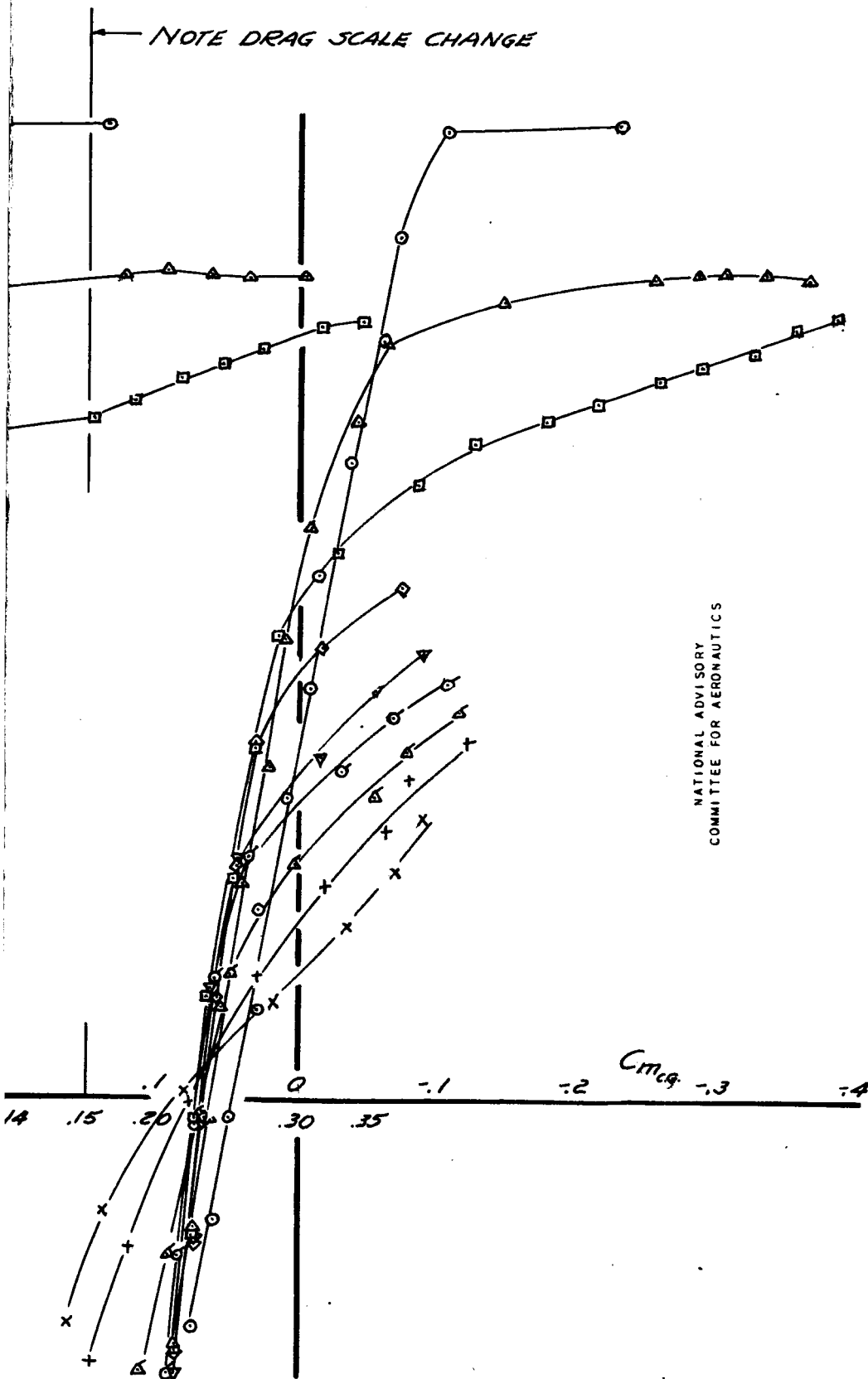
FIGURE 4B.- DRAG AND PITCHING-MOMENT CHARACTERISTICS OF THE MODEL WITH THE NACA 230-SERIES WING.
