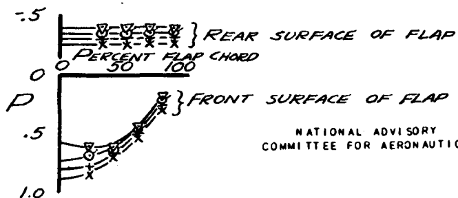
FIGURE 21 (a).- WING AND FLAP PRESSURE DISTRIBUTION AT WING STATION 28.6 ON THE HIGHLY CAMBERED 66-SERIES WING WITH OUTBOARD 45^\circ AUXILIARY CONTROL FLAPS AT 30-PERCENT WING CHORD. MACH NUMBER, 0.584.
