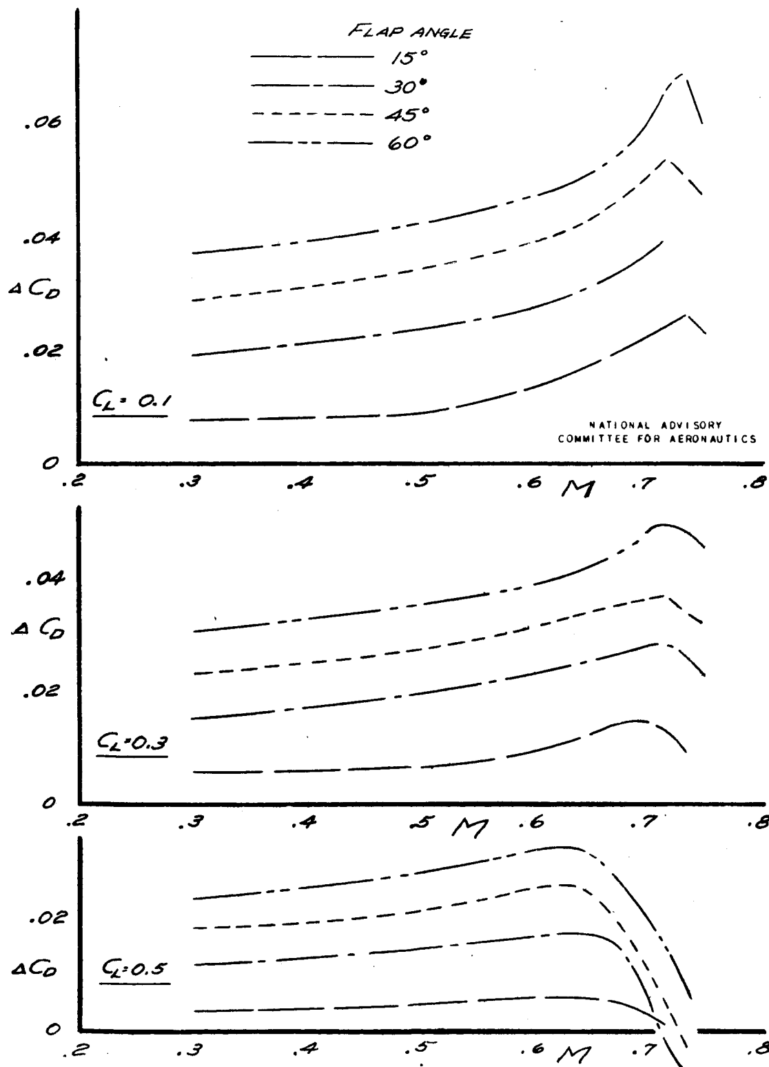
FIGURE 14. - ADDITIONAL DRAG COEFFICIENT FROM VARIOUS DEFLECTIONS OF THE OUTBOARD AUXILIARY CONTROL FLAPS AT 20-PERCENT WING CHORD ON THE 230-SERIES WING.
