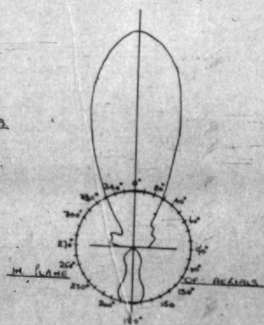
Fig. 2. TYPICAL POLAR DIAGRAMS.
