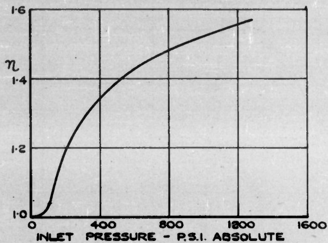
FIG. 8. VARIATION OF \eta WITH INLET PRESSURE.
