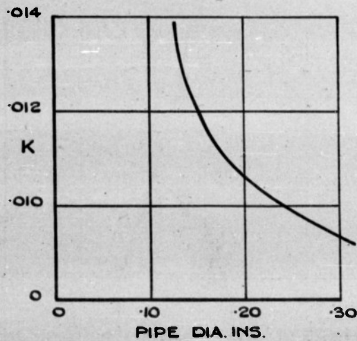
FIG. 9. VARIATION OF K WITH PIPE DIAMETER.
