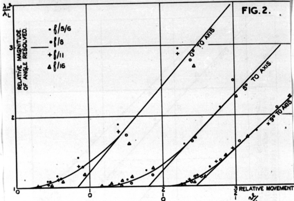
EFFECT OF MOVEMENT ON RESOLUTION.-TEST OBJECT. O/I DENSITY DIFFERENCE, MOVEMENT AT RIGHT ANGLES TO TEST LINES.
