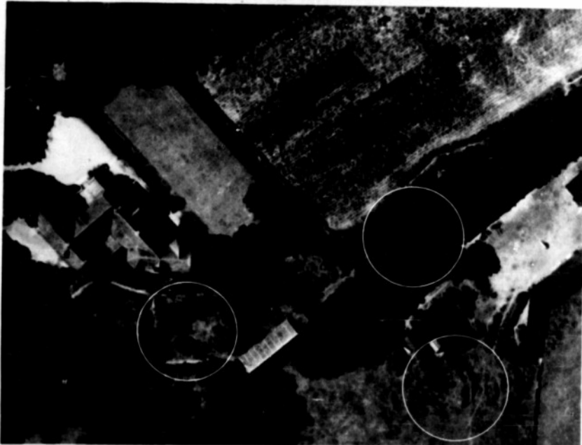
B. 5" PENTAC: f/8 : MINUS BLUE FILTER: 0.09 SEC. GYRO STABILISED F24 CAMERA MOVEMENT COMPENSATION: MAGNIFICATION 20X
