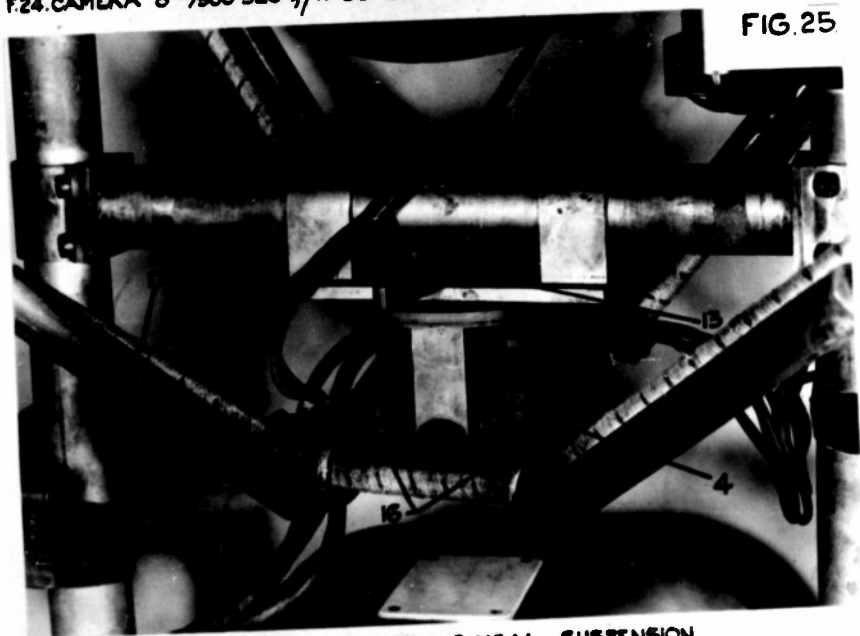
STABILISED CAMERA MOUNTING - GIMBAL SUSPENSION.
